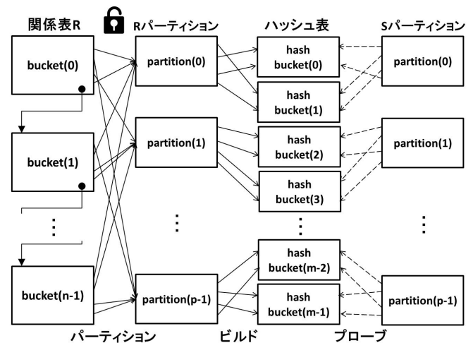
図2 shared-partitioning
