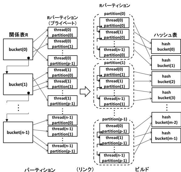
図 3 independent-partitioning
