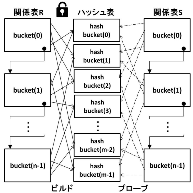
図1 no-partitioning
