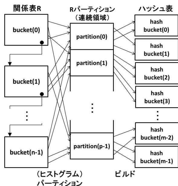
図 4 radix-partitioning
