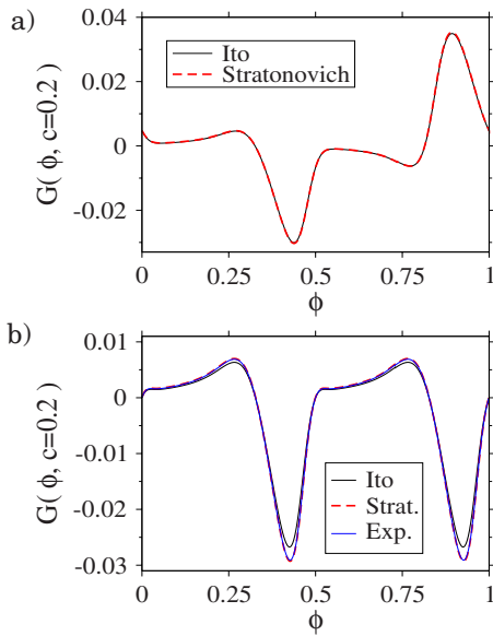
FIG. 3. (Color online) Comparison of Ito vs Stratonovich interpretations of Eq. (1) on the PRC G(\phi, c) of FHN for an impulse whose jump size is c=0.2 . (a) Additive impulse [\sigma(v, c)=c] and (b) linear multiplicative impulse [\sigma(v, c)=cv] . The curve ‘‘Ito’’ is calculated by affecting a discontinuous jump, i.e., impulse duration is 0. The curve ‘‘Stratonovich’’ and ‘‘Strat.’’ is calculated by continuously changing v using a narrow rectangular wave form of temporal width 0.0002. The curve ‘‘Exp.’’ is calculated using the Wang-Zakai-Marcus approximation for the continuous narrow impulse, namely, discontinuously changing the orbit by an amount g(v, c)=(e^c-1)v .
