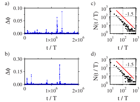
FIG. 9. (Color online) On-off intermittency exhibited by two oscillators in synchronized ( I_0=0.8 , additive impulses with c=0.1 ), and clustered ( I_0=0.875 , linear multiplicative impulses with c=0.1 ) states. Independent noise with D=9 \times 10^{-9} , and impulses with \lambda=1/4T were used. Phase difference \Delta\phi between the oscillators from stable configuration is small (laminar region) much of the time, but large occasional bursts occur. (a) Long-time evolution of \Delta\phi(t) , which shows excursions away from the synchronized state. (b) Distribution of laminar duration corresponding to (a) (arbitrary normalization). (c) Long-time evolution of \Delta\phi(t) from the 1/2 -out-of-phase clustered state, and (d) distribution of laminar duration corresponding to (c) (arbitrary normalization). Oscillators are considered to be in the laminar state when \Delta\phi < 0.0013 away from synchronized or clustered states. Laminar distributions exhibit power laws with exponent -1.5 . At this weak independent noise intensity, the phase difference between the oscillators takes only either 0 or 1/2 depending on the initial condition, and switching between the clustered state occurs is a very rare event.
