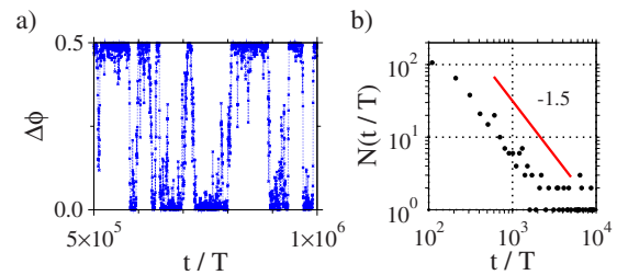
FIG. 10. (Color online) Transition between clustered states for two oscillators. \Delta\phi is the phase difference between the two oscillators. Poisson impulses with rate \lambda = 1/4T and c=0.1 was used. A larger independent noise with D=3 \times 10^{-4} is added in order to facilitate the transitions between single- and two-cluster states.
