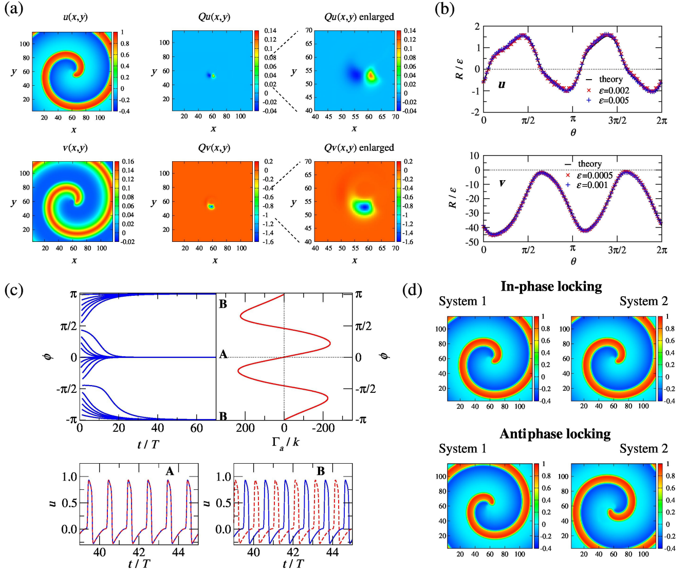
FIG. 4. Rotating spirals. The system is a 2D square of side L = 120 with no-flux boundary conditions. To pin the spiral at the center, a localized circular heterogeneity of radius r_0 = 4 is introduced to the parameter \alpha(x, y) as \alpha(x, y) = \alpha_0 + (\alpha_1 - \alpha_0) \exp(-r^4/r_0^4) , where r = [(x - L/2)^2 + (y - L/2)^2]^{1/2} is a distance from the center of the system. We assume \alpha_0 = 0.05 and \alpha_1 = 0.5 so that excitability is the highest at the center. Other parameters are fixed at \tau^{-1} = 0.005 , \gamma = 2.5 , \kappa = 0.15 , and \delta = 0 . With these parameters, the oscillation period of the spiral is T = 217.37 . (a) Spiral solution \mathbf{X}_0(x, y; \theta) = [u(x, y), v(x, y)] and the corresponding phase-sensitivity functions \mathbf{Q}(x, y; \theta) = [Q_u(x, y), Q_v(x, y)] at \theta = 0 . (b) Phase-response curves R(\theta) of the spiral normalized by the stimulus intensity \varepsilon . The checkerboard-like spatial perturbation is given either to the activator ( u ) or the inhibitor ( v ) component, where s(x, y) = \varepsilon for x, y > L/2 or x, y < L/2 , and s(x, y) = 0 otherwise. Results obtained by direct numerical simulations with two different values of \varepsilon are compared with the theory, R(\theta) = \langle \mathbf{Q}(x, y; \theta), \mathbf{s}(x, y) \rangle , where the inner product is taken over the 2D square ( 0 \leq x, y \leq L ). (c) Evolution of phase differences between two systems coupled through the u component with the coupling intensity matrix \mathbf{K} = \text{diag}(k = 2 \times 10^{-4}, 0) , compared with the antisymmetric part of the phase-reduction function \Gamma_a(\phi) (rescaled by the coupling intensity k ). Different blue lines show the evolution of \phi for different initial conditions. Both in-phase synchronization (A) and antiphase synchronization (B) can occur, depending on the initial conditions. The solid line corresponds to system 1, and the dashed line corresponds to system 2. (d) Snapshots of the in-phase and antiphase synchronized states.
