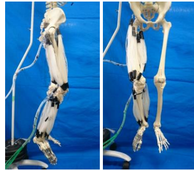
Fig. 4 A musculoskeletal robot mechanism with a very redundant drive mechanism having 50 independent muscles
