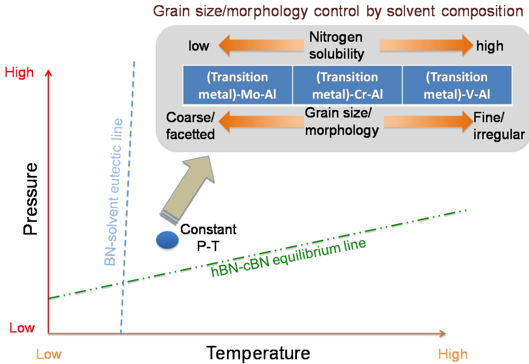
Fig. 1.9. Proposed method of grain size and morphology control in cubic BN synthesis process
