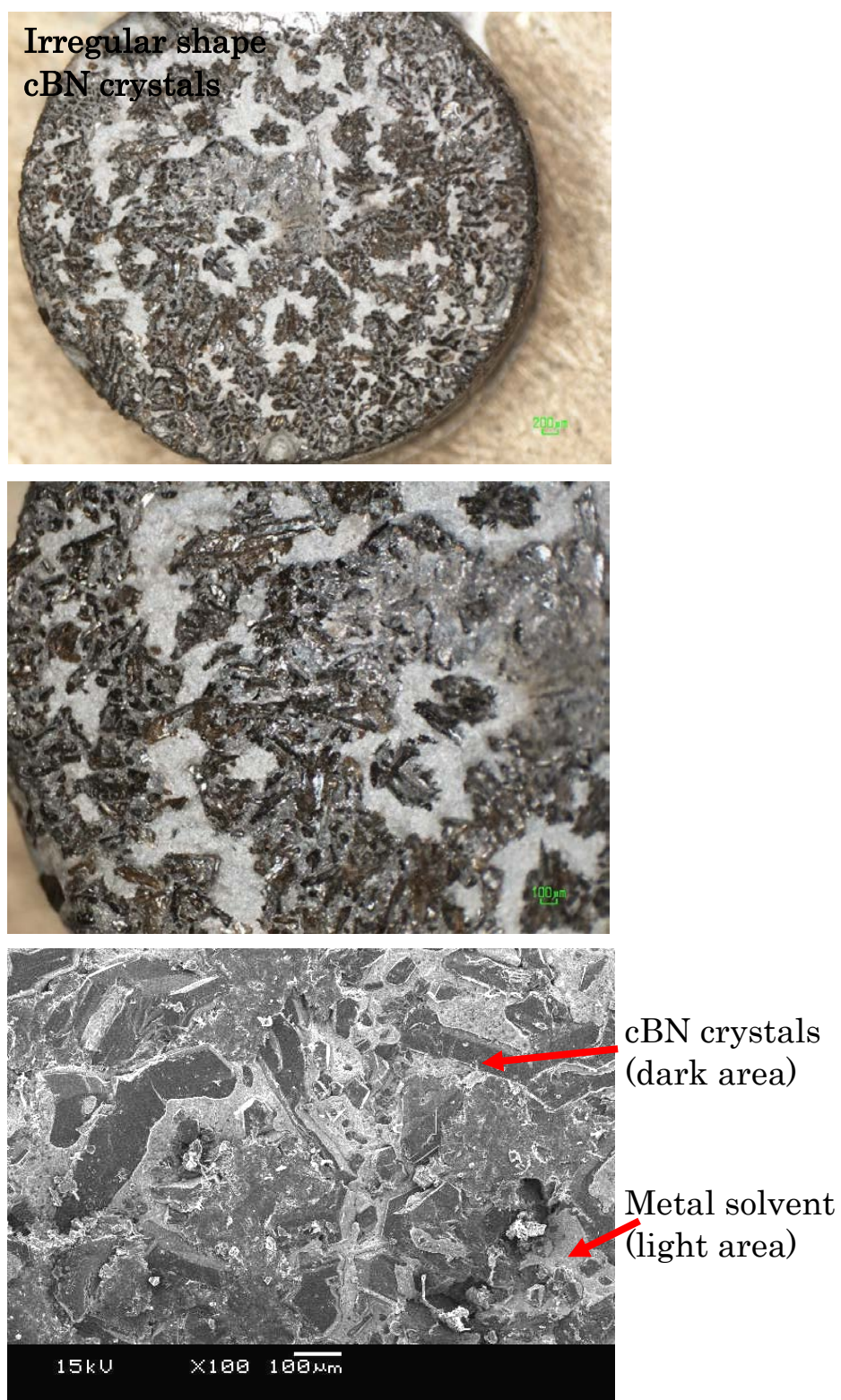
Fig.3.10. Optical photograph and SEM image of cBN synthesized using Fe 52.5 Ni 5.8 -Cr 38.8 -Al 2.9 solvent at 5 GPa 1320 °C 1 h.
