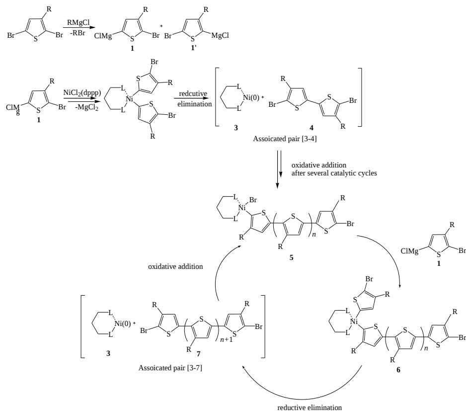
Scheme 1.2 Mechanism of Grignard metathesis method for the synthesis of regio-regular poly(3-alkylthiophene).
