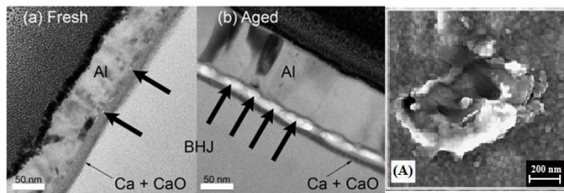
Figure 1.15 TEM images for (a) freshly prepared, (b) aged ITO/BHJ/Ca/Al device and (A) 500 nm size flaw on Al after aged, denoted by Lloyd et al. 21 .
