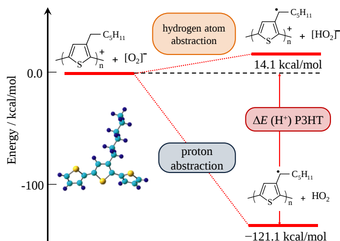
Figure 3.9 Energy diagram of [P3HT]^+ + [O_2]^- , [P3HT\cdot]^+ + [HO_2]^- , and [P3HT\cdot] + HO_2 . Superoxide anion [O_2]^- reacts with the \alpha -hydrogen and \alpha -proton of P3HT. Inset; model compound (3'-hexyl-2,2':5,2''-terthiophene) structure of P3HT.
