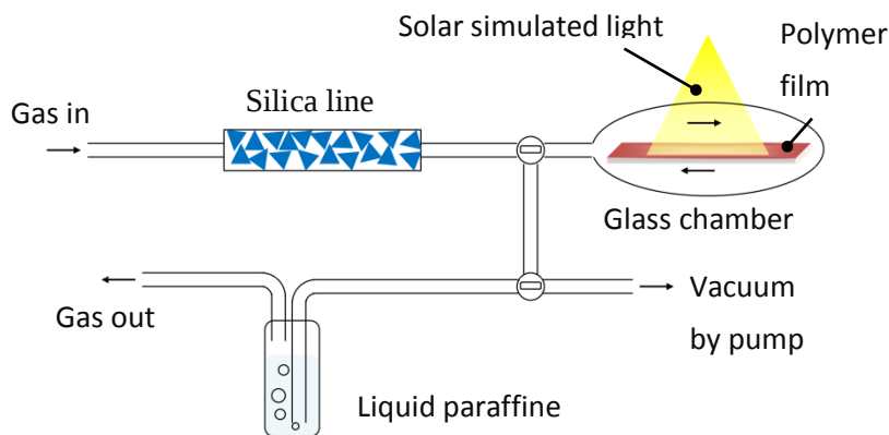
Figure 3.1 The experimental setup for gas perge.
