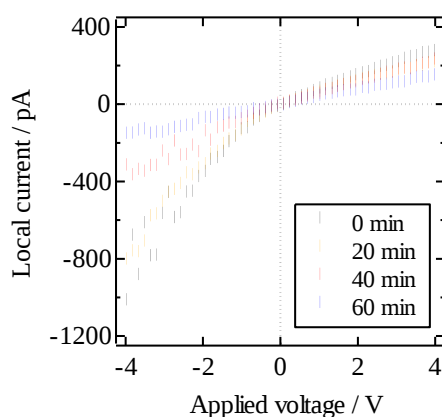
Figure 2.7 Local I-V curves of ITO/PEDOT:PSS/P3HT:PCBM/Pt/Ir tip device. Before fabrication, the blended solution was irradiated for (●) 0, (●) 20, (●) 40, and (●) 60 min in air using simulated solar light (AM 1.5 G) at an intensity of 100 \text{ mW/cm}^2 .
