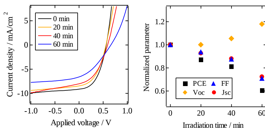
Figure 2.4 I-V curves for (—) 0, (—) 20, (—) 40, and (—) 60 min, and the changes in (■) PCE, (▲) FF, (◆) V_{oc} , and (●) J_{sc} of the ITO/PEDOT:PSS/P3HT:PCBM/Al device. Before fabrication of the organic film, the blended solution was irradiated in air using simulated solar light (AM 1.5 G) at an intensity of 100 mW/cm 2 .
