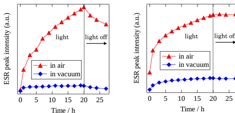
Figure 3.6 Temporal changes in the ESR peak intensities of (a) P3HT and (b) P3OOT films (▲) in air and (◆) in vacuum. The light condition: 0–20 h. The dark condition: 20–27 h.
