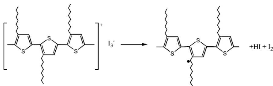
Scheme 3.1 Deprotonation reaction of [\text{poly(3-alkylthiophene)}]^+ , which is denoted in Koizumi et al. 31 .
