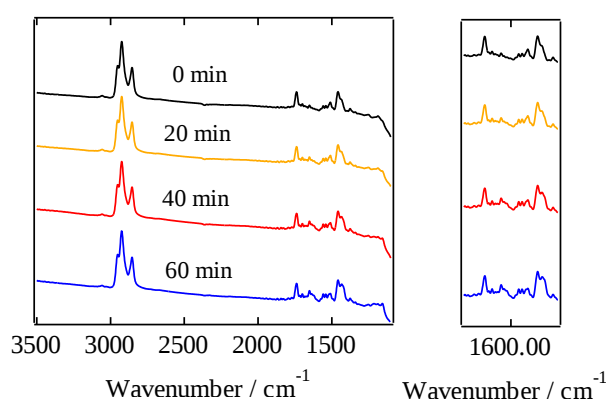
Figure 2.11 FT-IR spectra of P3HT:PCBM organic films. Before fabrication, the blended solution was irradiated for (—) 0, (—) 20, (—) 40, and (—) 60 min in air using simulated solar light (AM 1.5 G) at an intensity of 100\text{ mW/cm}^2 .
