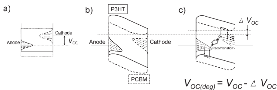
Figure 1.13 Schematic energy diagram of bulk heterojunction organic solar cells a) under the initial open circuit condition, b) under the initial short circuit condition, and c) after degradation. The carriers are accumulated in two trap sites. Alleviation of the energy band slope occurs, resulting in a decrease of V_{OC} , denoted by Kawano et al 18 .
