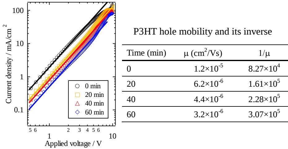
Figure 2.15 (left) I - V curve for (—) 0, (—) 20, (—) 40, and (—) 60 min of the ITO/PEDOT:PSS/P3HT:PCBM/Au device. (Right) P3HT hole mobility given by the Mott-Gurney law, J_{sclc} = \frac{9}{8} \epsilon_0 \epsilon_r \mu \frac{V^2}{L^3} . Before fabrication of the organic film, the blended solution was irradiated in air using simulated solar light (AM 1.5 G) at an intensity of 100 mW/cm 2 .
