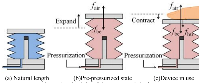
Figure 2 Principle of the proposed device
