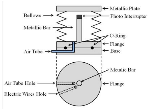
Figure 3 Structure of the proposed haptic device.
