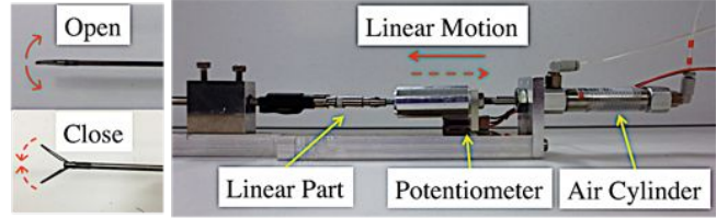
Figure 10 Pneumatic forceps
