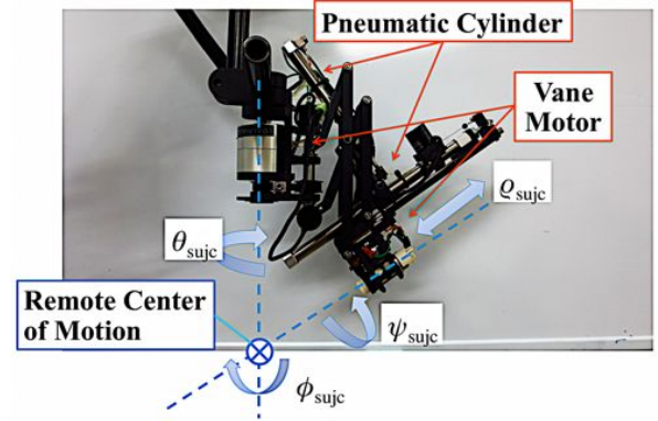
Figure 11 Forceps holder
