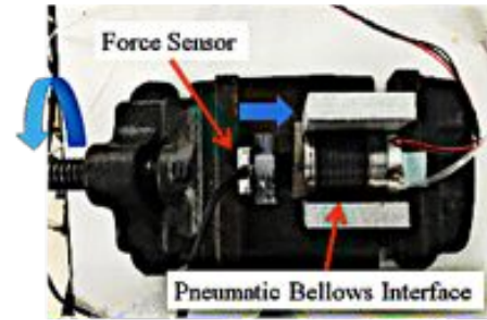
Figure 5 Performance experiment
