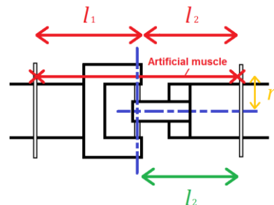
Fig. 5 Model diagram of the joint part when 2 arm segments are straight
