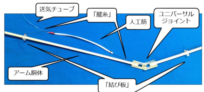
Fig. 2 One unit of the manipulator's drive system
