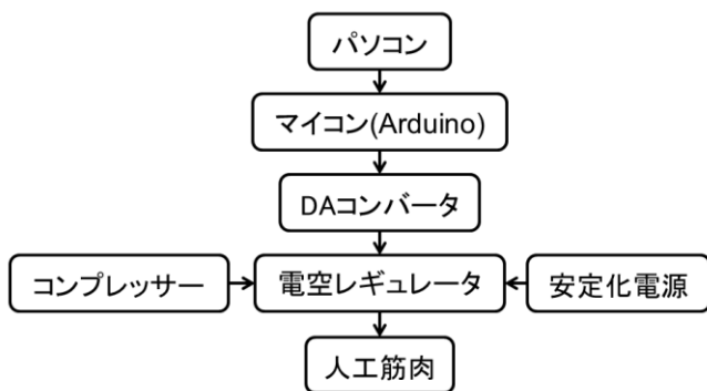
Fig. 8 Control system of the manipulator's drive
