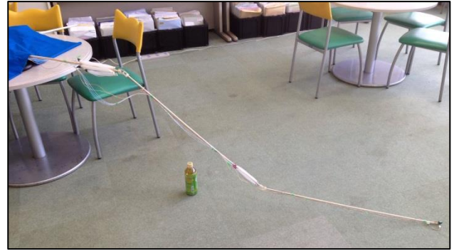
Fig. 9 Prototype of the robot arm
