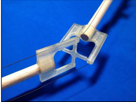
Fig. 3 Universal joint when “Tendon-strings” are passed through 2 “String-holes”
