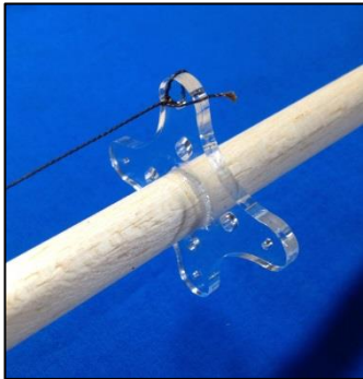
Fig. 4 “Knotting board” when “Tendon-string” is tied to “String-knotted-hole”
