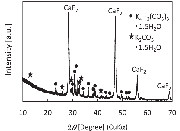
Fig. 6 X-ray diffraction pattern of the precipitate in the suspension with \text{Ca}(\text{OH})_2 and KF
