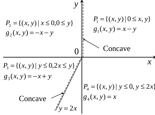
Figure 4.1: Two-variable piecewise linear function
