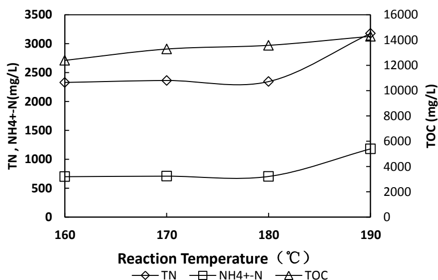
Fig. 2.8 Effect of the reaction temperature on TN, NH 4 + -N and TOC contents
