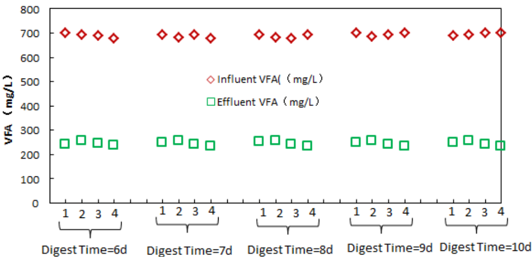
3.10 VFA concentration changes of the EGSB reactor with different digestion times
