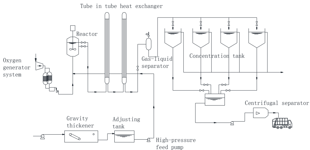
Fig. 1-10 Pilot reaction process of the hydrothermal drying combination technology
