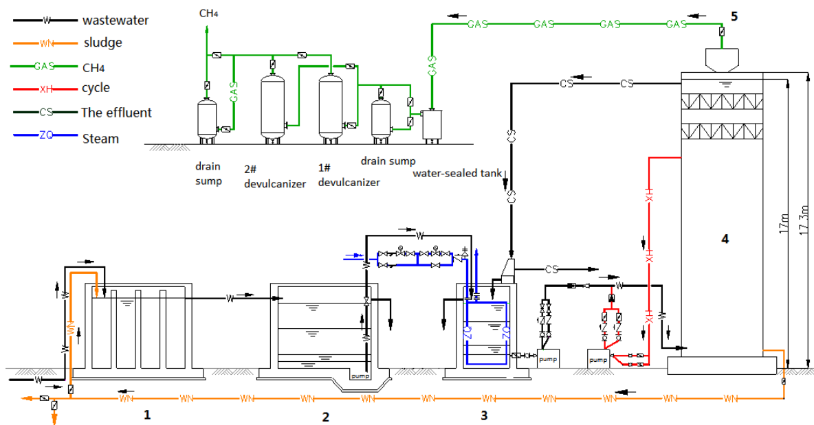
Figure 3.6 Process flow diagram of methane production from sludge
