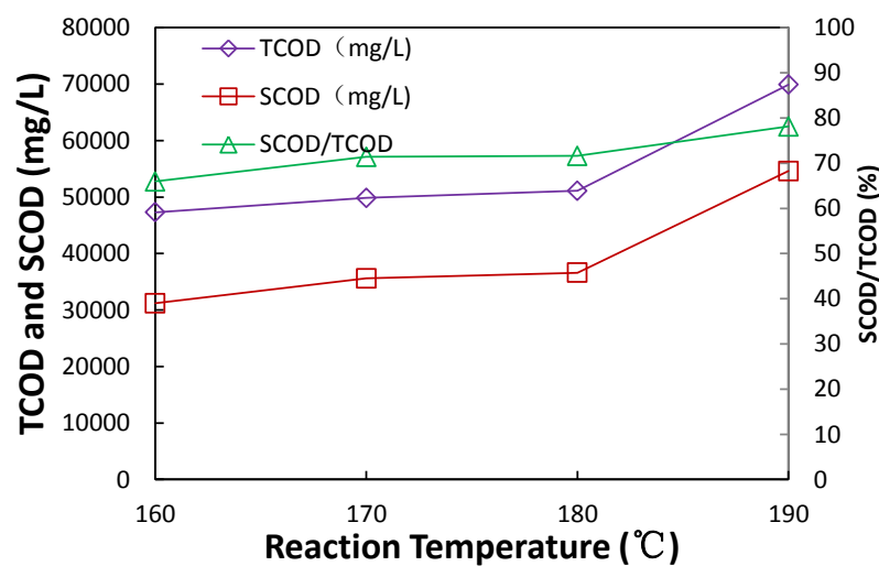
Fig. 2.6 Tendencies of TCOD, SCOD, and SCOD/TCOD in the separated liquid under different reaction temperatures
