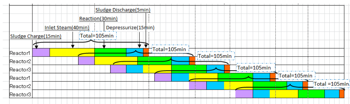
Fig. 4.6 Sequencing of three reactors working time in the energy-saving process
