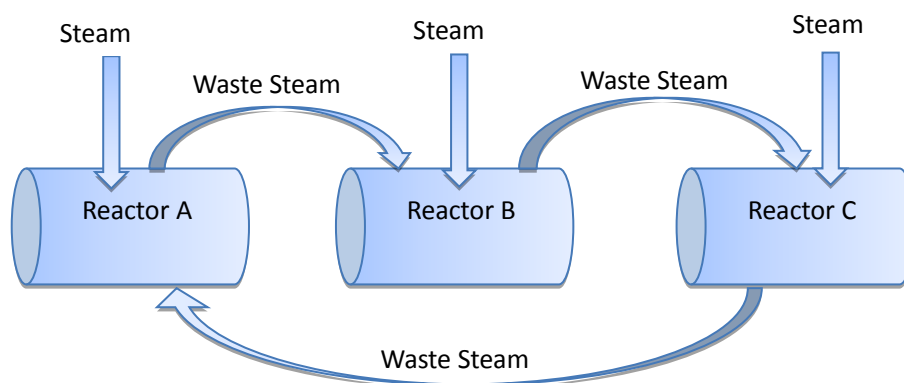
Fig. 4.4 Concept map of energy-saving for sludge hydrothermal system
