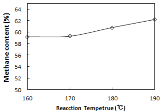
Fig. 2.12 The methane content of biogas product from the separated liquid under different reaction temperatures
