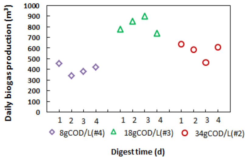
Fig. 3.11 Daily gas production of the EGSB reactor under different volume load regulations
