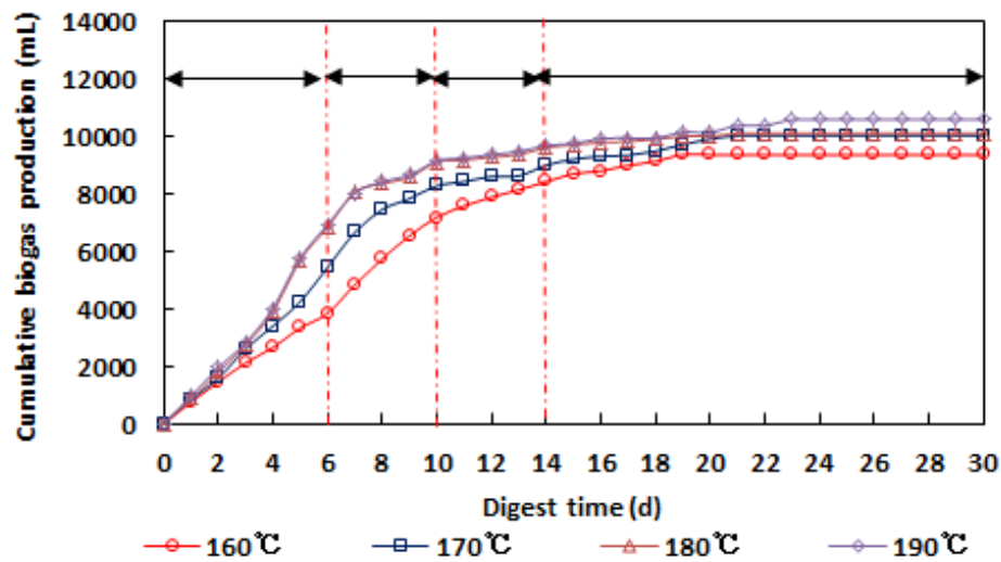
Fig. 2.11 Cumulative biogas production of the separated liquid under different reaction temperatures
