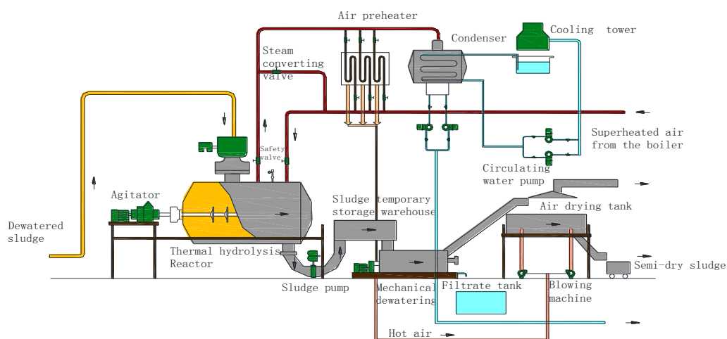
Fig. 1-9 Flow diagram of the water sludge thermal drying process developed by BMEI Co. Ltd.
