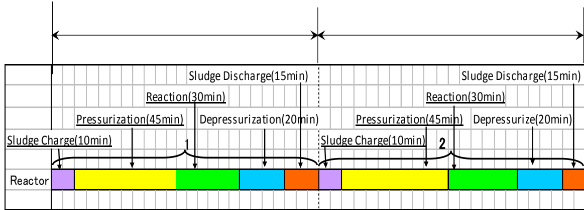
Fig. 4.2 One cycle time of the batch reactor under the design conditions [4-1]
