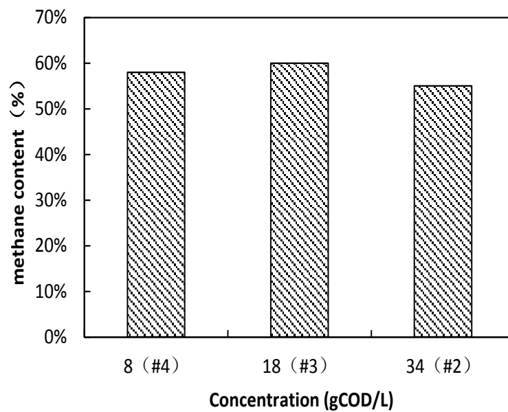
Fig. 3.13 Methane content with different influent CODs
