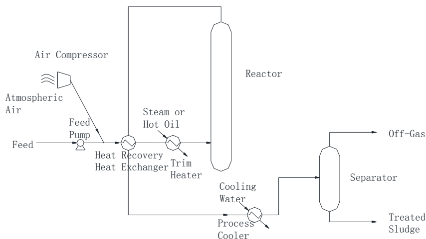
Fig. 1-4 Flow diagram of the Zimpro process
