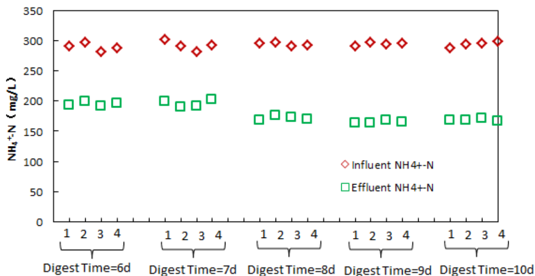
Fig. 3.8 Influent and effluent \text{NH}_4^+\text{-N} changes of the EGSB reactor with different digestion times
