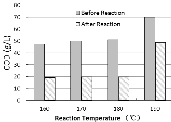
Fig. 2.13 COD changes before and after the anaerobic digestion
