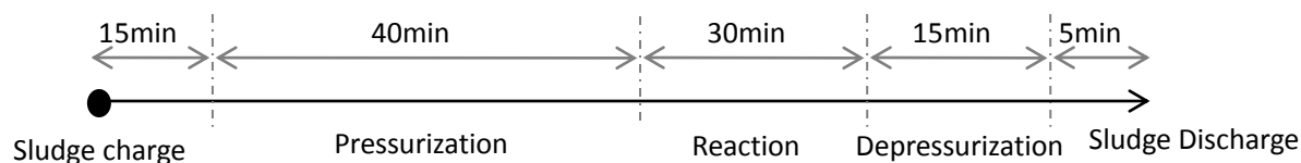
Fig. 4.5 One cycle time of the batch reactor for the optimization process
