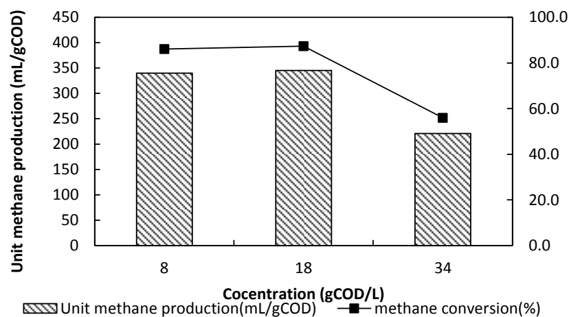
Fig. 3.12 Unit methane production and methane conversion with different influent CODs
