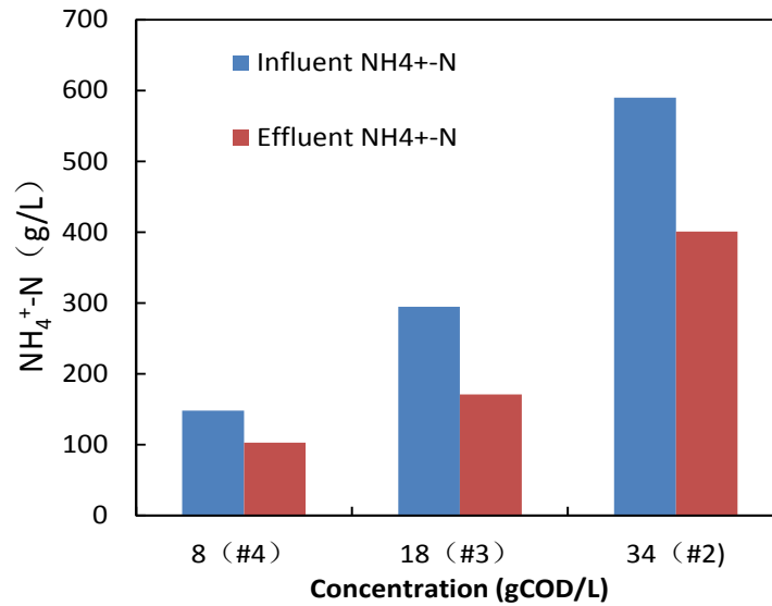
Fig. 3.9 NH 4 + -N changes of different influent CODs
