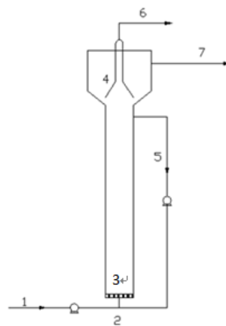
Figure 3.4 Schematic of the EGSB
