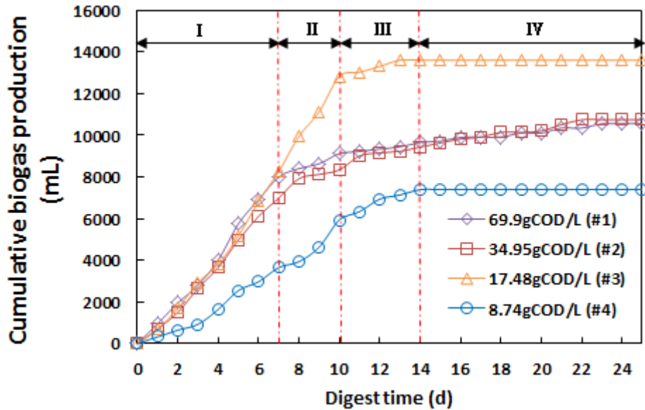
Fig.2.14 Cumulative biogas production of separated liquid with different dilution rate
