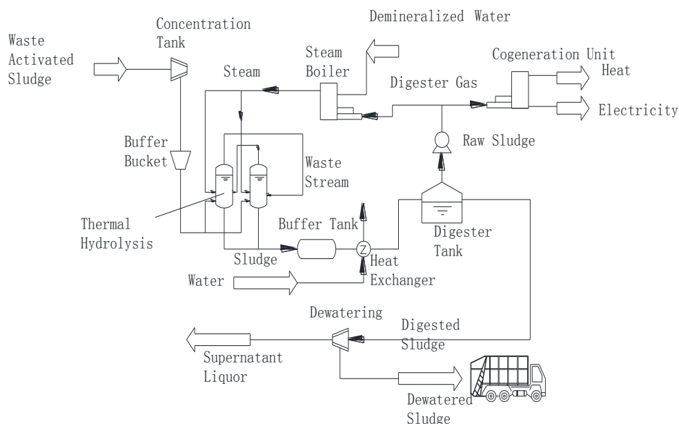
Fig. 1-5 Flow diagram of the Biorthelys process
