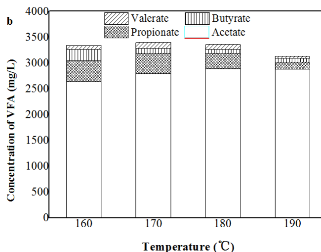
Fig. 2.7 Tendencies of VFA in sludge separated liquid under different reaction temperatures
