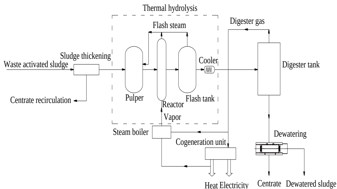
Fig.1-6 Flow diagram of the Cambi™ process
