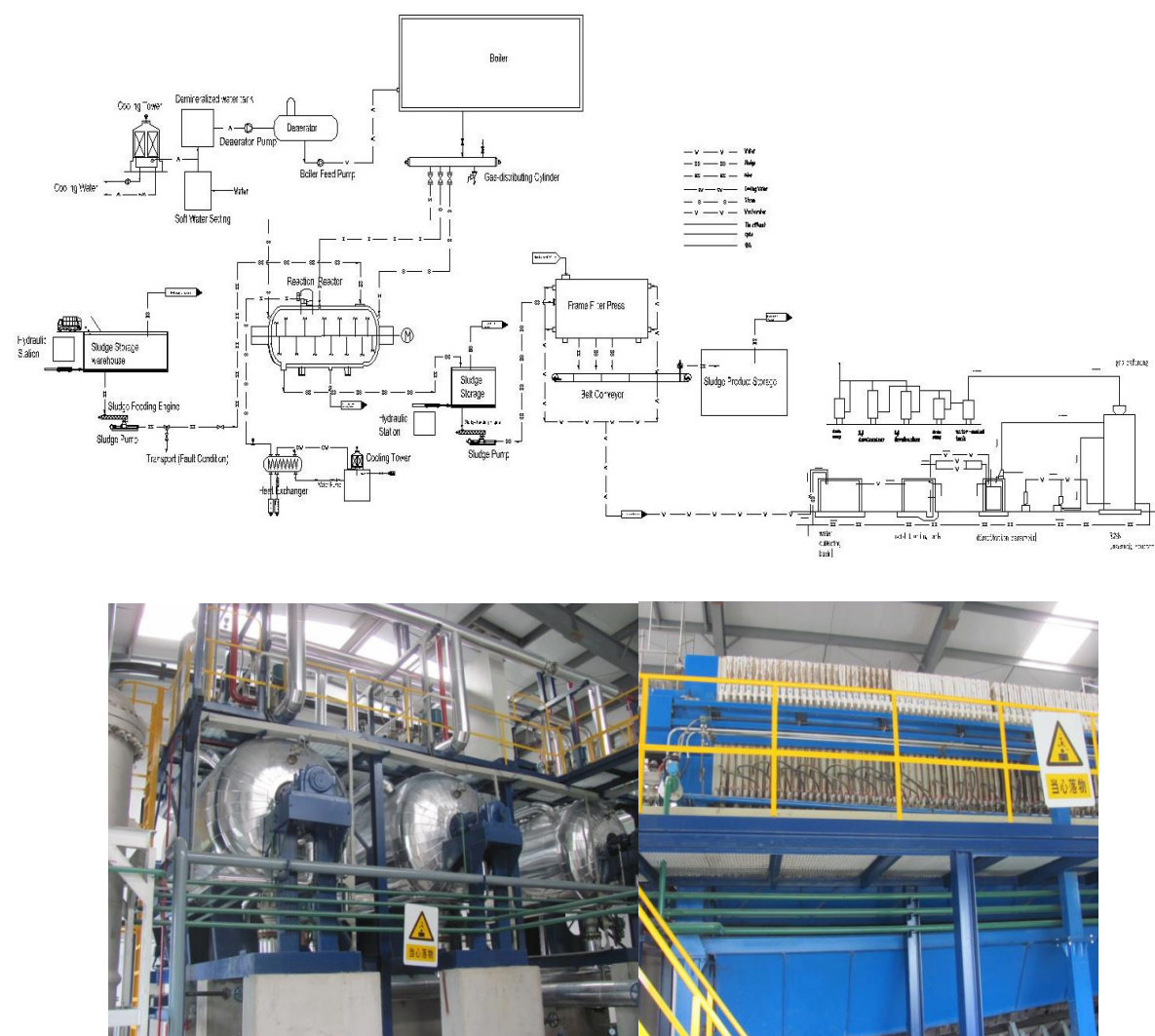
Fig. 4.1 Process flow diagram of the commercial plant
