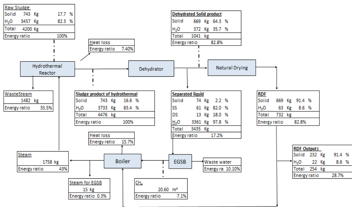
Fig. 4.3 Energy balance with RDF and CH 4 recycles
