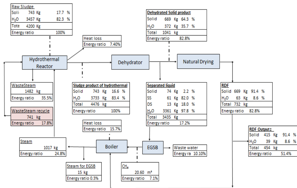
Fig. 4.7 Mass and energy balances with RDF, waste steam and CH 4 recycles
