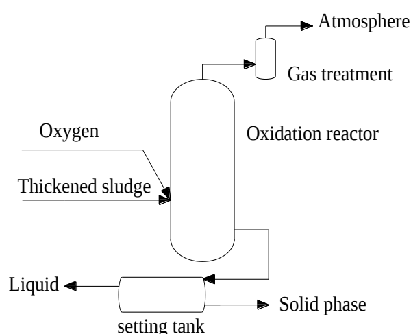
Fig. 1-8 Flow diagram of the Athos™ WAO process
