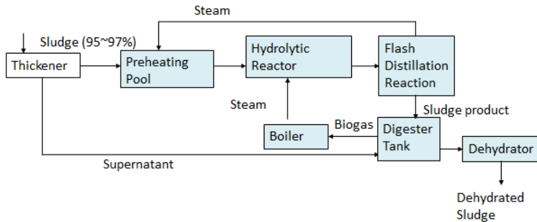
Fig. 4.9 Process of sludge hydrothermal treatment technology 1
