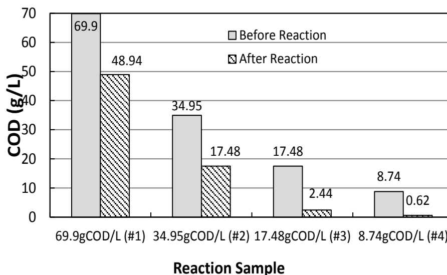
Fig.2.16 The changes of COD before and after the anaerobic digestion
