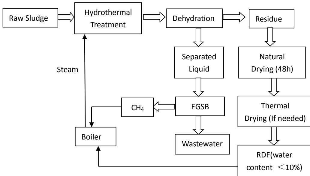
Figure 4.8 Flow Chart of the hydrothermal treatment System
