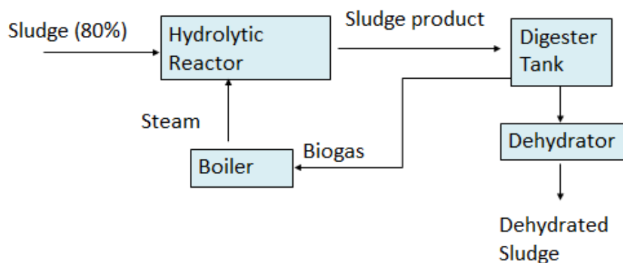
Fig. 4.10 Process sludge hydrothermal treatment technology 2
