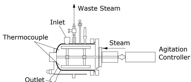
Fig. 2.1 The hydrothermal reactor of the small-scale facility
