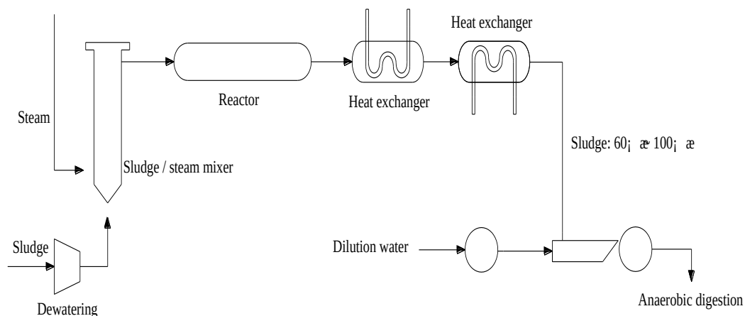
Fig. 1-7 Flow diagram of the Exelys™ process
