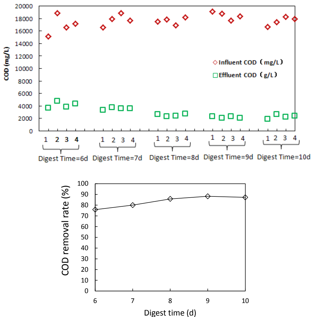
Figure 3.7 Influent and effluent COD changes of the EGSB reactor with different digest times
