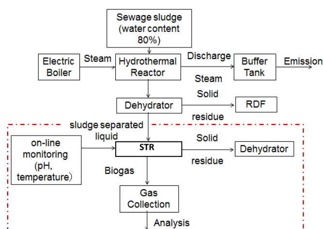
Fig. 2.5 The experimental procedure
