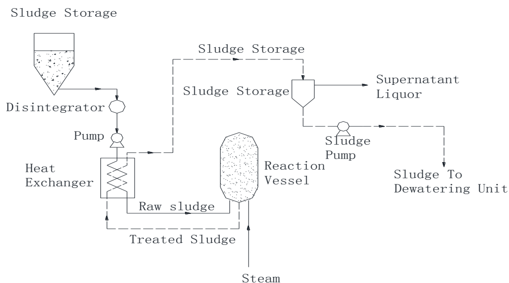
Fig. 1-3 Flow diagram of the Porteous process
