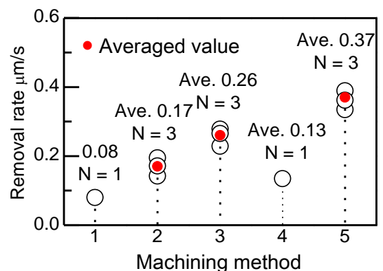
Fig. 2.31 Removal rate
