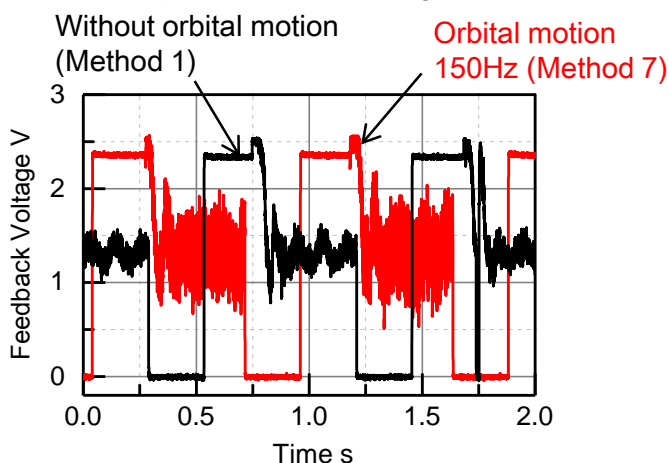
Fig. 4.39 Feedback voltage
