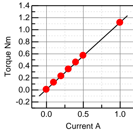
Fig. 3. 7 Relationship between i_0 and torque (Simulated)
