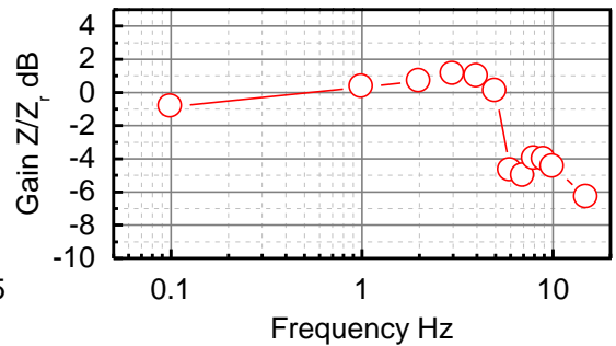
Fig. 2.20 Bode diagram of positioning stage of conventional EDM machine
