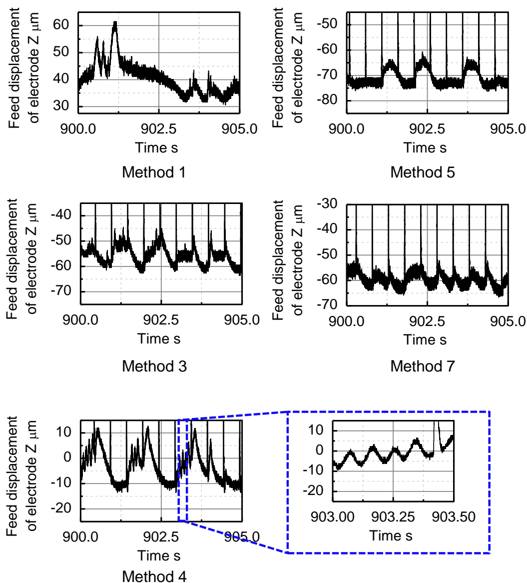
Fig. 4. 10 Feed displacement of electrode
