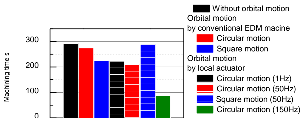
Fig. 4.37 Machining time
