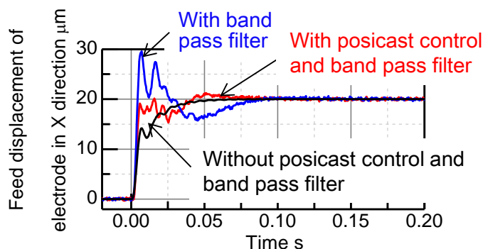
Fig. 4.28 Step response of electrode (Experimental)
