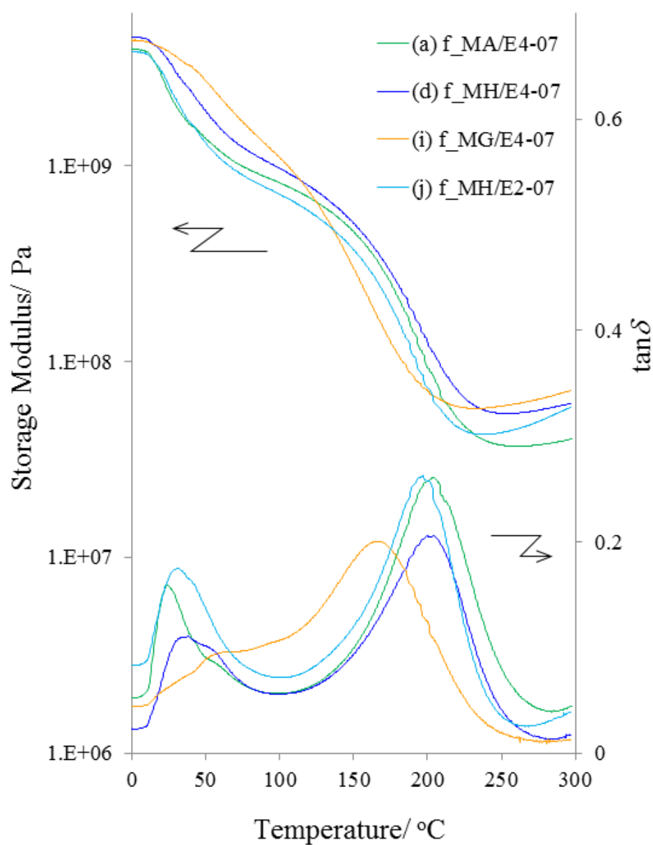
Figure 7. The temperature dependence of storage modulus and \tan \delta for (a) f\_MA/E4 , (d) f\_MH/E4 , (i) f\_MG/E4 , and (j) f\_MH/E2 measured by DMA.
