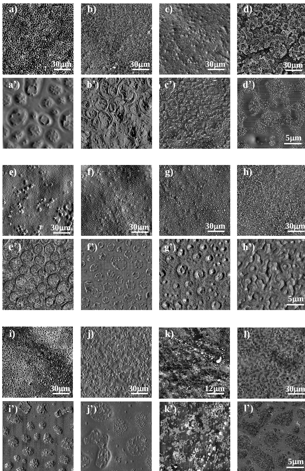
Figure 3. SPM phase image of 125μm square for (a) f_MA/E4, (b) f_Mh/E4, (c) f_MhL/E4, (d) f_MH/E4, (e) f_MHiP/E4, (f) f_MHB/E4, (g) f_MBz/E4, (h) f_MHBz/E4, (i) f_MG/B4, (j) f_MH/E2, (k) f_MH/E4-TPE*, and (l) f_MH/E4_C and the image of 20μm square of each accompanied the letter with apostrophe.
