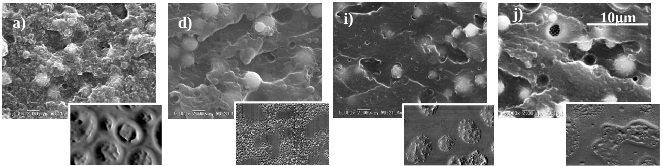
Figure 8. Cross section after fracture toughness test at 250°C observed by SEM. (a) f_MA/E4, (d) f_MH/E4, (i) f_MG/B4, (j) f_MH/E2 (The insets are SPM image shown in Figure 3 in the same magnification)
