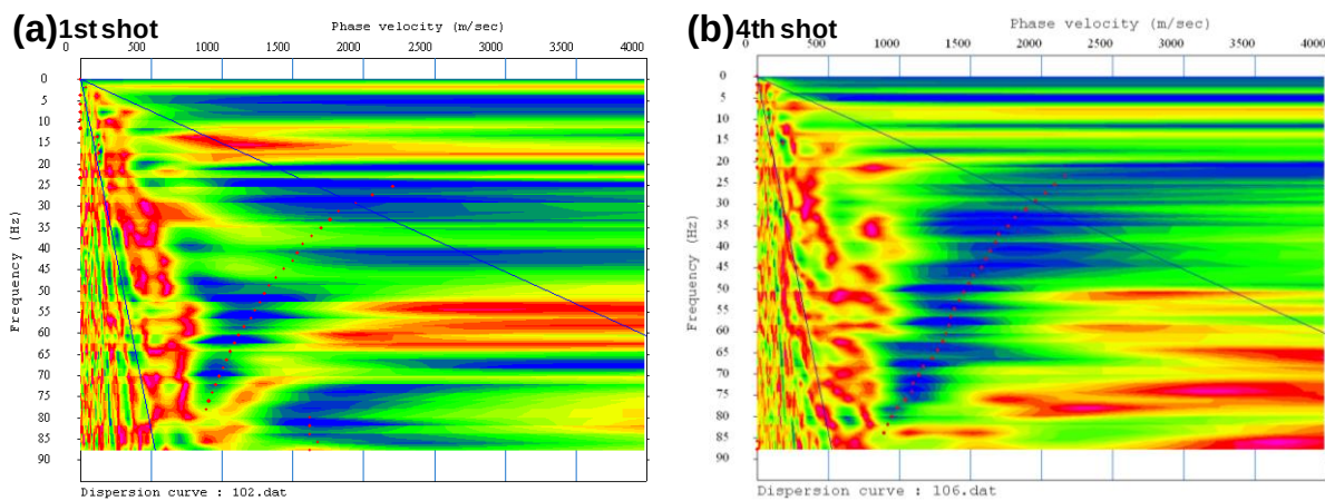
Figure 26. Images of dispersion curves obtained at LMO rock site for (a) first shot, and (b) forth shot.
