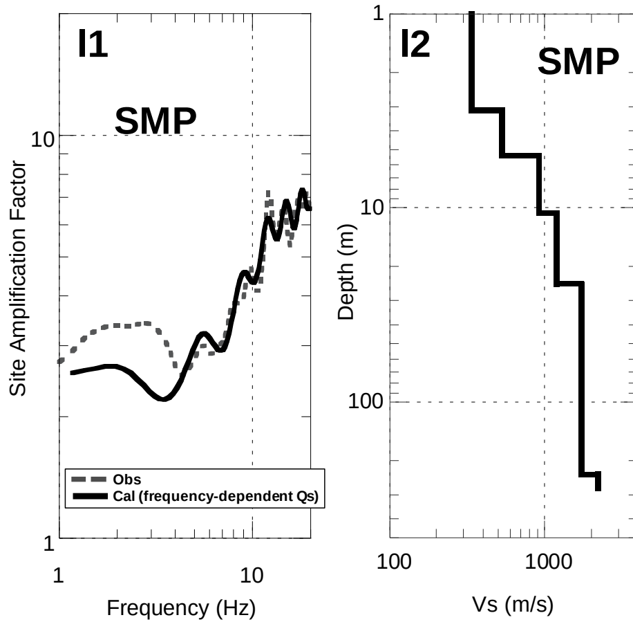
Figure 41 (l). (l1) Comparison of observed site response (grey dashed line) and theoretical amplification factors with the assumption frequency-dependent Q_s (black solid line). (l2) Black line indicates S-wave velocity model obtained from inversion. No S-wave velocity subsurface structure was previously available at SMP station.
