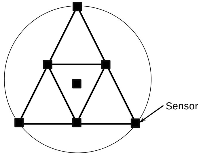
Figure 12. Geometry of the microtremor array.
