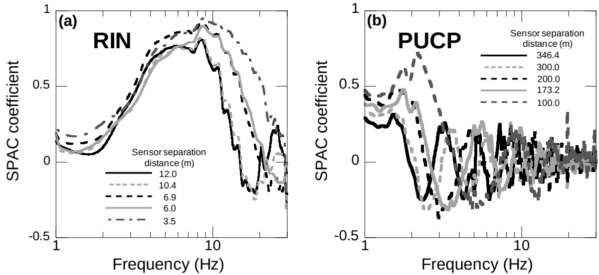
Figure 14. SPAC coefficients as a function of frequency for different sensor separation distances at (a) the RIN site (with a maximum side length of 12.0 m) and (b) the PUCP site (with a maximum side length of 346.4 m).
