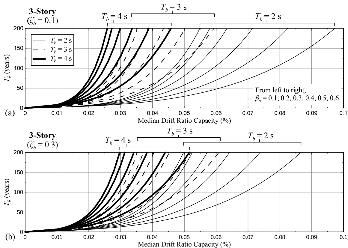
Figure 4.13 Performance curves for drift-sensitive components (3-story)
