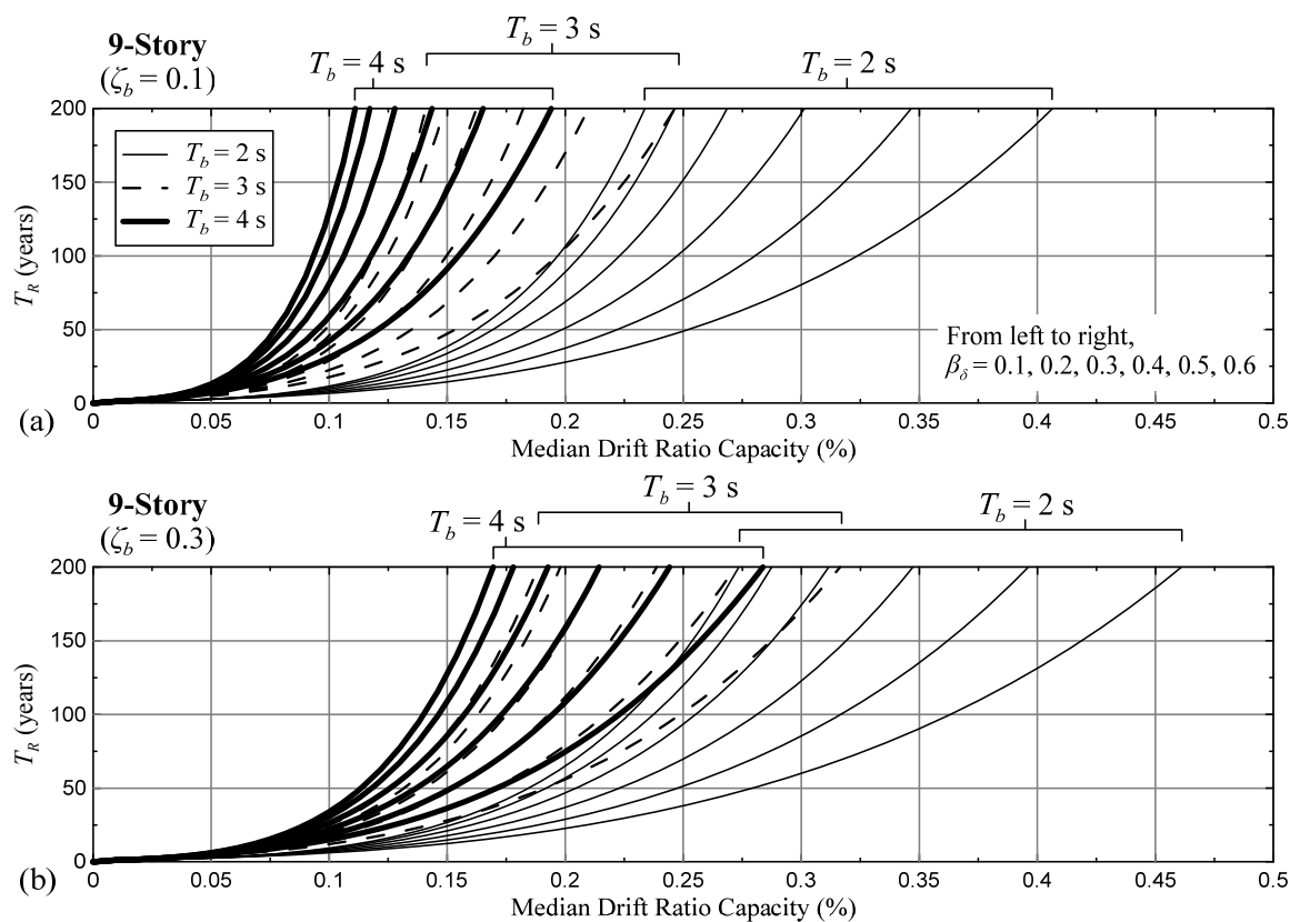
Figure 4.14 Performance curves for drift-sensitive components (9-story)
