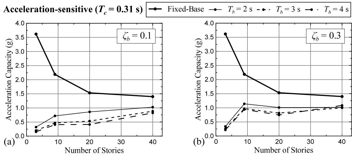
Figure 4.30 Acceleration capacities ( T_c = 0.31 s) for T_R = 100 years
