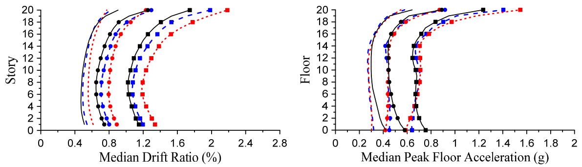
(c) 20-story
