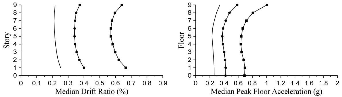
(b) 9-story
