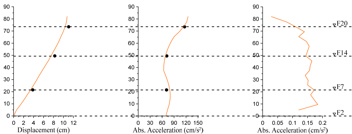
Figure 6.76 Envelope responses
