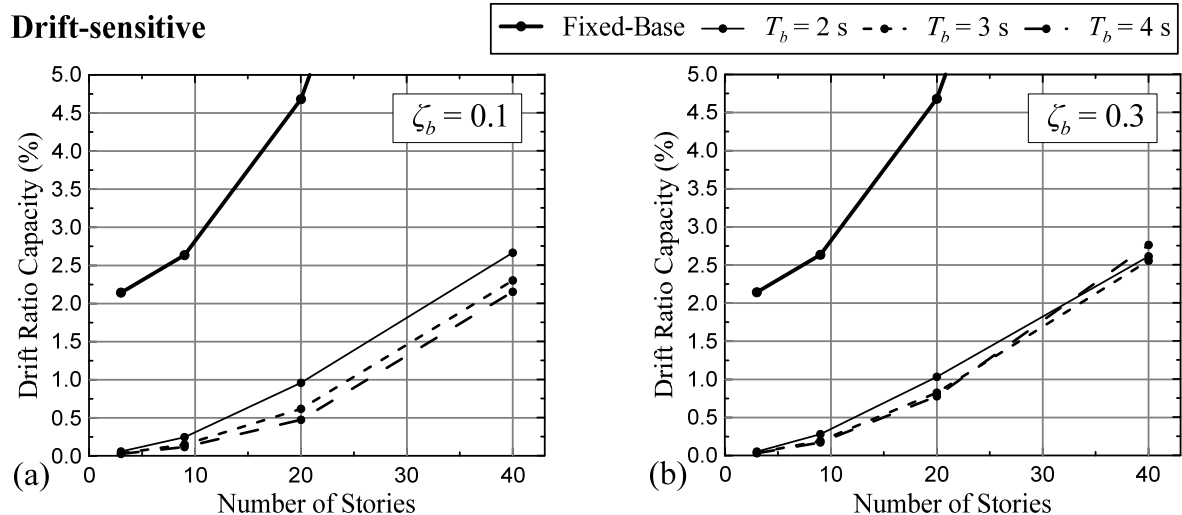
Figure 4.28 Drift ratio capacities for T_R = 100 years
