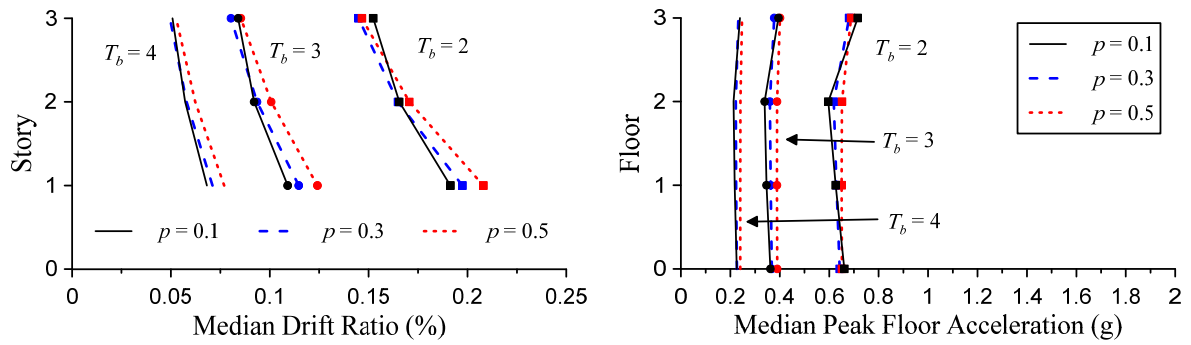
(a) 3-story
