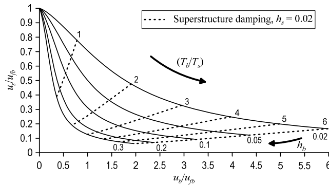
(b) Performance curve
