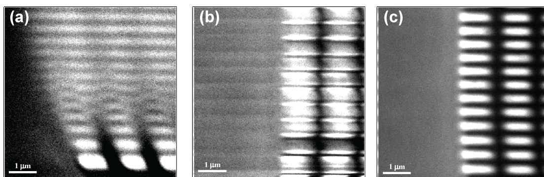
Figure 4.6 Nanomembrane and nanowire area (6 μm x 6 μm) scanned with different environmental parameters: (a) room air conditioning OFF, autofocus system OFF and thermal control booth OFF; (b) room air conditioning ON, autofocus system ON and thermal control booth OFF; (c) all three systems are turned ON.
