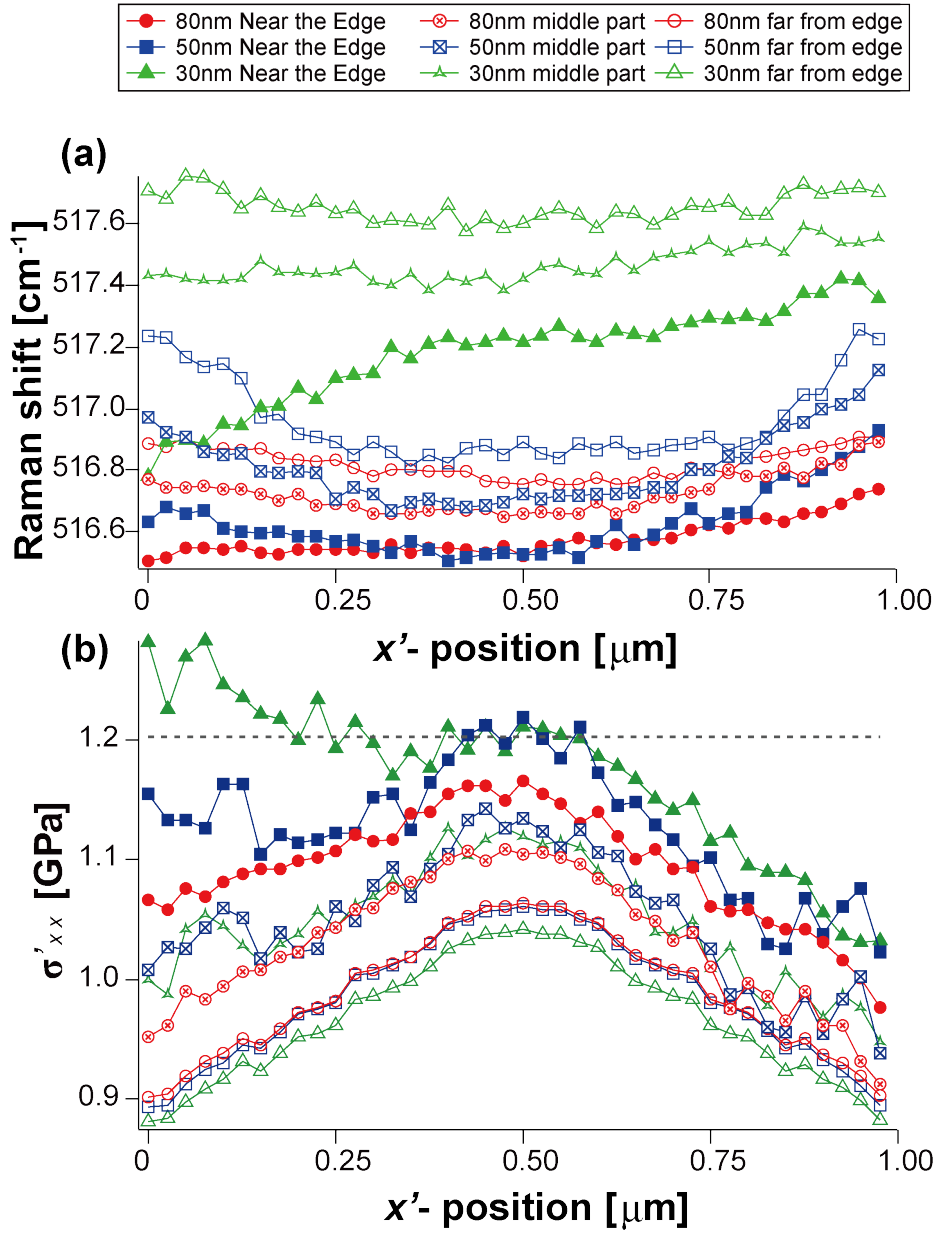
Figure 4.12. Raman shift along the x' -axis of the \epsilon -SiNWs show that the Raman shift (a) increases from the near edge to the middle region up to the far from edge. (b) The stress along the x' -axis exhibits relaxation from the center to the going to the edge of the NW, with NWs near the edge having higher stress compared to the middle part and far from edge region. Gray dashed line indicates the stress on an unpatterned nanomembrane.
