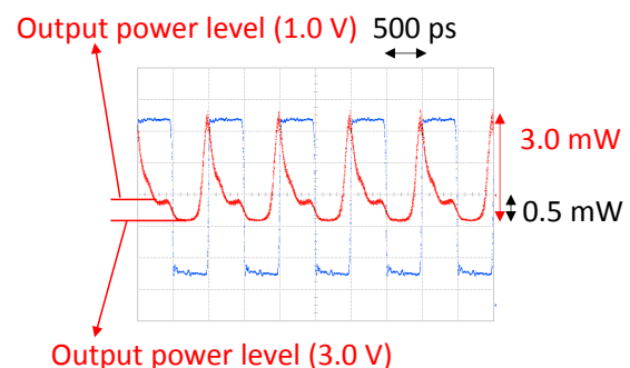
Fig. 3. Output signal at 1 GHz.
