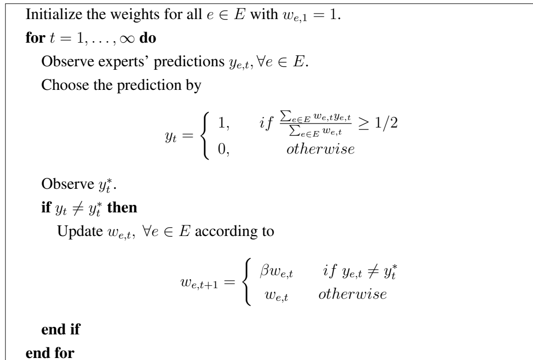
Figure 2.1: Weighted majority algorithm
