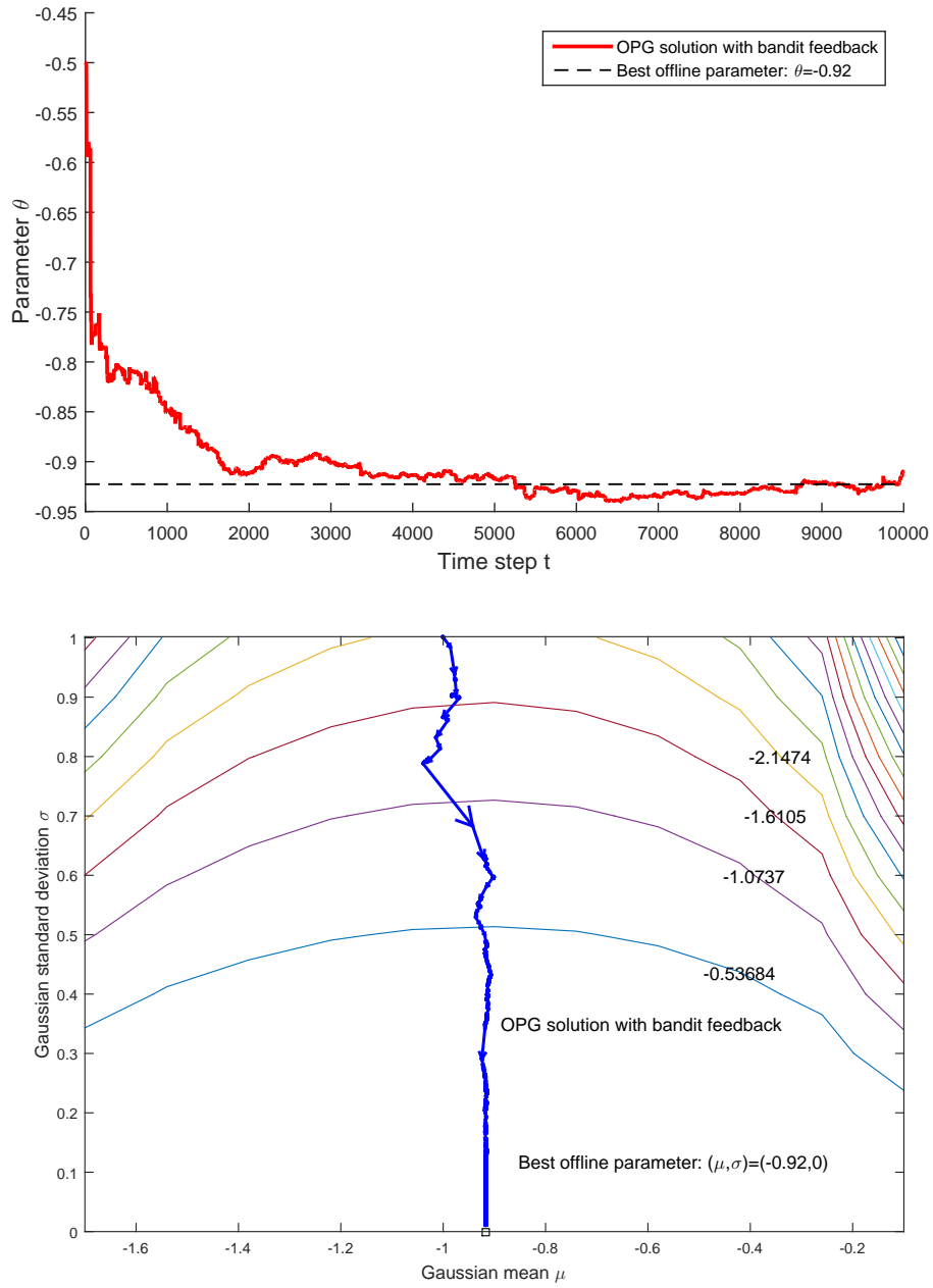
Figure 3.5: Trajectory of the OPG solution with bandit feedback and the best of-fine parameter.
