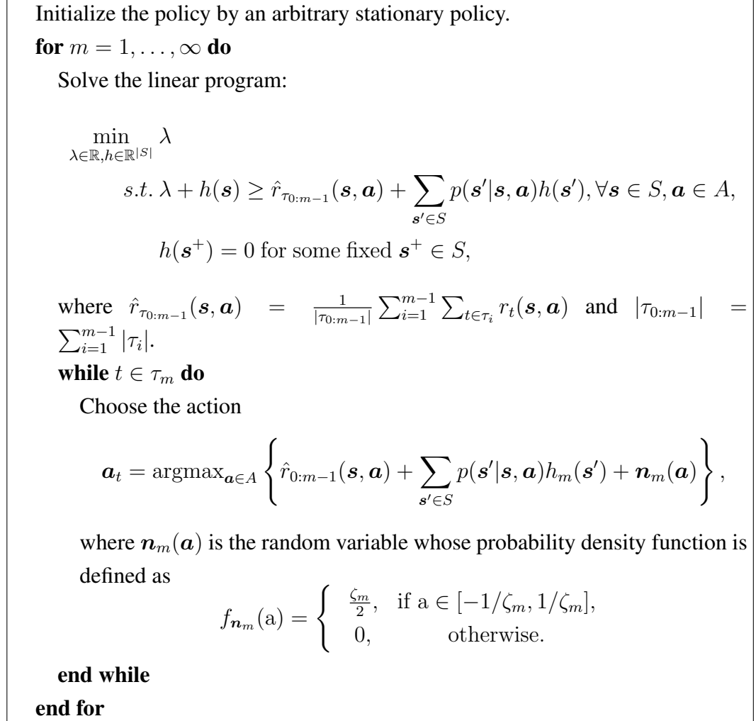
Figure 2.4: Lazy Follow the Perturbed Leader (Lazy-FPL) Algorithm
