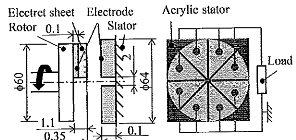
Fig. 1 Configuration of the electrostatic induction type generation with electret sheets
