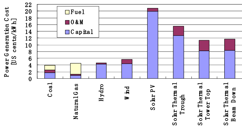
Fig. 5 Power generation cost of renewable energy and fossil energy.
