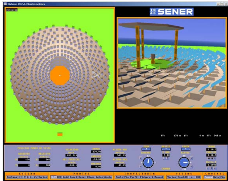
Fig. 2 Field design with SENSOL for BDS applications.
