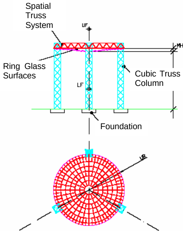
Fig. 4 Multi-ring central reflectors for BDS.
