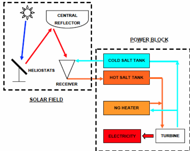
Fig. 1 Beam-Down energy flow diagram.
