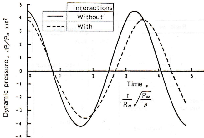
FIG. 5 TIME HISTORY OF DYNAMIC PRESSURE IN POOL
