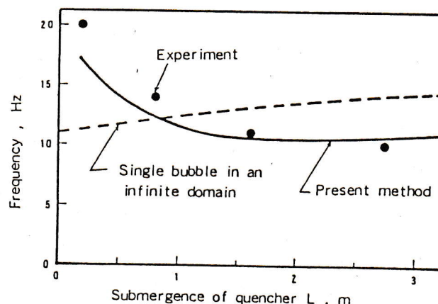
FIG.11 CHANGE OF FREQUENCY WITH BUBBLE SUBMERGENCE VARIED
