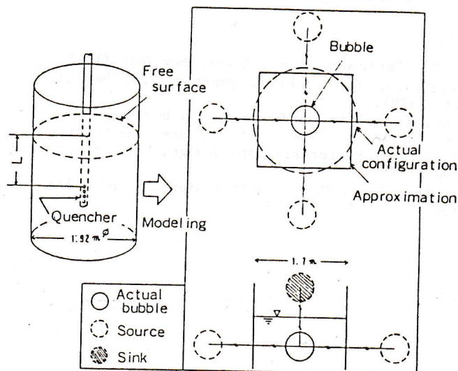
FIG.10 MODELING OF TEST TANK
