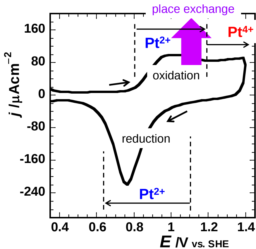
Fig. 5.1. Potential regions for dissolution of \text{Pt}^{2+} and \text{Pt}^{4+} from bulk samples under potential cycling in 0.5 M \text{H}_2\text{SO}_4 .
