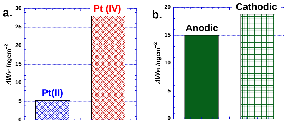
Fig. 3.11. Comparisons of \text{Pt}^{2+}/\text{Pt}^{4+} and anodic/cathodic Pt dissolutions in \text{Cl}^- -contaminated 0.5 \text{ H}_2\text{SO}_4 solution.
