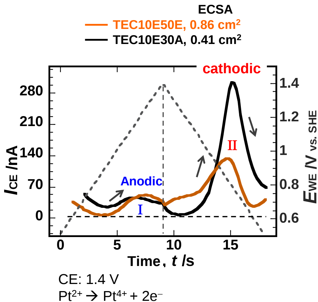
Fig. 4.11. I_{CE} plotted against time at 65 °C, while the WE loaded with TEC10E50E and TEC10E30A underwent CV at 100 mV/s.
