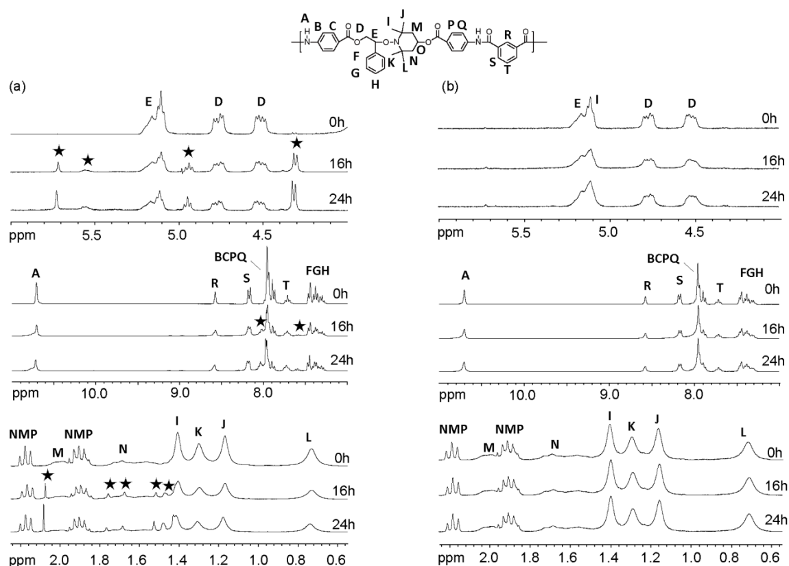
Figure 5-5 ^1\text{H} NMR spectra of TEMPO-PA heated at 130 °C for 0, 16, and 24 h under (a) an air and (b) argon atmosphere. The asterisked peaks cannot be assigned to the peaks corresponding to TEMPO-PA , indicating that side reactions occurred in the presence of oxygen in addition to the reversible recombination reaction between the nitroxide and styryl radicals.
