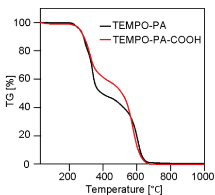
Figure 5-4 TG curves of TEMPO-PA and TEMPO-PA-COOH .
