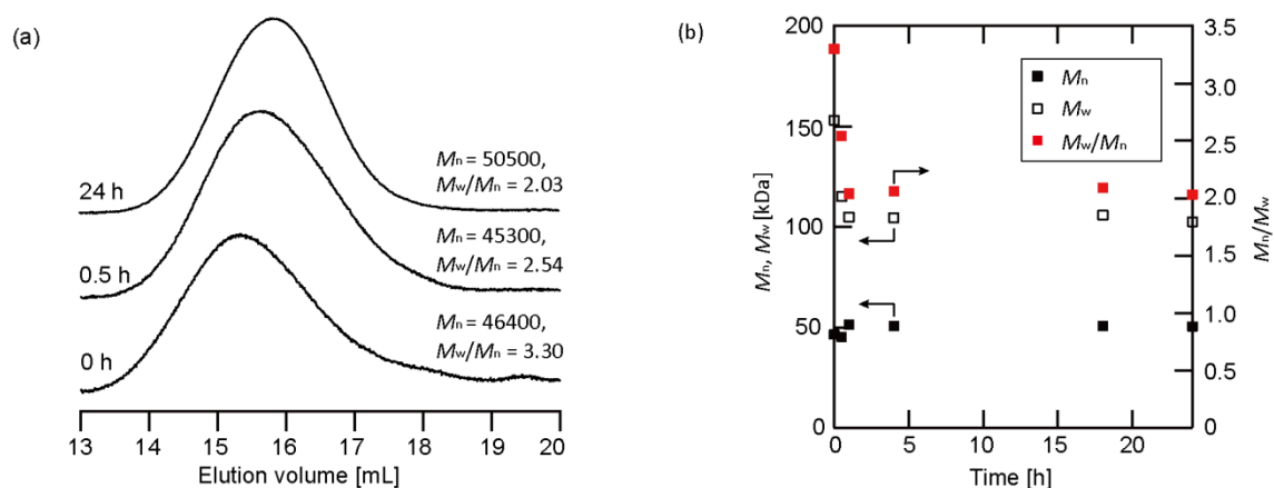
Figure 5-6 (a) GPC RI curves for TEMPO-PAs with heat treatment in DMF at 130 °C for 0, 0.5, 24 h. (b) Plots of M_n , M_w , and M_w/M_n as a function of time for TEMPO-PAs with heat treatment in DMF at 130 °C for 0, 0.5, 24 h.
