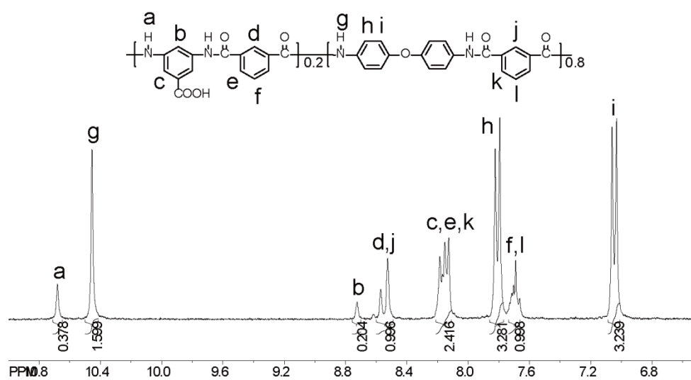
Figure 2-2 1 H NMR spectrum of PA2-20 .
