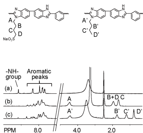
Figure 4-1 The ^1\text{H} NMR spectra of the (a) PBI , (b) BSPBI , and (c) BPBI in \text{DMSO}-d_6 at 40^\circ\text{C} .
