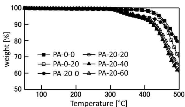
Figure 3-3 TG curves of PA-X-Ys under nitrogen atmosphere.
