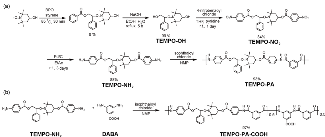
Scheme 5-1 Synthesis of (a) TEMPO-PA and (b) TEMPO-PA-COOH .
