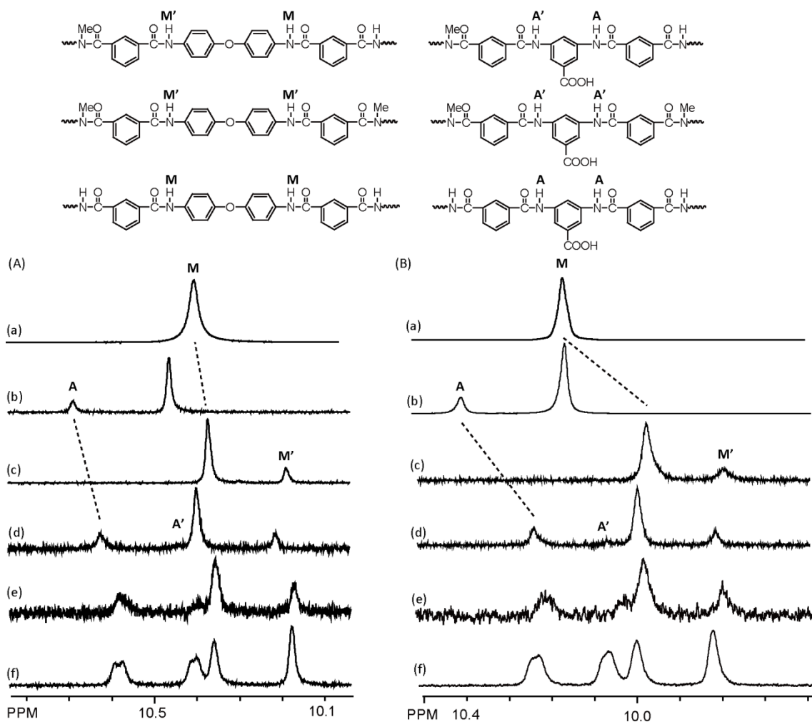
Figure 3-4 ^1\text{H} NMR spectra showing the region of the amide linkage signals of (a) PA-0-0 , (b) PA-20-0 , (c) PA-0-20 , (d) PA-20-20 , (e) PA-20-40 , and (f) PA-20-60 in \text{DMSO}-d_6 at (A) 40 and (B) 100 °C.
