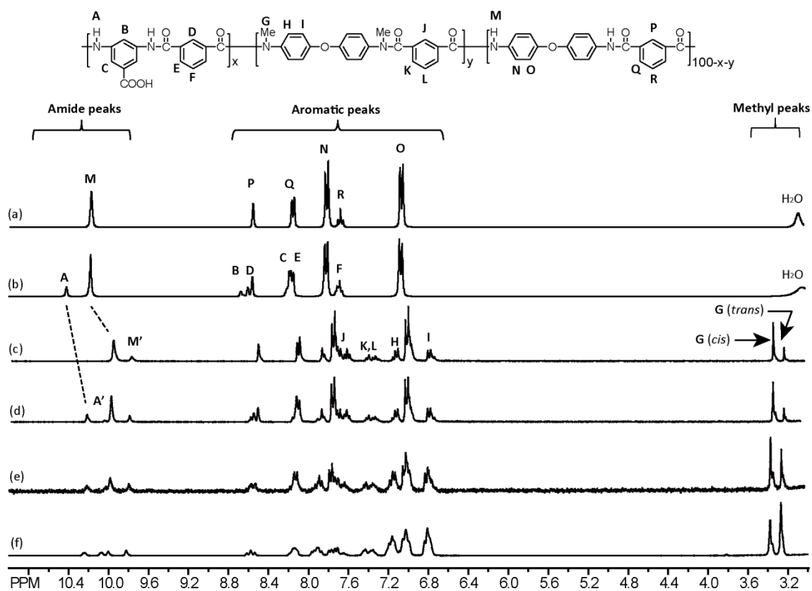
Figure 3-2 ^1\text{H} NMR spectra of (a) PA-0-0 , (b) PA-20-0 , (c) PA-0-20 , (d) PA-20-20 , (e) PA-20-40 , and (f) PA-20-60 in \text{DMSO-}d_6 at 100^\circ\text{C} .
