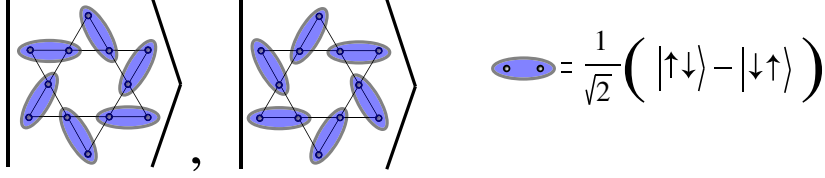
(a) Valence-bond-solid (VBS)
