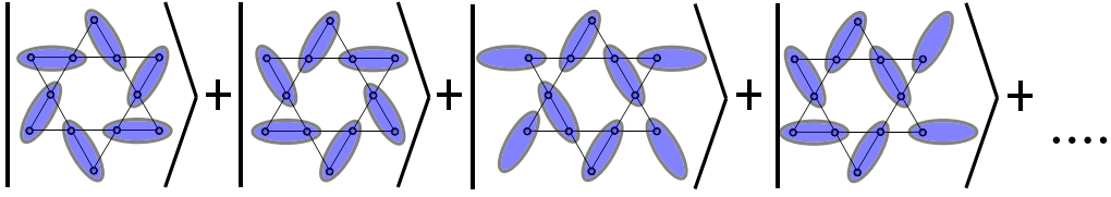
(b) Resonating-valence-bond (RVB)
