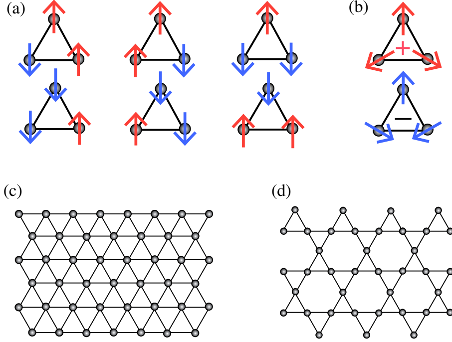
Figure 1.1: Illustration of frustration and frustrated lattices. (a) Ising spins coupled via antiferromagnetic exchange interaction on a triangle. Any spin configurations cannot be optimized with respect to Ising Hamiltonian. (b) XY or Heisenberg spins coupled via antiferromagnetic exchange interaction on a triangle. + and - indicate a vector chirality \kappa with the amplitude of +1 or -1. (c) Triangular lattice and (d) kagome lattice, which are typical geometrically frustrated lattices.
