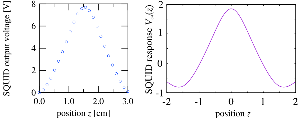
Figure 2.6: (a) Typical SQUID response as function of the sample position z and (b) response with Eq. 2.4, where the parameters X(1) = X(2) = X(4) = 0 , X(3) = 1 , R = 0.97 , and \Lambda = 1.517 are used.
