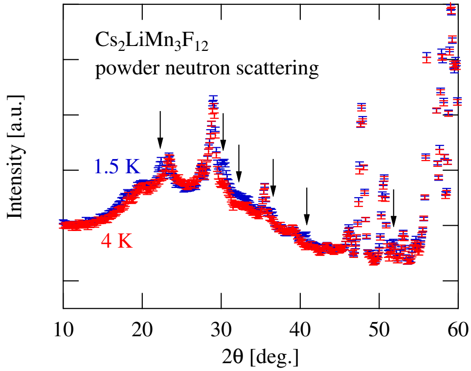
Figure 4.8: Neutron diffraction intensities of Cs 2 LiMn 3 F 12 measured at 1.5 K and 4 K. Small magnetic peaks indicated by arrows are observed.
