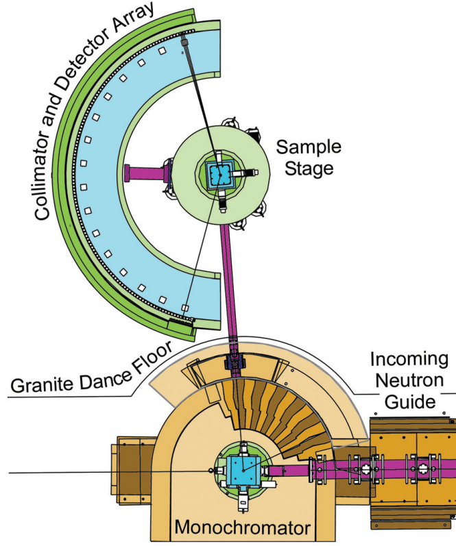
Figure 2.9: View of Echidna spectrometer at Australian Nuclear Science and Technology Organisation (ANSTO) reprinted from Ref. [129]. Echidna is a high resolution powder diffractometer.
