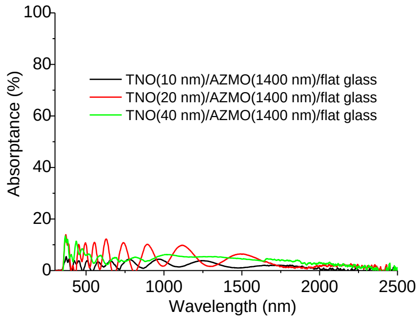
Fig. 5.9 Absorbance of AZMO/flat glass substrates coated with TNO.
