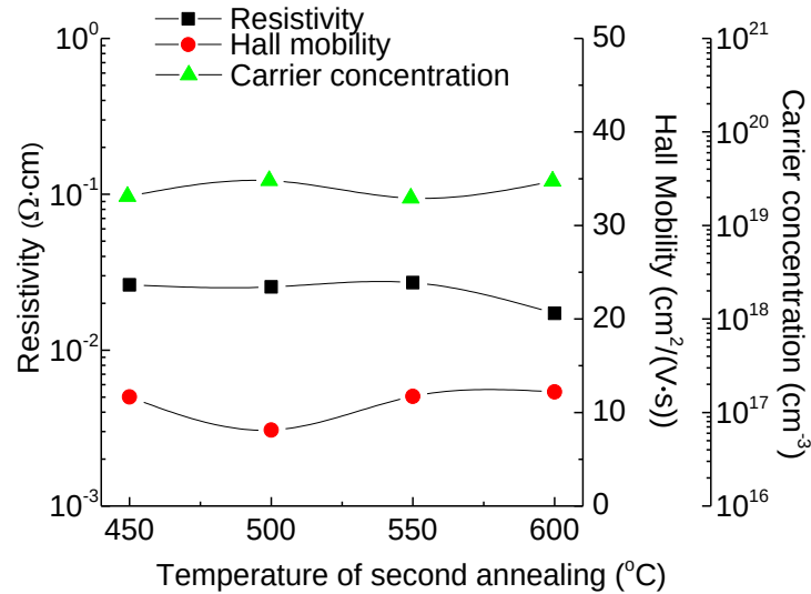
Fig. 3.58 Hall measurement results of AZMO films after the first annealing in air and the second annealing in FG with GC. The first annealing temperature was fixed at 500 °C, while the second annealing temperature was changed.
