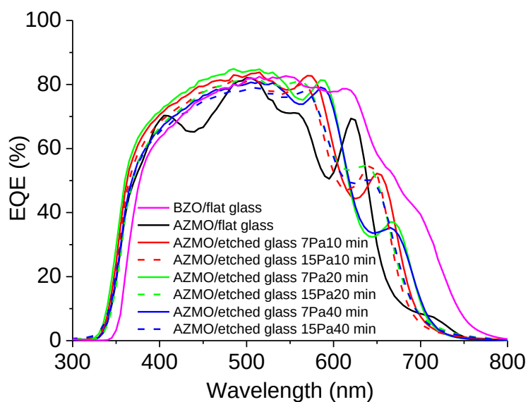
Fig. 5.19 EQE of a-Si solar cells deposited on BZO and AZMO/etched 7059 substrates.
