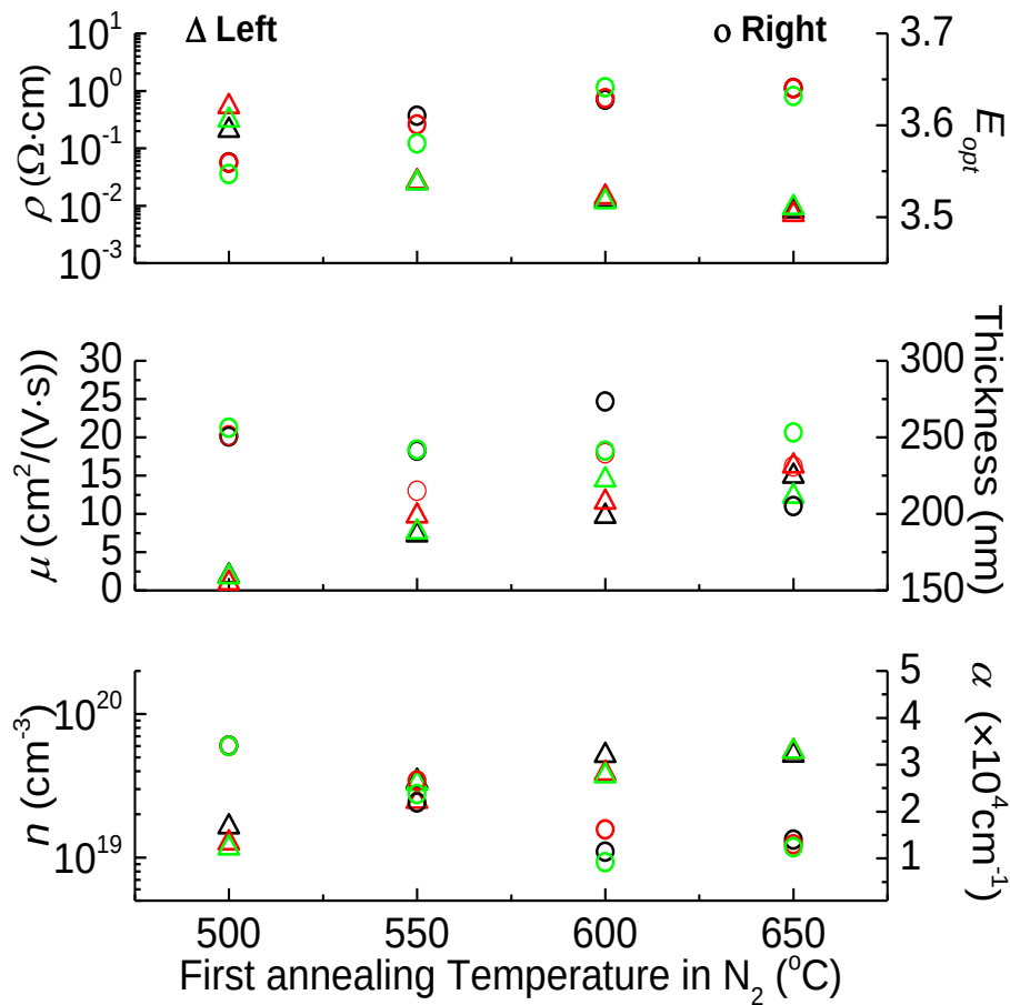
Fig. 3.45 Effect of annealing temperature on the electrical properties of AZMO thin film during the first annealing in \text{N}_2 . The absorption coefficient refers to the value at 350 nm.
