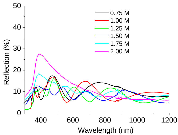
Fig. 3.13 Effect of \text{Zn}^{2+} solute concentration (in 2-M) on the reflection of AZMO thin film.
