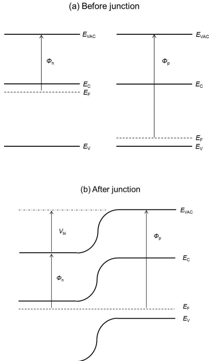
Fig. 1.6: Band profile of (a) before and (b) after p-n junction in equilibrium.
