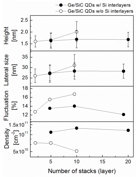
Fig. 5.13: Structural parameters as a function of number of stacks for Ge/Si 0.9995 C 0.0005 QDs (open circle) and Ge/Si 0.9995 C 0.0005 QDs with 2 nm-thick Si interlayers (closed circle).
