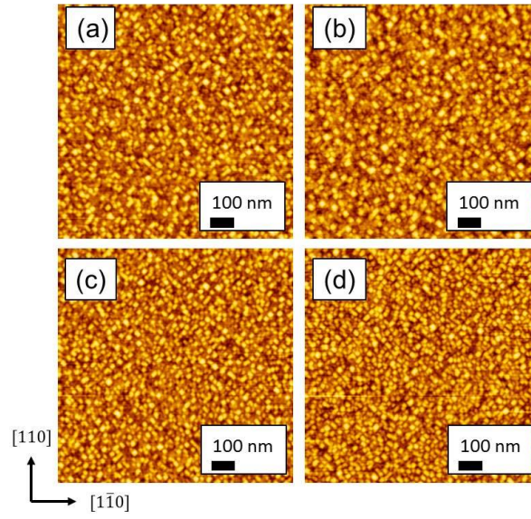
Fig. 5.12: 1 \times 1 \mu\text{m}^2 AFM images of topmost surface for (a) 5-layer and (b) 10-layer-stacked Ge/Si 0.9995 C 0.0005 QDs and for (a) 5-layer and (b) 10-layer-stacked Ge/Si 0.9995 C 0.0005 QDs with 2 nm-thick Si interlayers, respectively.
