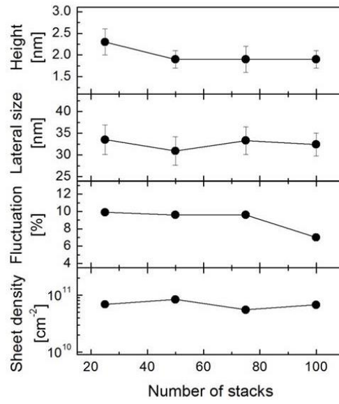
Fig. 4.6: Structural parameters of multi-stacked Ge/Si QDs as a function of number of stacks.
