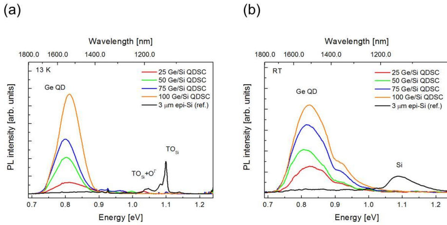
Fig. 6.7: PL spectra for the multi-stacked Ge/Si QDSCs measured at (a) 12 K and (b) room temperature (RT).
