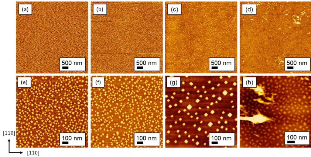
Fig. 4.11: 5 \times 5 \mu\text{m}^2 and 1 \times 1 \mu\text{m}^2 AFM images of topmost surface for 20-layer-stacked Ge/Si QDs with d_{\text{SL}} = (a) and (e) 40, (b) and (f) 20, (c) and (g) 10, and (d) and (h) 6 nm, respectively.
