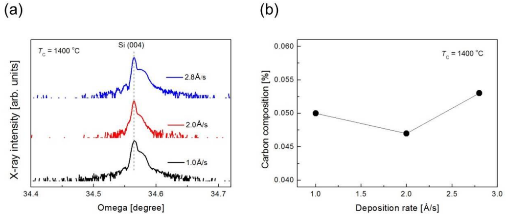
Fig. 5.8: (a) \omega - 2\theta scans for \text{Si}_{1-x}\text{C}_x layers grown on Si(001) substrates at C-cell temperature of 1400 °C and (b) its C concentration.
