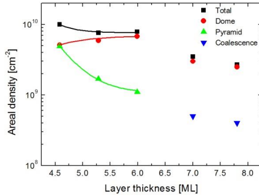
Fig. 3.6: Dependence of areal density for different shape Ge QDs on layer thickness.
