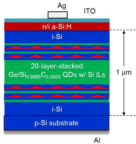
Fig. 6.17: Schematic structure of 20-layer-stacked \text{Ge/Si}_{0.9995}\text{C}_{0.0005} QDSCs. The resistivity of p-Si substrate is 2\ \Omega\text{cm} .
