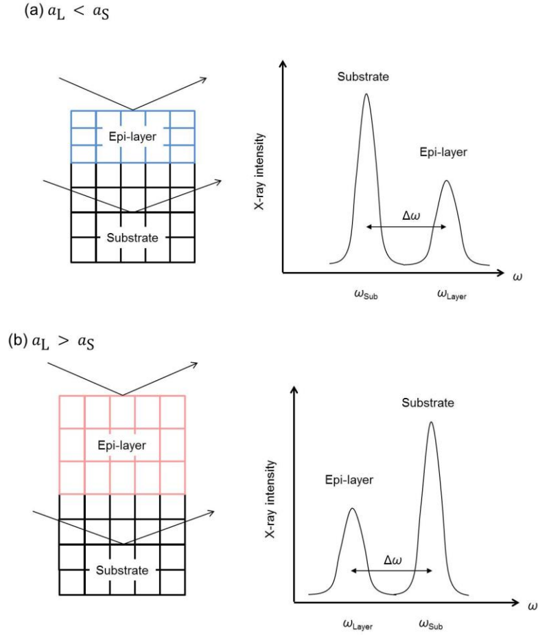
Figure 2.4: Schematic of \omega - 2\theta measurement in case of (a) a_L < a_S and (b) a_L > a_S .
