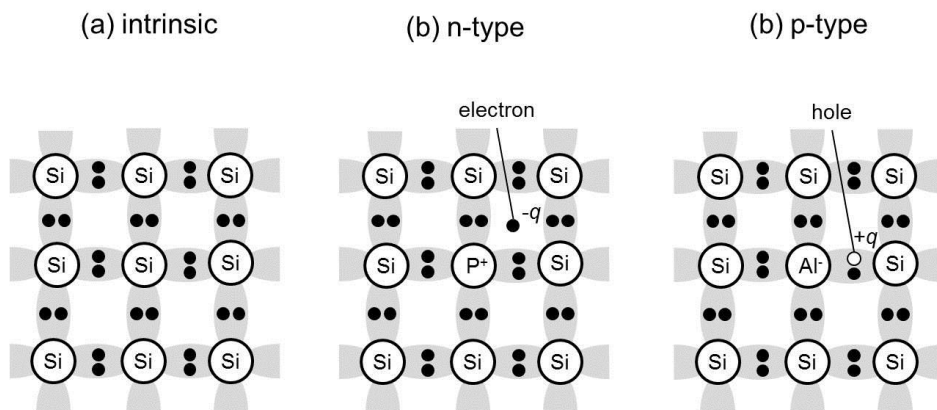
Fig. 1.4: Bond representations of (a) intrinsic, (b) n-type and (c) p-type semiconductors.
