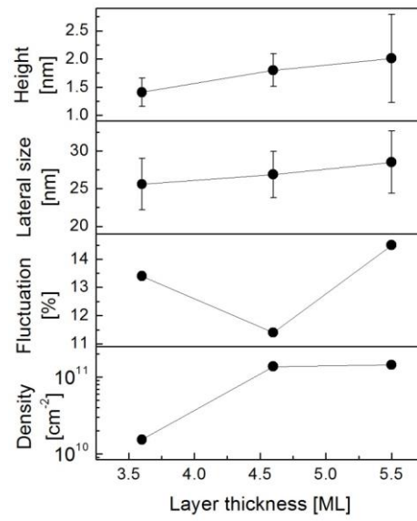
Fig. 5.11: Structural parameters of Ge/Si 0.9995 C 0.0005 QDs as a function of Ge layer thickness.
