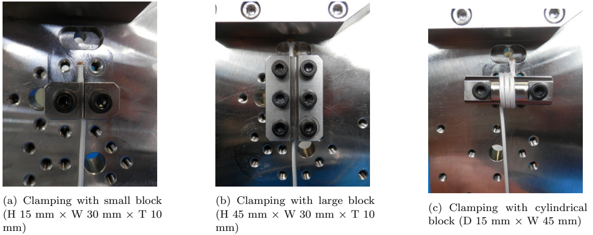
Figure 9. Clamping fixation types
