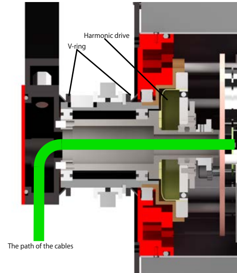
Figure 12. The end of the wheel
