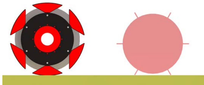
Figure 14. Comparison of swing-grouser and normal grouser on flat
