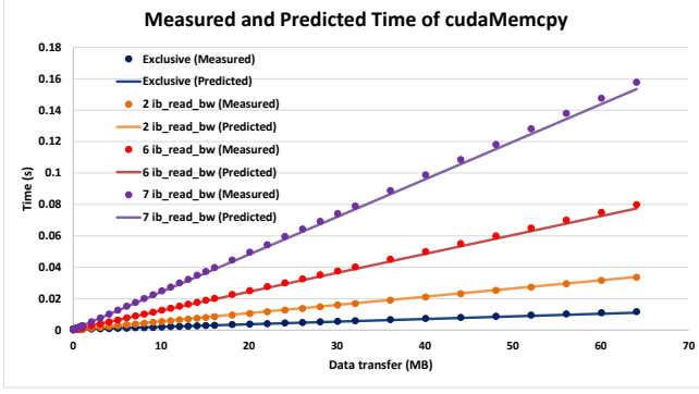
Figure 4. The effect of network contention on cudaMemcpy using rCUDA
