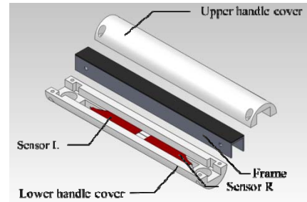
Fig.11 Configuraton of the handle; there are two pressure sensors which are able to detect the difference between right and left force signal when the user turns with twisting the handle.
