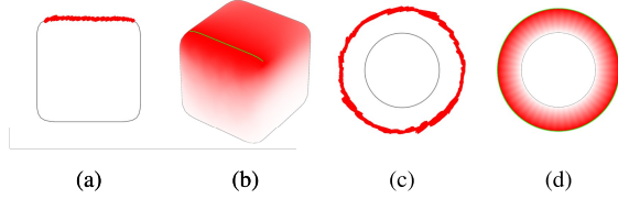
Figure 4: Generation of the influence area of a registered stroke.
