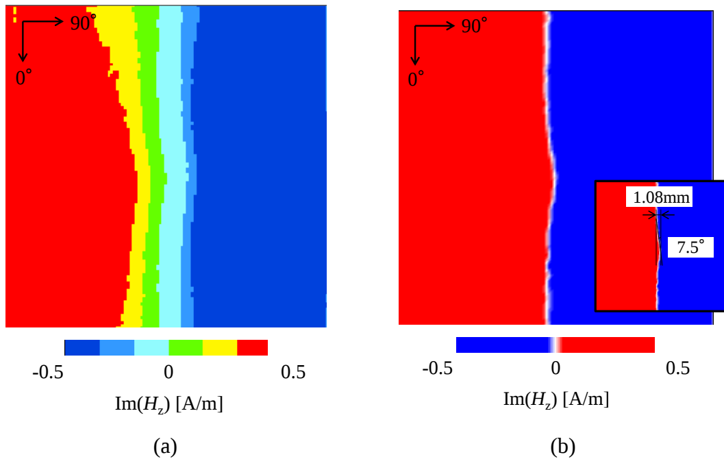
Fig. 4.15 \text{Im}(H_z) distribution obtained for a three-layer cross-ply specimen (specimen #1). A Tukey window was used before the inverse Fourier transform. The displayed area is a 30 mm \times 30 mm region in the surface waviness zone. (a) \text{Im}(H_z) distribution data. (b) The interpolated image with a highlighted \text{Im}(H_z) = 0 line. The lower right window shows auxiliary lines used for the estimation of the waviness size.
