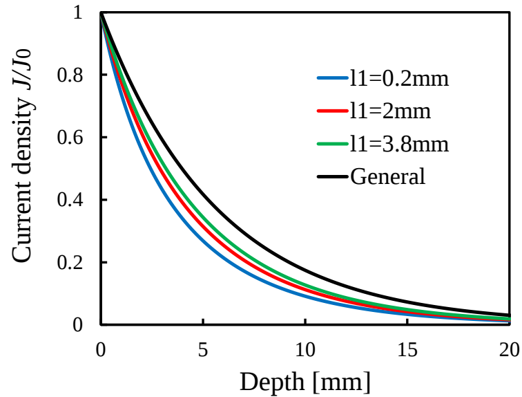
Fig. 2.9 Change in eddy current density at y = y_0 with lift-off l_1 of the drive current.
