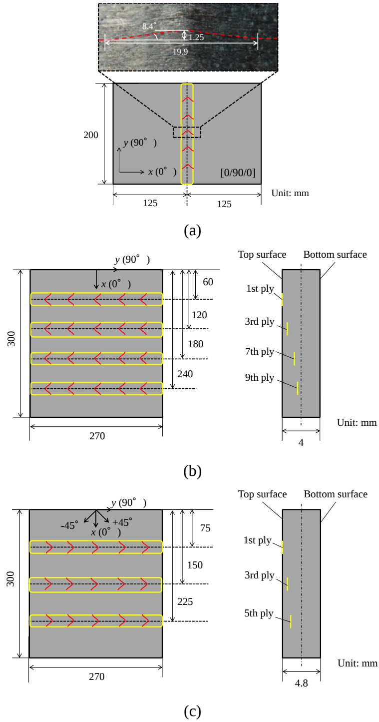
Fig. 4.10 CFRP specimens with artificially induced in-plane waviness: (a) specimen #1, a three-layer cross-ply CFRP ( [0/90/0] ) with surface in-plane waviness, (b) specimen #2, a 20-layer cross-ply CFRP ( [(0/90)_5]_s ) with in-plane waviness in the first, third, seventh and ninth layers from the top surface, (c) specimen #3, a 24-layer CFRP including \pm 45^\circ layers ( [(0/45/0/-45/0/90)_2]_s ) with in-plane waviness induced in the first, third and fifth 0^\circ layers from the top surface.
