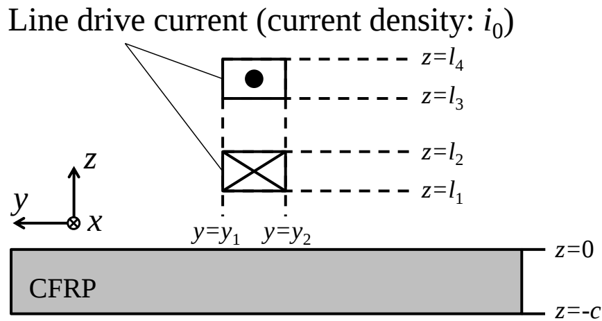
Fig. 4.2 Analytical model of line drive currents placed above CFRP directed in opposite directions to each other.
