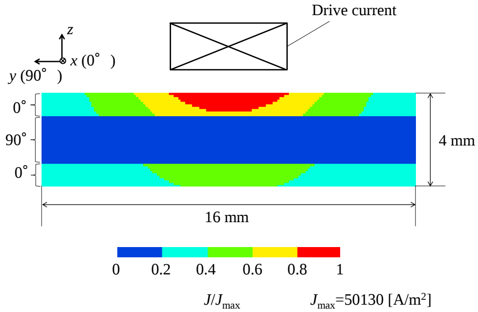
Fig. 2.6 Distribution of eddy current in the x direction when a line drive current is placed above cross-ply CFRP with the stacking sequence of [0/90/0].
