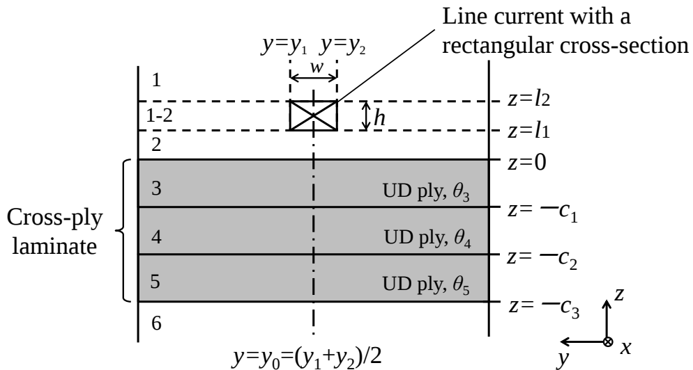
Fig. 2.5 Analytical model of a drive current with a rectangular cross-section placed above a cross-ply CFRP laminate.
