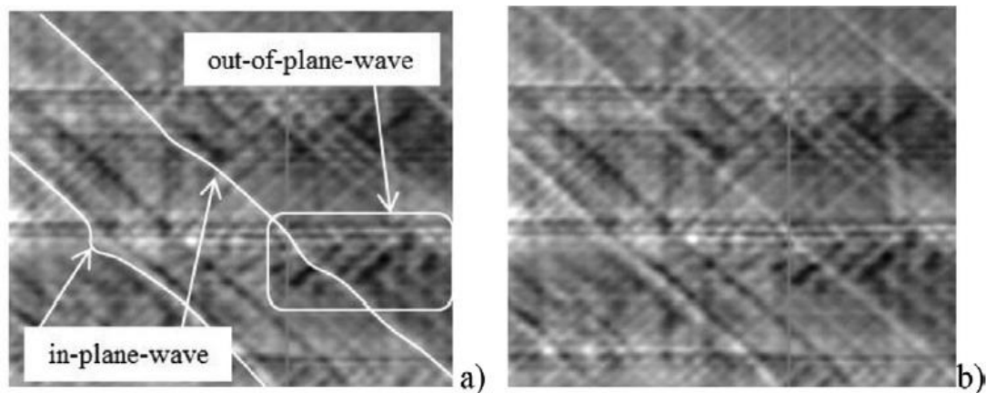
Fig. 1.10 High-frequency eddy current images of CFRP plates with in-plane and out-of-plane waves. (Size 150 mm × 150 mm × 5 mm): a) indication of the wave position, b) raw data image [1.59].
