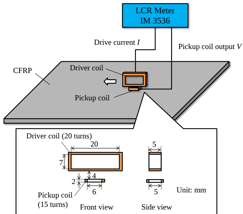
Fig. 3.30 Experimental setup for the inspection of specimen #3. The LCR meter supplies the drive current and measures the pickup coil voltage.
