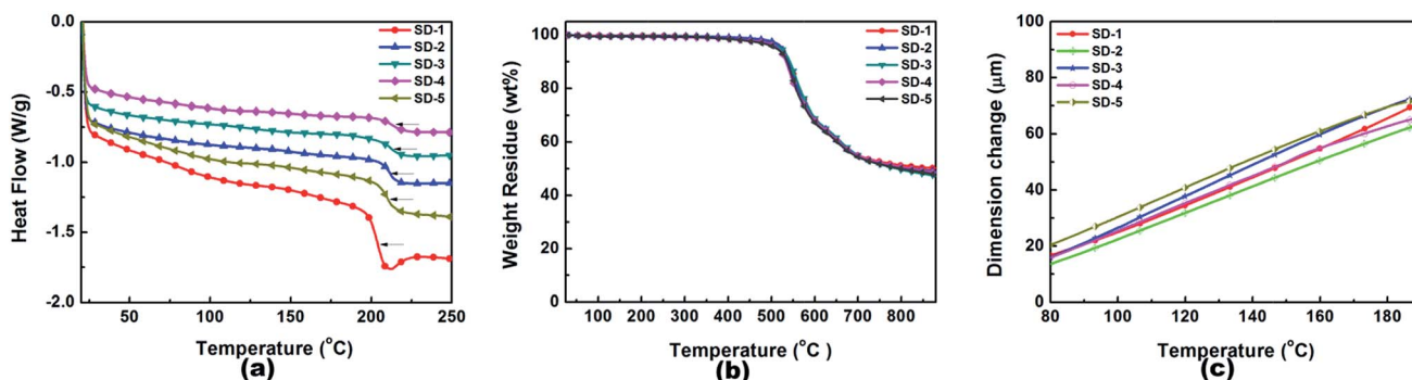
Fig. 6 DSC (a), TGA (b) and CTE (c) spectra of the linear binary composite (SD-1, PI (Si) -SiO 2 -20%) 32 and the hybrid ternary composites (SD-2 to SD-5, PI (Si) -HBPI (Si) -10%-40%-SiO 2 -20%).
