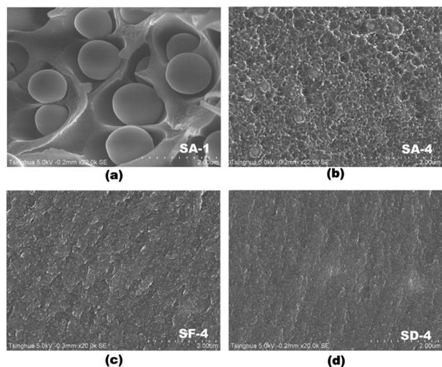
Fig. 3 Typical SEM images of PI and the composites. (a) SA-1 (PI 6 FDA-APB-SiO 2 -20%), 30 (b) SA-4 (PI 6 FDA-APB-HBPIBPADA-TAP(OH)-30%-SiO 2 -20%), 30 (c) SF-4 (PI 6 FDA-APB(Si)-HBPIBPADA-TAP(OH)-30%-SiO 2 -20%), 32 and (d) SD-4 (PI 6 FDA-APB(Si)-HBPIBPADA-TAP(Si)-30%-SiO 2 -20%). Scale bar: 2 μm.
