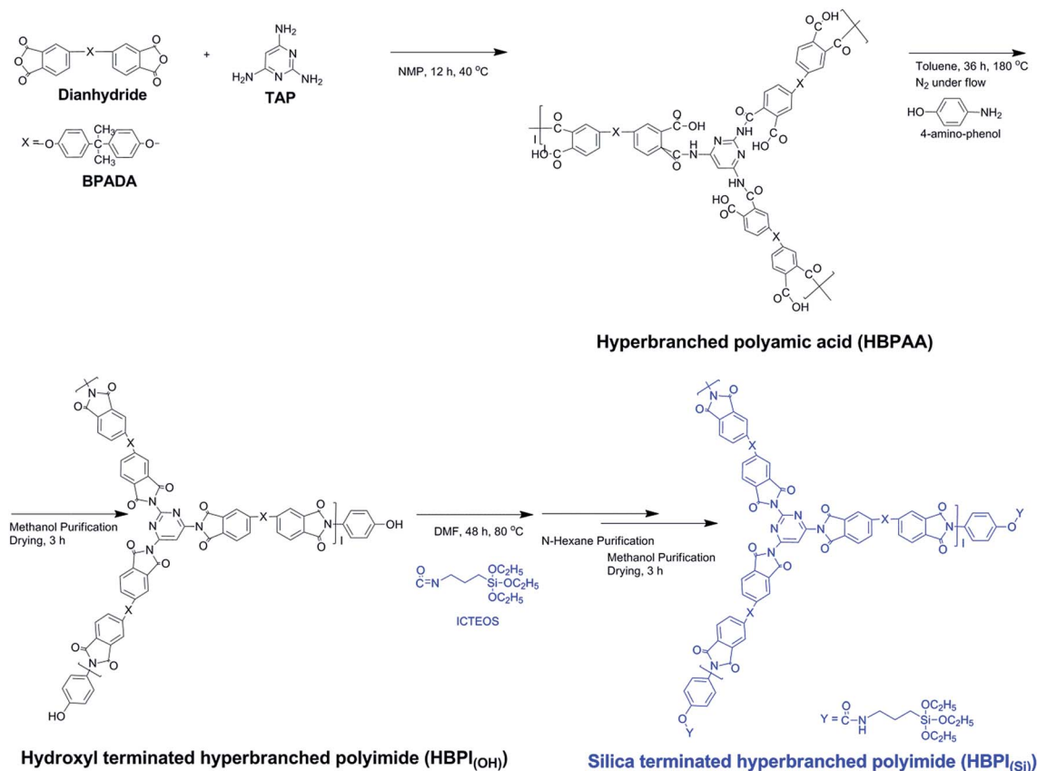
Scheme 1 Synthetic route for the PI 6FDA-APB(Si) -HBPI BPADA-TAP(Si) -SiO 2 hybrid ternary composite film.
