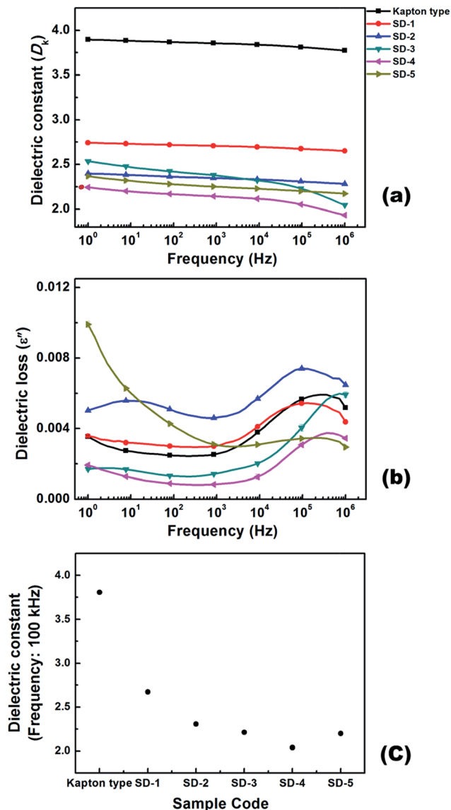
Fig. 4 Dielectric constants ( D_k ) of linear binary composite (SD-1, PI (Si) -SiO 2 -20%) 32 and hybrid ternary composites (SD-2 to SD-5, PI (Si) -HBPI (Si) -10%-40%-SiO 2 -20%) (a) from 10 6 to 1 Hz, (c) at 100 kHz, and (b) dielectric loss ( \varepsilon'' ) from 10 6 to 1 Hz.
