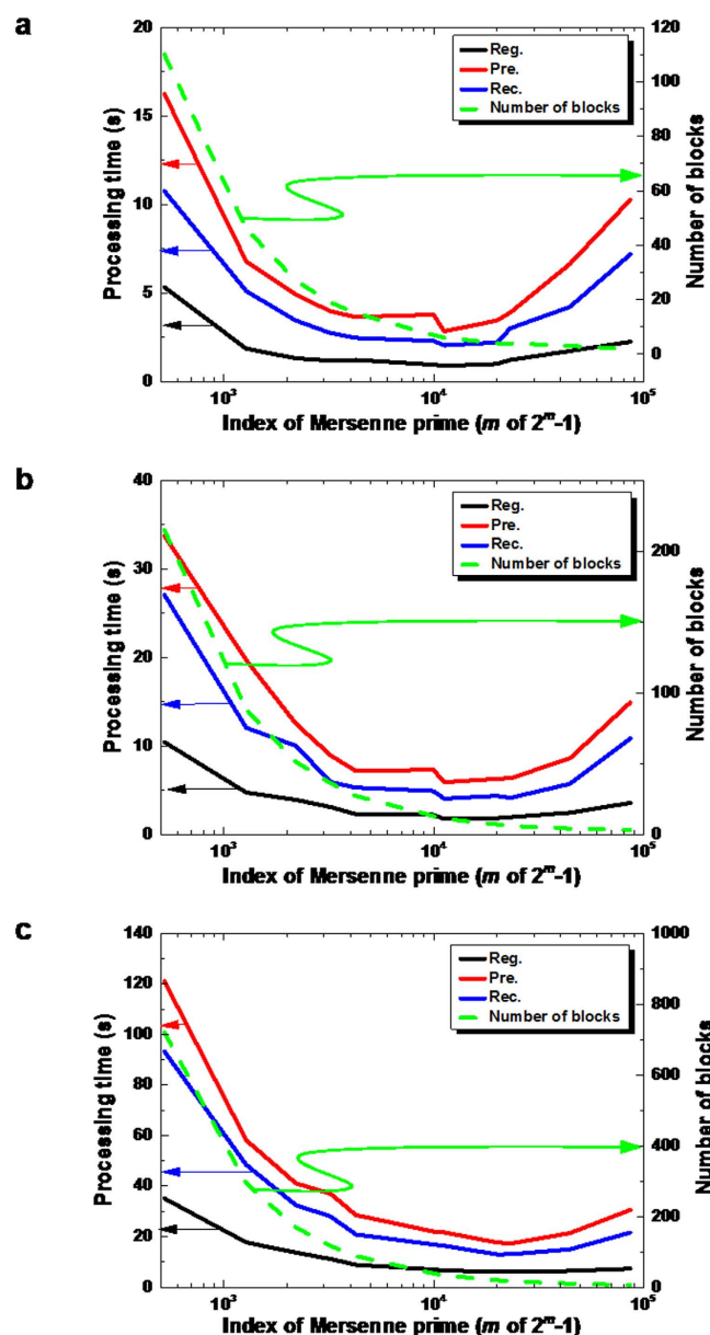
Figure 3. Processing time as a function of index of Mersenne prime for each phase. Reg Registration phase (black). Pre: Pre-computation and communications phase (red). Rec: Data reconstruction phase (blue). Dependence of numbers of divided blocks on Mersenne prime size is shown by green dashed line. The sizes of secret data are, (a) 6955 bytes, (b) 13695 bytes, and (c) 46000 bytes respectively.
