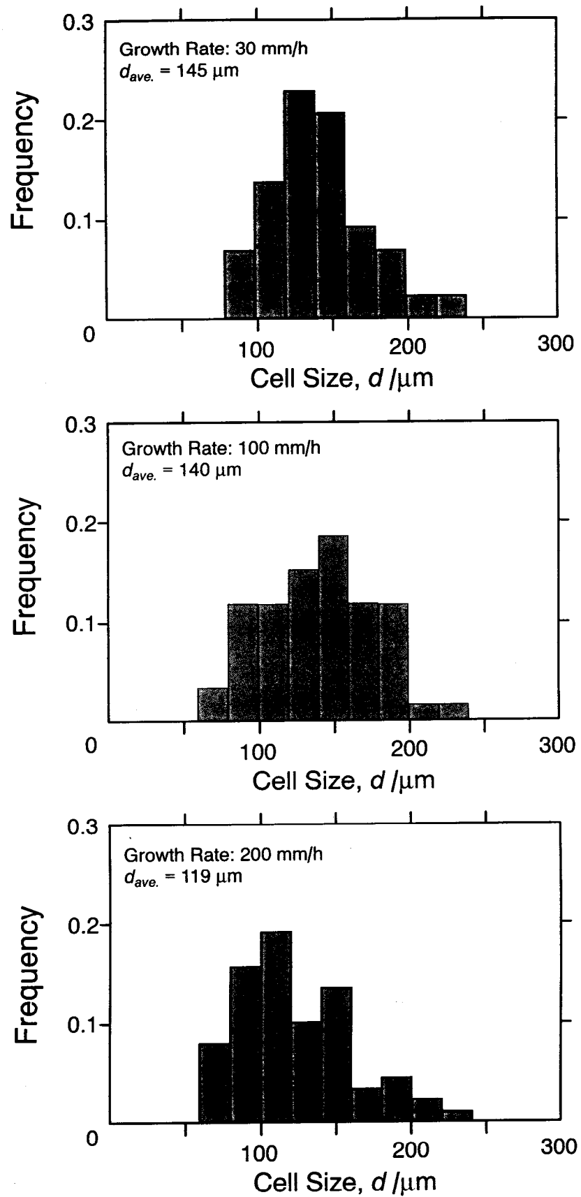
Fig. 5-13 Distribution of cell size measured in the Nb-17.5Si binary alloy comparing the growth rate; R = 30, 100, and 200 \text{ mm/h} .
