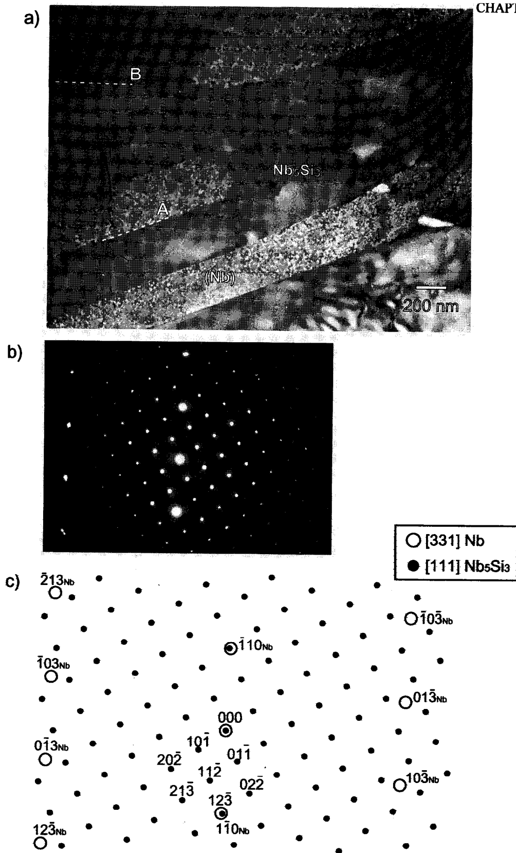
Fig. 2-9 TEM micrographs for the (Nb)/Nb 5 Si 3 lamellar microstructure in Nb-20Si-10Ti alloy; a) BF, b) SAD pattern, and c) its indexing.
