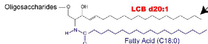
Figure 3-1: Structure of GM1a.
