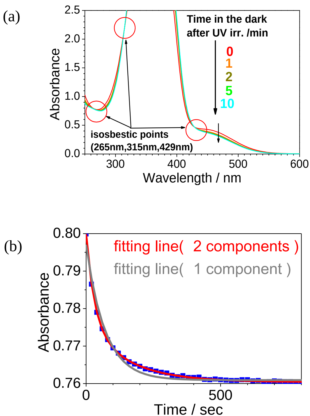
Figure 7-1. (a) Absorption spectra of neat [2PA-Hmim] \text{Tf}_2\text{N} during thermal isomerization after UV irradiation stopped. (b) The measured change in absorbance during thermal isomerization, and their fitting curves by single exponential and biexponential decay functions.
