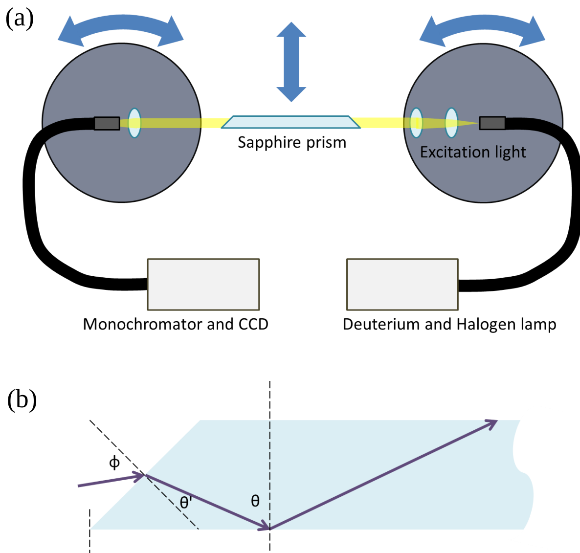
Figure 7-3. (a) Experimental apparatus for ATR-UV/Vis absorption spectroscopy, and (b) View of incident light and sapphire prism.
