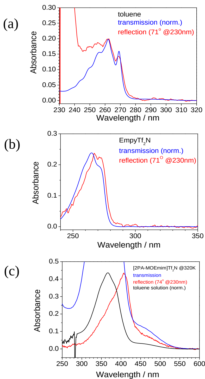
Figure 7-5. Absorption spectra of neat liquids by using reflection method (red), transmission method (blue), and that of toluene solution by using transmission method (black) as (a) toluene, (b) EmptyTf 2 N, and (c) [2PA-MOEmim]Tf 2 N.
