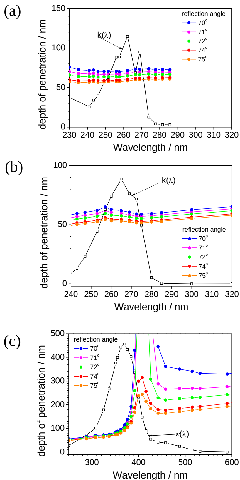
Figure 7-7. Theoretically estimated depth of penetration ( d_p ) depending on reflection angle comparing with band shape of \kappa for (a) toluene, (b) EmPyTf 2 N, and (c) [2PA-MOEmim]Tf 2 N.
