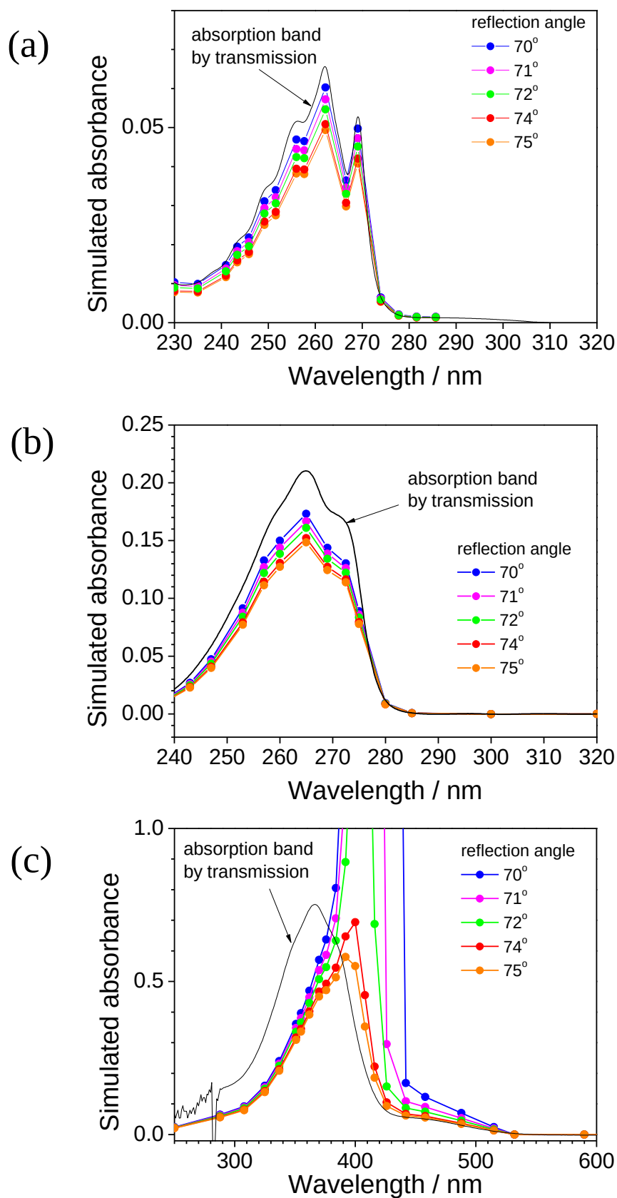
Figure 7-8. Calculated absorption band for various reflection angle and observed one by transmission method. (a) toluene (z=4), (b) EmptyTf 2 N (z=2), and (c) [2PA-MOEmim]Tf 2 N (z=1).
