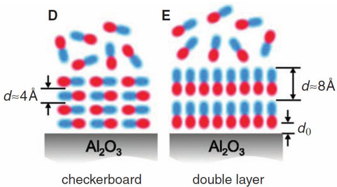
Figure 1-2. Sketch for the 1,1-butylmethylpyrrolidinium tris(pentafluoroethyl)trifluorophosphate- \text{Al}_2\text{O}_3 interface.
