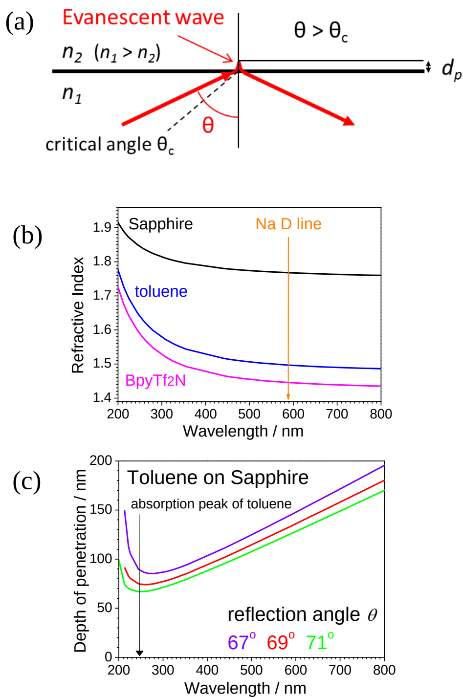
Figure 7-4. (a) Principle of evanescent wave generation, (b) estimated wavelength dispersion of refractive indices, and (c) estimated depth of penetration ( d_p ) depending on light wavelength in the case of toluene on sapphire.
