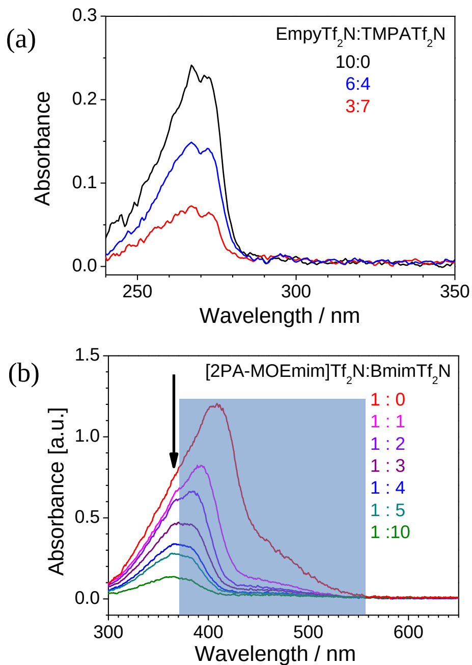
Figure 7-10. Absorption spectra by ATR method for various concentration of (a) EmpyTf 2 N in EmpyTf 2 N/TMPATf 2 N mixture, and (b) [2PA-MOEmim]Tf 2 N in [2PA-MOEmim]Tf 2 N/BmimTf 2 N mixture. The numbers in vertical axis of (b) are arbitrary units due to various number of reflections for each samples.
