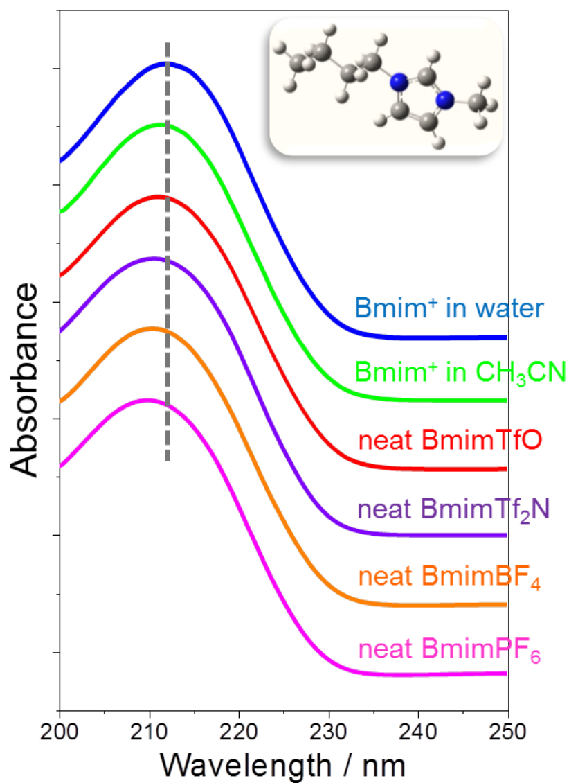
Figure 4-1. Normalized absorption spectra of \text{Bmim}^+ in two polar solvents and four neat RTILs. Inset is a structure of \text{Bmim}^+ calculated by DFT method: blue atom is for nitrogen, dark grey for carbon and light grey for hydrogen.
