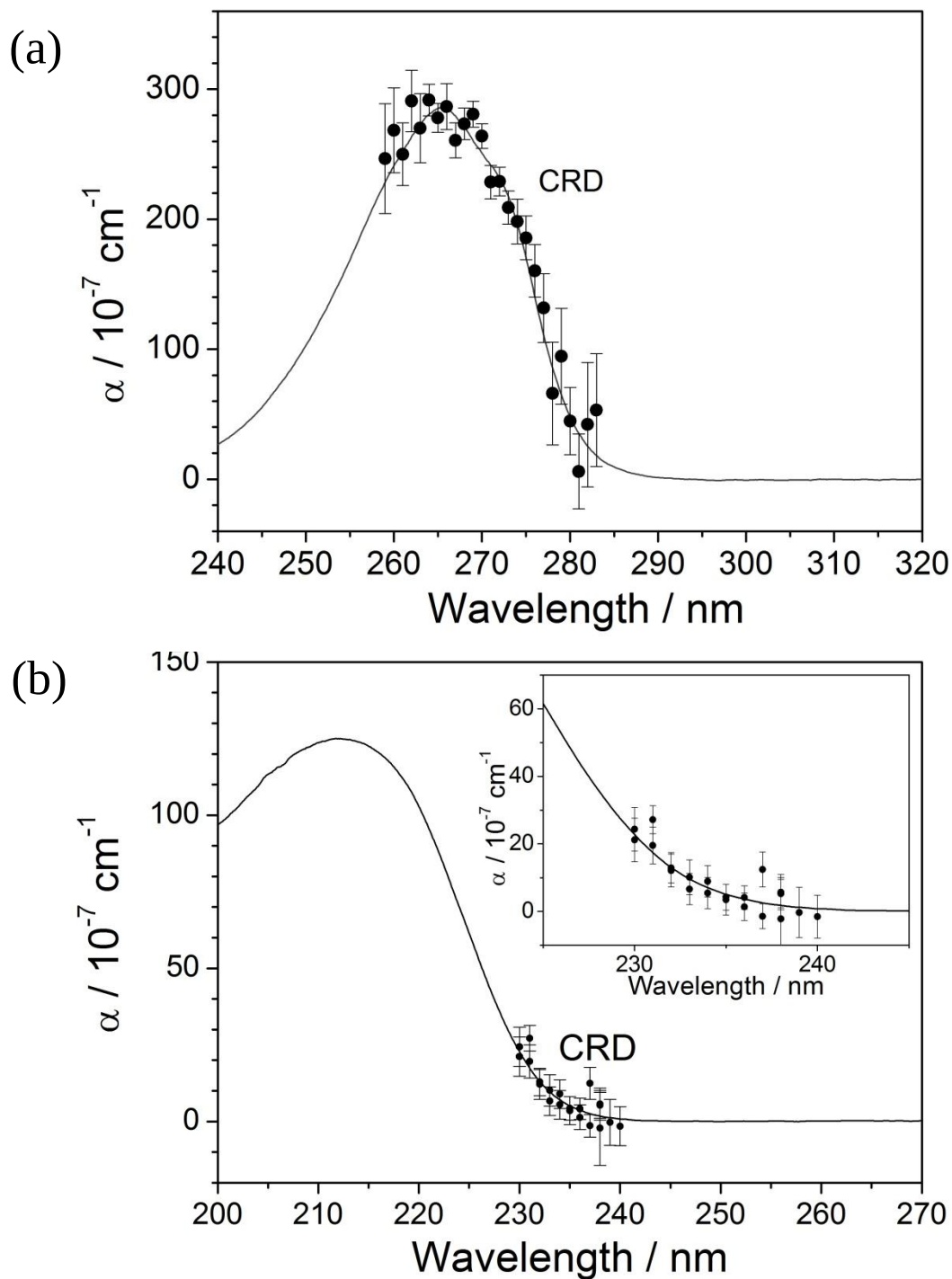
Figure 3-3. Absorption spectra (closed circles) of vaporized (a) EmPyTf 2 N at 453 K and (b) BmimTf 2 N in red edge of the band at 443 K measured by CRDS. The solid lines are single-path absorption spectra (in arbitrary units) of neat liquids at almost the same temperature as in the gas phase.
