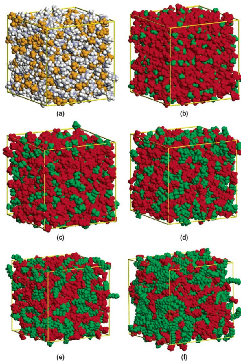
Figure 1-1. Snapshots of simulation boxes containing 700 ions of C_n\text{mimPF}_6 . The application of a coloring code enables clear identification of the charged (red) and nonpolar (green) domains that form in ionic liquids. The lengths of the box sides are given: (a) n=2 , CPK coloring; (b) n=2 , same configuration as in a with red/green (charged/nonpolar) coloring; (c) n=4 , l = 49.8 \text{ \AA} ; (d) n=6 , l = 52.8 \text{ \AA} ; (e) n=8 , l = 54.8 \text{ \AA} ; (f) n=12 , l = 59.1 \text{ \AA} . Graph from Lopes et al. , J. Phys. Chem. B , 110 , 3330 (2006) ( ref.[9] ).
