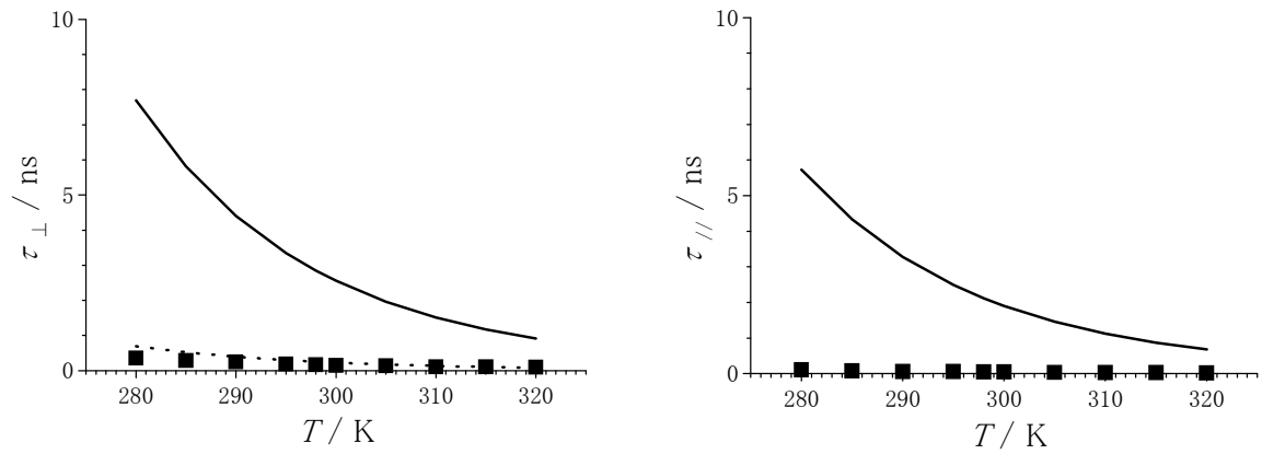
(c) BmimBF 4
