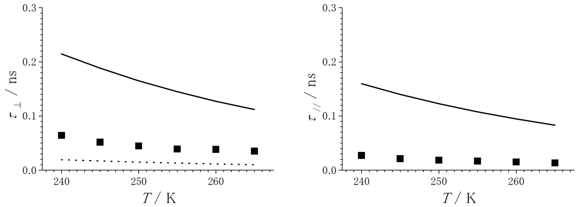
(c) BmimBF 4
