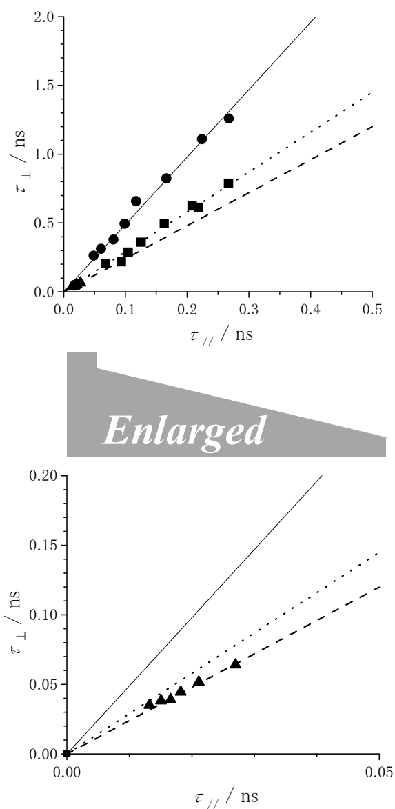
Figure 4.4: Relation plots of \tau_{\perp} vs. \tau_{\parallel} values of PADS radical measured in three solvents. The solvents were BmimCH 3 OSO 3 (■), DemeTf 2 N (●) and N -methylimidazole (▲). Solid, dotted and dashed lines were obtained by least-squares fittings with N values of 4.9, 2.9 and 2.4, respectively.
