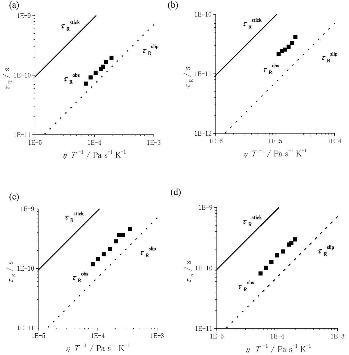
Figure 4.6: Logarithmic plots of measured \tau_R values (■) of PADS vs. \eta T^{-1} in (a) BmimTf 2 N, (b) N -methylimidazole, (c) DemeTf 2 N and (d) N 3111 Tf 2 N. Theoretical \tau_R values calculated under the stick and slip conditions are shown by solid and dotted lines, respectively (see text for the details).
