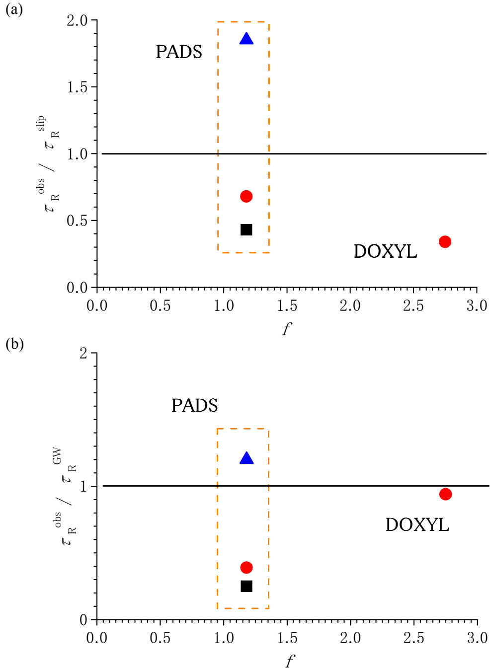
Figure 5.3: \tau_R^{obs} / \tau_R^{calc} vs f plots. The \tau_R^{calc} values were calculated by (a) hydrodynamic theory with slip boundary condition and (b) Gierer and Wirtz hydrodynamic theory. The solvents were BmimBF 4 (■), BmimPF 6 (●) and BmimTf 2 N (▲).
