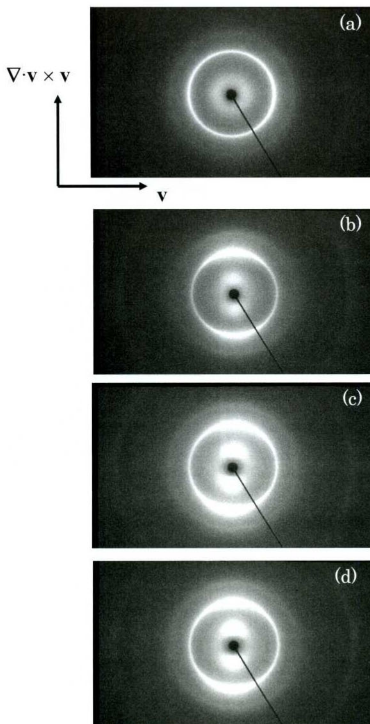
Figure 2-4. WAXD patterns of P-Std nematic film sheared by rotational rheometer in regions 0, I, II and III. X-ray beam was irradiated along the velocity gradient ( \nabla \mathbf{v} ) direction. The strong reflection in the central part has a spacing of 4.8 Å, which is attributed to the lateral packing of polymers.
