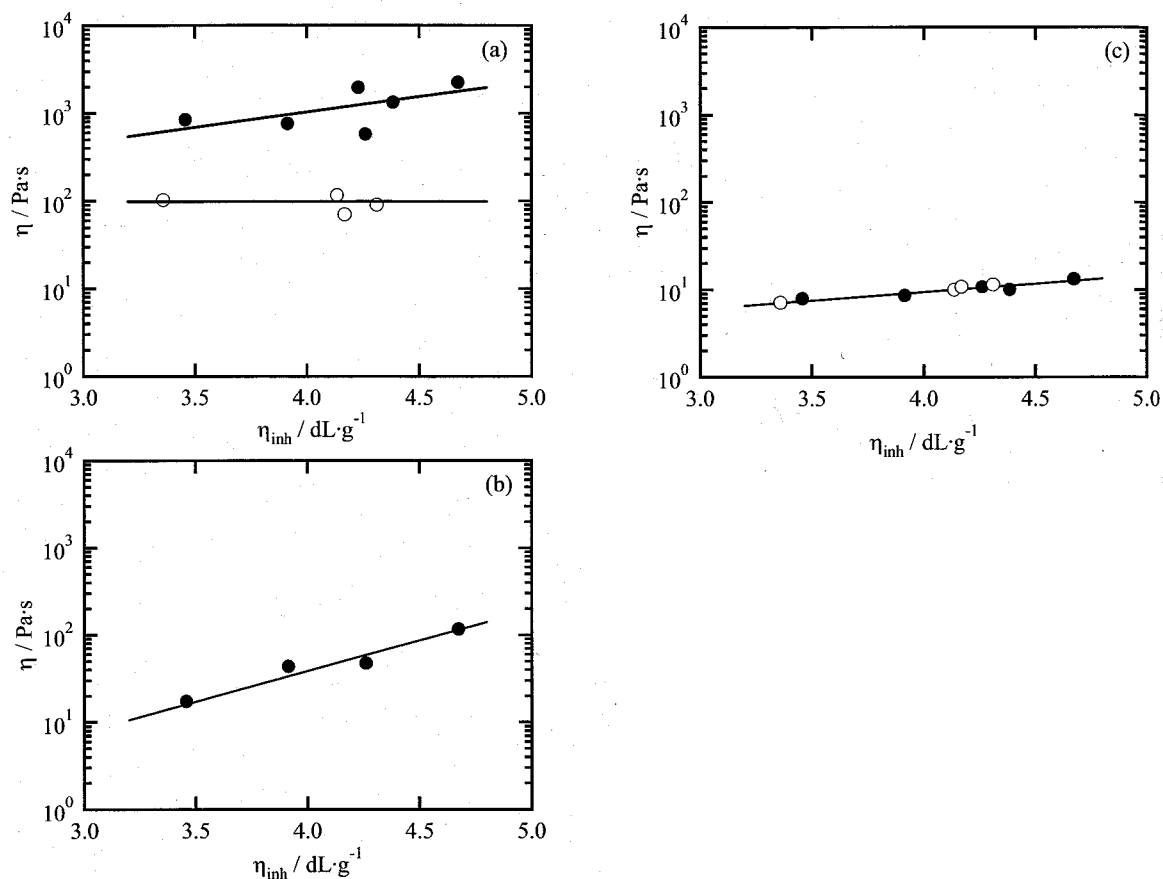
Figure 2-3. Variation of apparent viscosity (a) in the lowest-shear-rate Newtonian plateau (region 0), (b) in the high-shear-rate Newtonian plateau (region II), and (c) at a shear rate of 4864 s -1 in high-shear-rate shear-thinning region III with inherent viscosity of copolymers. The applied temperature is 330°C. The viscosities of the SHG-active and non-SHG-active polymers are plotted by closed and open symbols, respectively.
