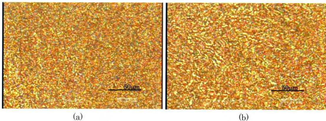
Figure 4-4. Optical microscopic nematic textures of (a) P-0.017 and (b) P-0.029 .
