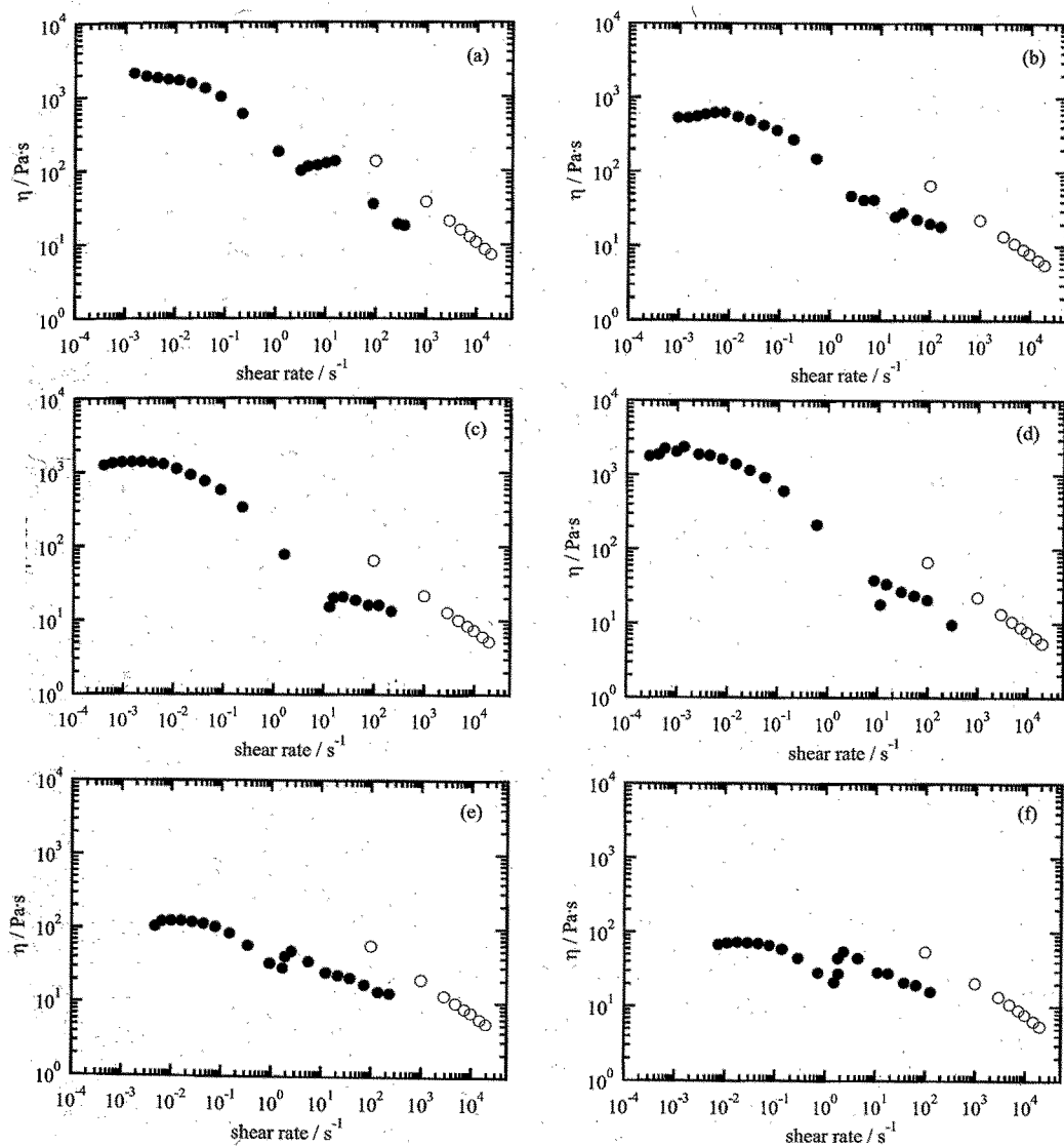
Figure 2-2. Steady-state viscosity for the nematic LCs of (a) P-Std, (b) P-0.015, (c) P-0.03, (d) P-0.05, (e) P-0.08, (f) P-0.09 at 330°C. The data presented by closed and open circles are collected by the plate-and-plate rheometer and the capillary rheometer, respectively.
