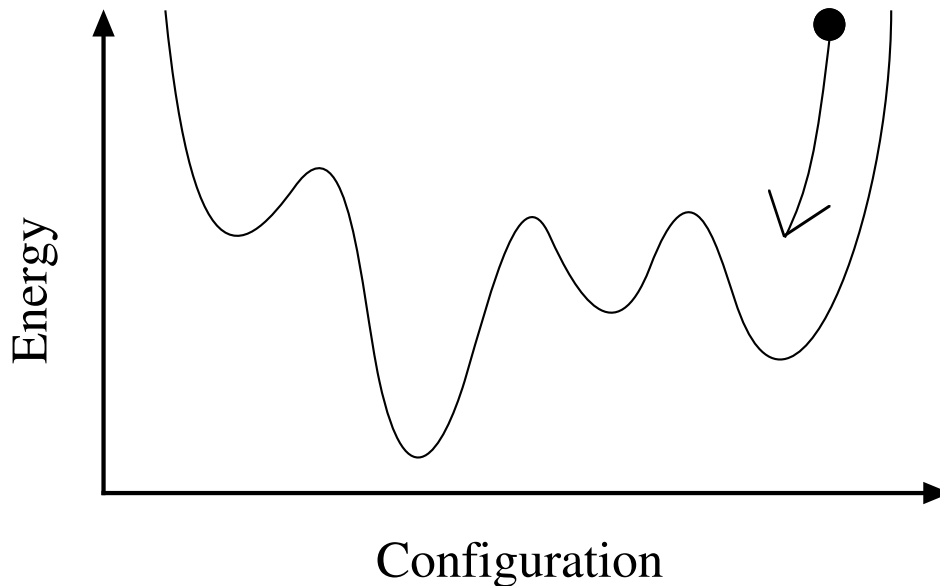
Figure 1.7: Cooling from high temperature to low temperature. If the cooling rate is too fast, the system may be trapped in a local minimum.
