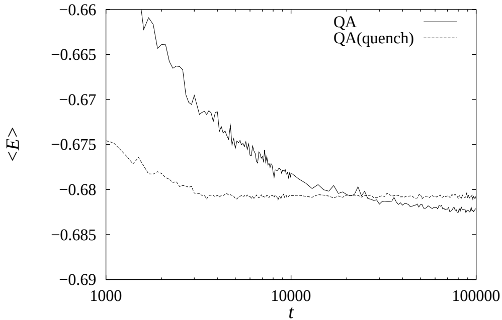
Figure 3.19: Solutions for annealing and quenching processes are plotted. The annealing schedule is T = \Gamma = 10/\sqrt{t} and the quenched value is T = \Gamma = 0.1/\sqrt{10} = 0.0316 \dots which is the final value of the schedule.
