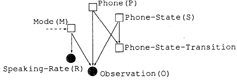
Figure 10.5: Hidden mode mixture weight model. The dotted link represents an edge from the previous time frame. (HM-MW)
