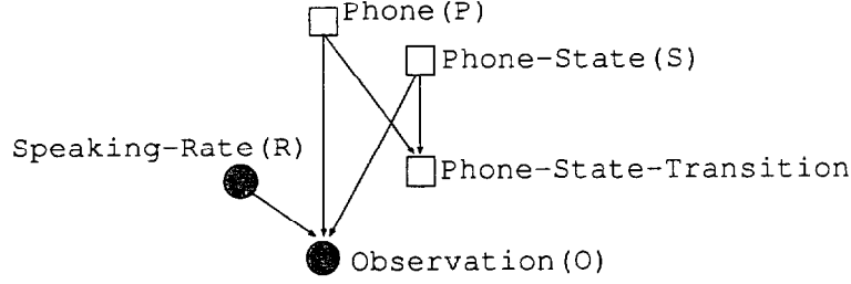
Figure 10.4: Regression model. (REG)
