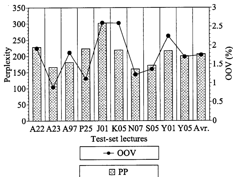
Figure 7.1: Test-set perplexity and OOV rate of the task.
