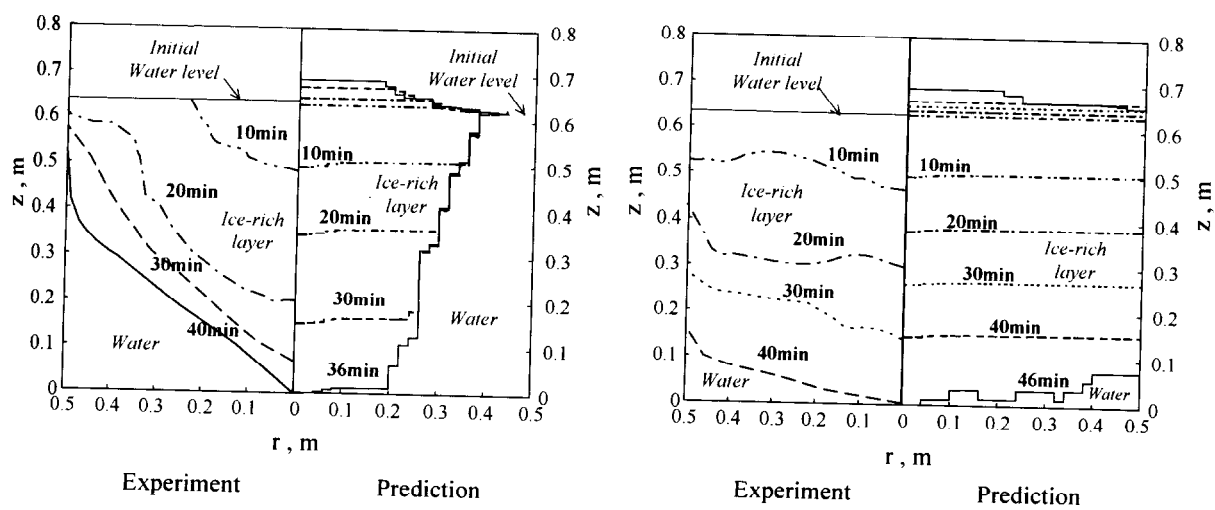
a) G = 0.33 \text{ kg/s} ( v_{\text{avg}} = 4.2 \times 10^{-4} \text{ m/s} ) (b) G = 0.92 \text{ kg/s} ( v_{\text{avg}} = 1.17 \times 10^{-3} \text{ m/s} )
