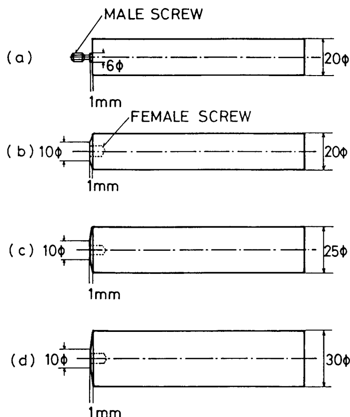
Fig.2-1 The types of wave-trapped horns used in the experiments of low amplitude operation.
