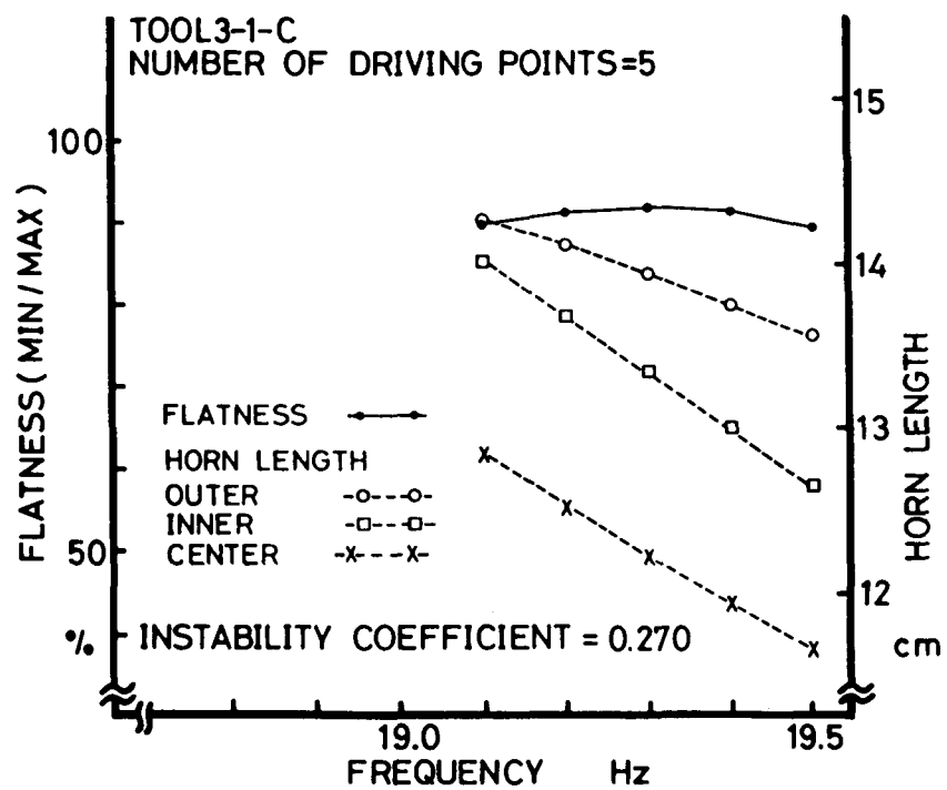
Fig.3-7 The plane configuration of a vibrating system and the evaluation of the instability coefficient for it.
