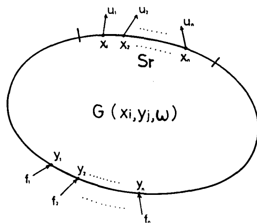
Fig.1-2 A schematic explanation of modal vibration control of elastic systems by superposition of Green's functions.
