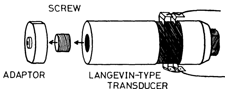
Fig.2-6 The Langevin-type transducer and the adaptor for resonance adjustment.
