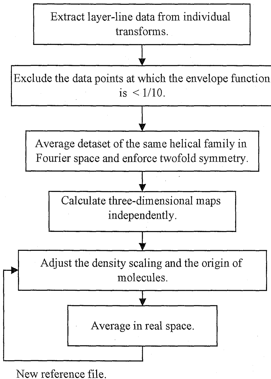
FIGURE II.1 Flow diagram of averaging of different images of tubular crystals.
