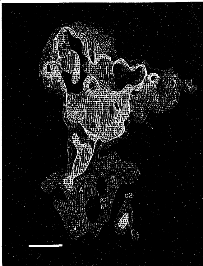
FIGURE III.8 (a) the structural model of a whole \text{Ca}^{2+} -ATPase molecule at better than 10 Å resolution. (b) a cut out model viewed in a direction similar to (a). The largest membrane segment A is marked; c1 and c2 identify two transmembrane columns. Red and white nets enclose 80% and 40% of the expected volume, respectively. Orange arrows indicate a mass (white nets) in the groove, which presumably represent the bound CrATP molecule. Bars represent 20 Å.
