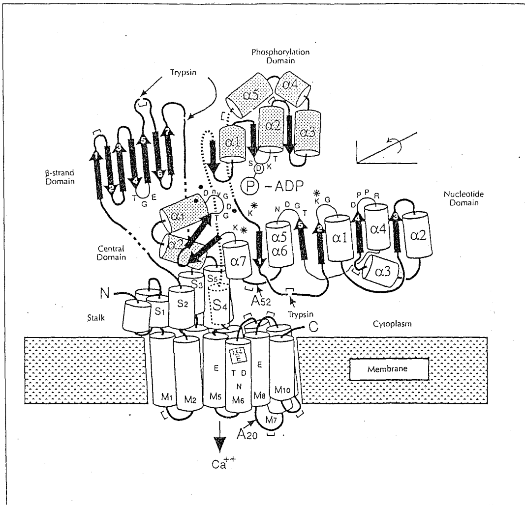
FIGURE I.2 Secondary structure prediction of \text{Ca}^{2+} -ATPase. Reprinted from Green and Stokes (1992).
