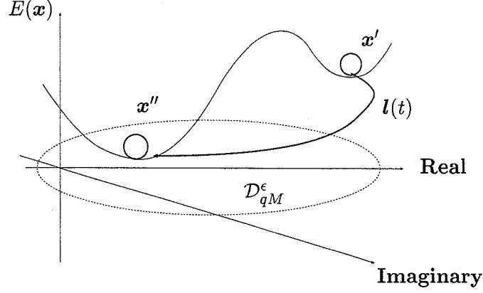
Figure 3.2: monotone path l(t)
