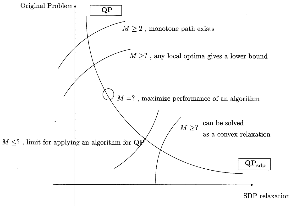
Figure 6.1: Open Problems
