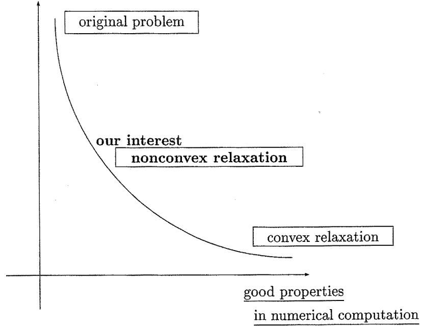
Figure 1.2: location of nonconvex relaxation problems
