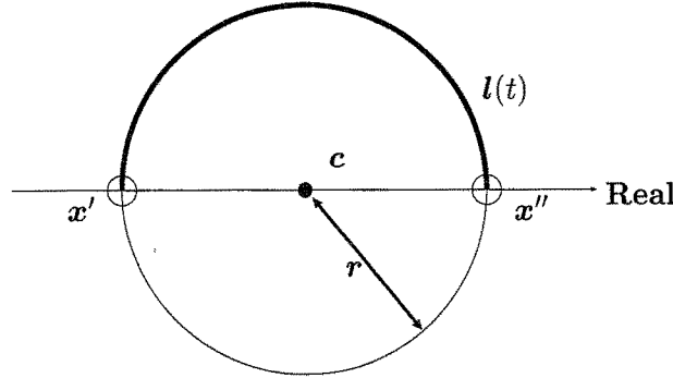
Figure 3.3: the monotone path defined by eq.(3.4)
