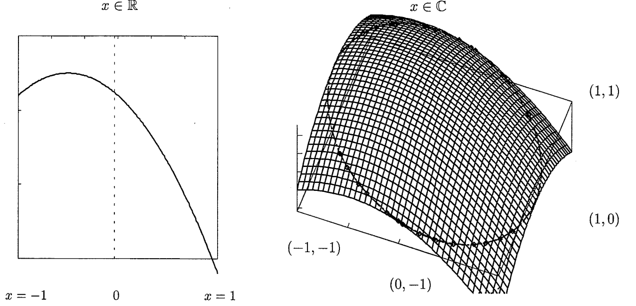
Figure 1.1: x \in \mathbb{R} (left) and x \in \mathbb{C} (right)
