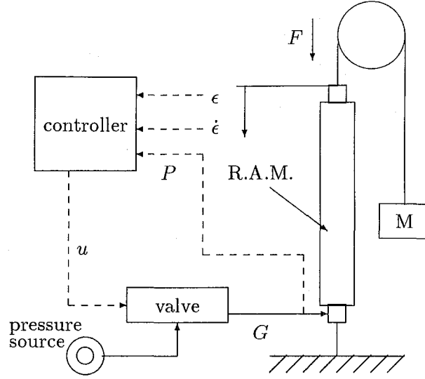
Figure 6.2.1: experimental apparatus
