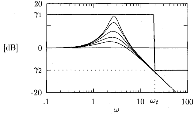
Figure 4.4.3: Gain plots of T(j\omega) for \alpha = 1, 2, 3, 4, 4.5 . ( \gamma_1 = -10[\text{dB}] , \gamma_2 = 15[\text{dB}] )
