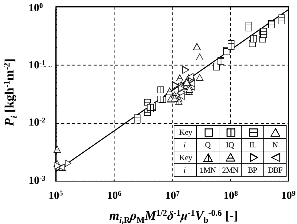
Fig. 4.7 Correlation between overall permeation coefficient and distribution coefficient
