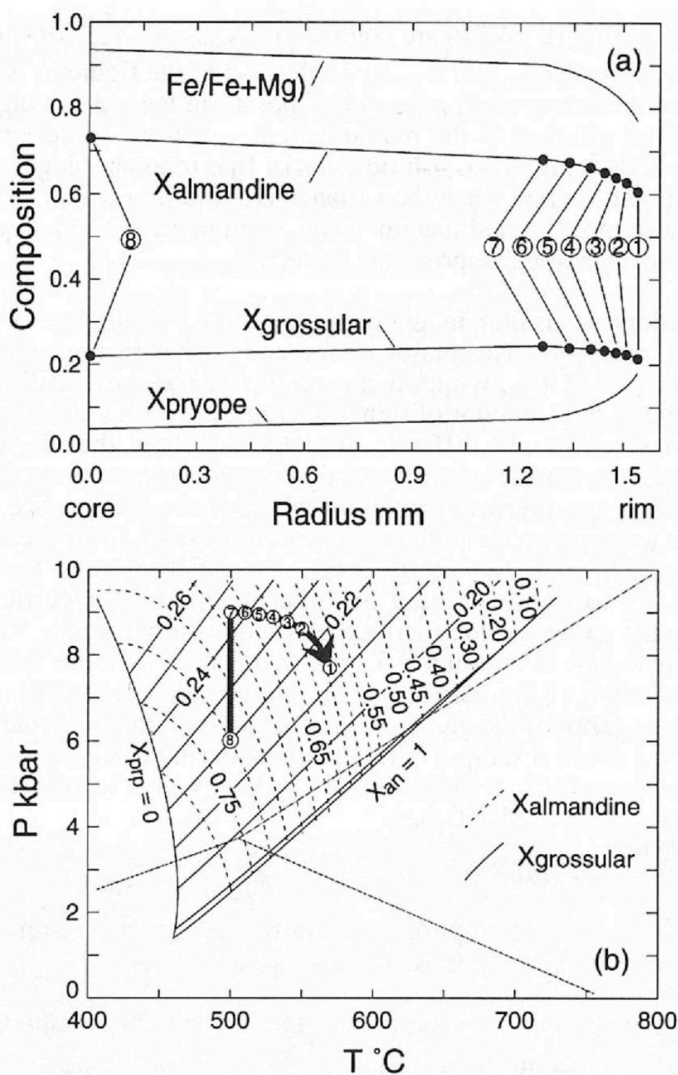
Fig. III-12 An example of P - T - t path estimation from compositionally zoned garnet (Spear, 1993). a) A hypothetical zoning profile of garnet. The numeros 1-8 correspond to those in (b). b) P - T - t path estimation by Gibb's method from the almandine and grossular zoning patterns of (a).
