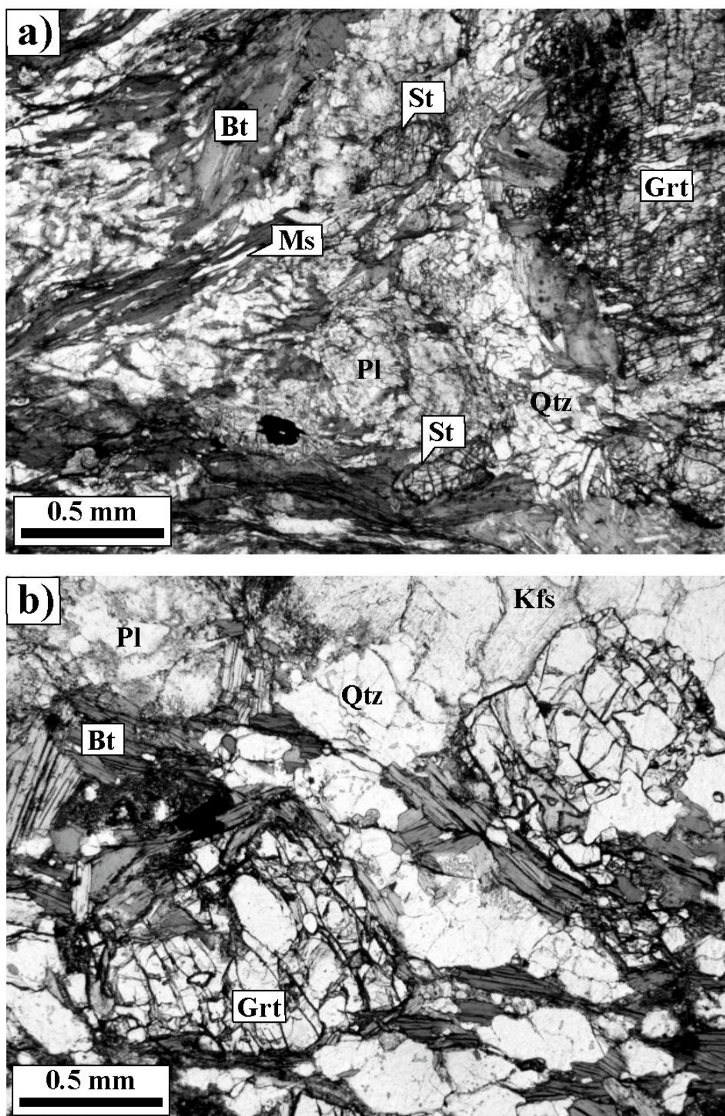
Fig. II-4 Photomicrographs showing the representative minerals and textures of metapelites. a) Grt-St-Bt schist, Chaglinka region; b) Migmatitic gneiss, Kumdy-Kol region. Plane-polarised light.
