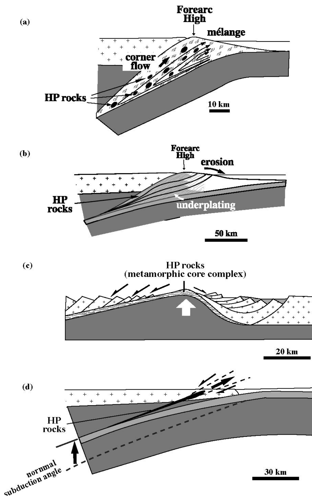
Fig. C-8 Representative exhumation tectonic models of high-P/T metamorphic belt. a) mélange model (simplified after Cloos, 1982), b) two-way-street model (simplified after Platt et al. , 1975), c) extension model (simplified after Lister & Davis, 1989), d) wedge extrusion model (simplified after Maruyama et al. , 1997). See main text for detailed explanation.
