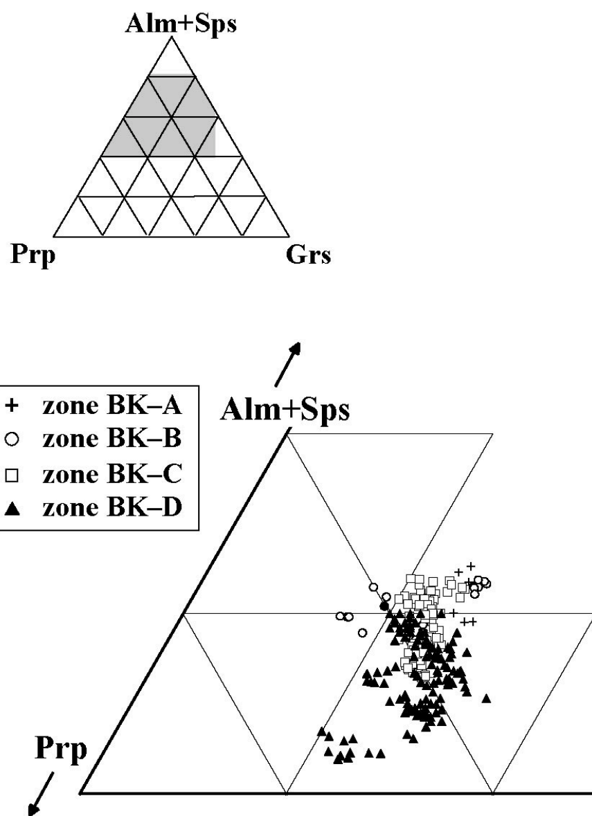
Fig. I-11 Compositions of analysed garnets from each zone of the Barchi-Kol region.
