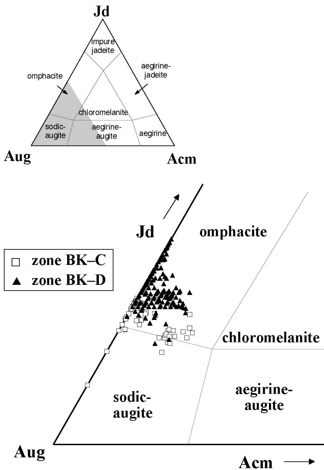
Fig. I-20 Compositions of analysed clinopyroxenes from each zone in the Barchi-Kol. Clinopyroxene nomenclature is after Essene & Fyfe (1967).
