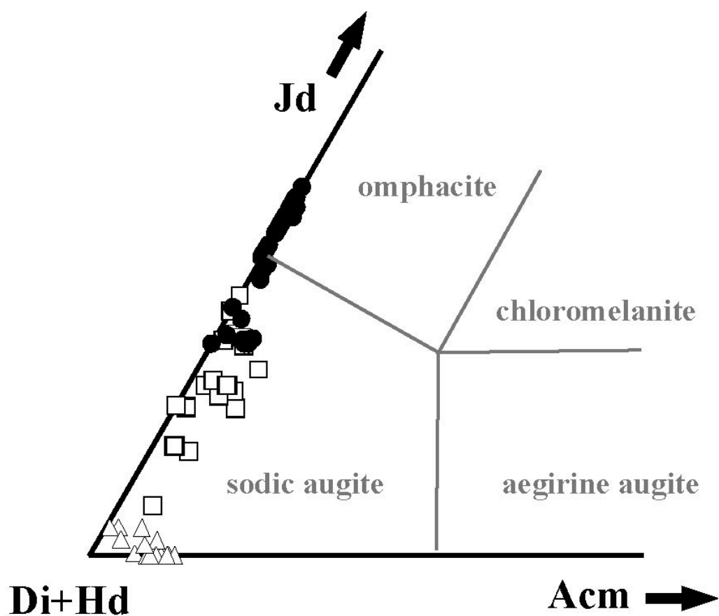
Fig. I-21 Clinopyroxene compositions of various zones and lithologies in the Borovoye region. Clinopyroxene nomenclature is followed after Esson & Fyfe (1967).
