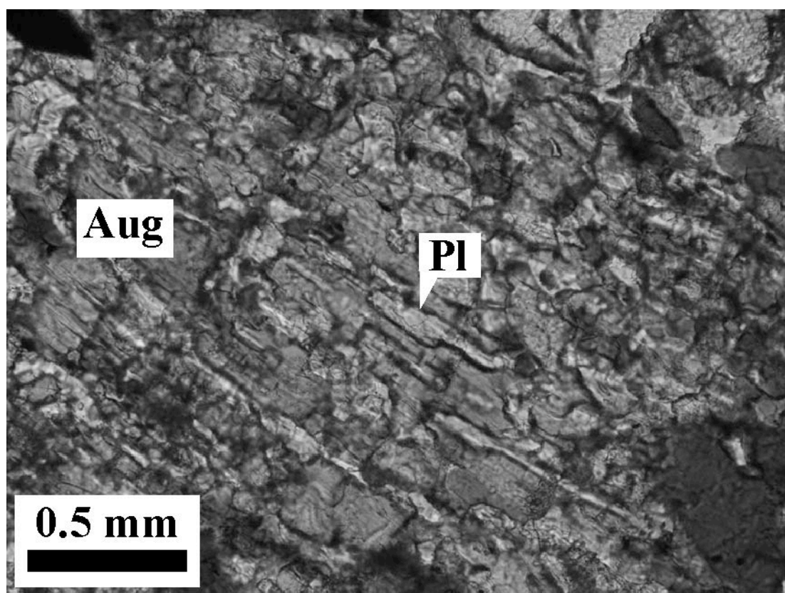
Fig. I-10 Plagioclase exsolution lamellae in augite in zone BV-D amphibolite in the Borovoye region. Exsolved plagioclase has topotaxial relationship with host augite. Plain polarised light .
