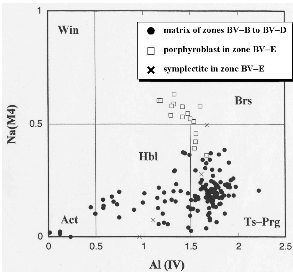
Fig. I-19 Amphibole compositions of various textures in the Borovoye metabasites.
