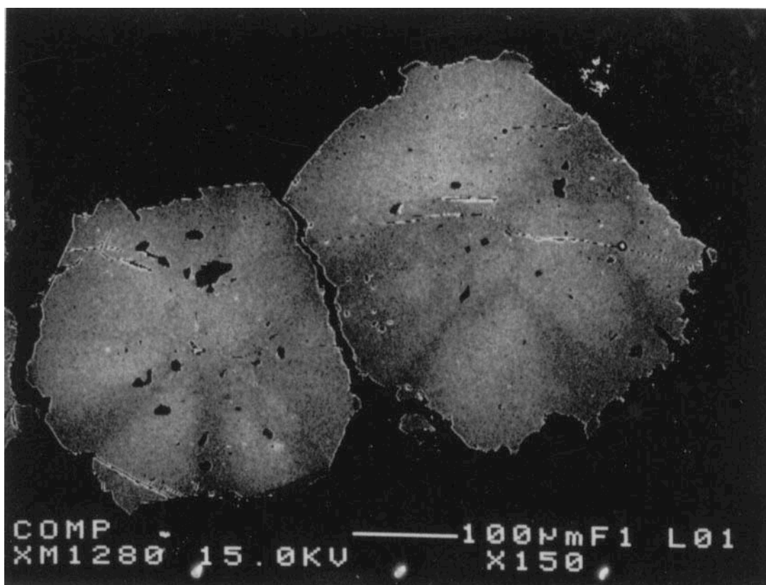
Fig. I-14 Back-scattered electron imagery of type II (sector-zoned) garnets observed in zone BK-B in the Barchi-Kol region.
