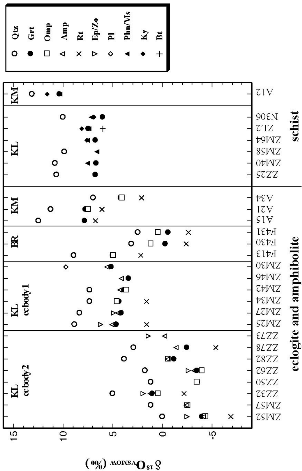
Fig B-2 δ¹⁸O values of eclogites, amphibolites and schists. KL: Kuleit; BR: Barchi-Kol; KM: Kundy-Kol.
