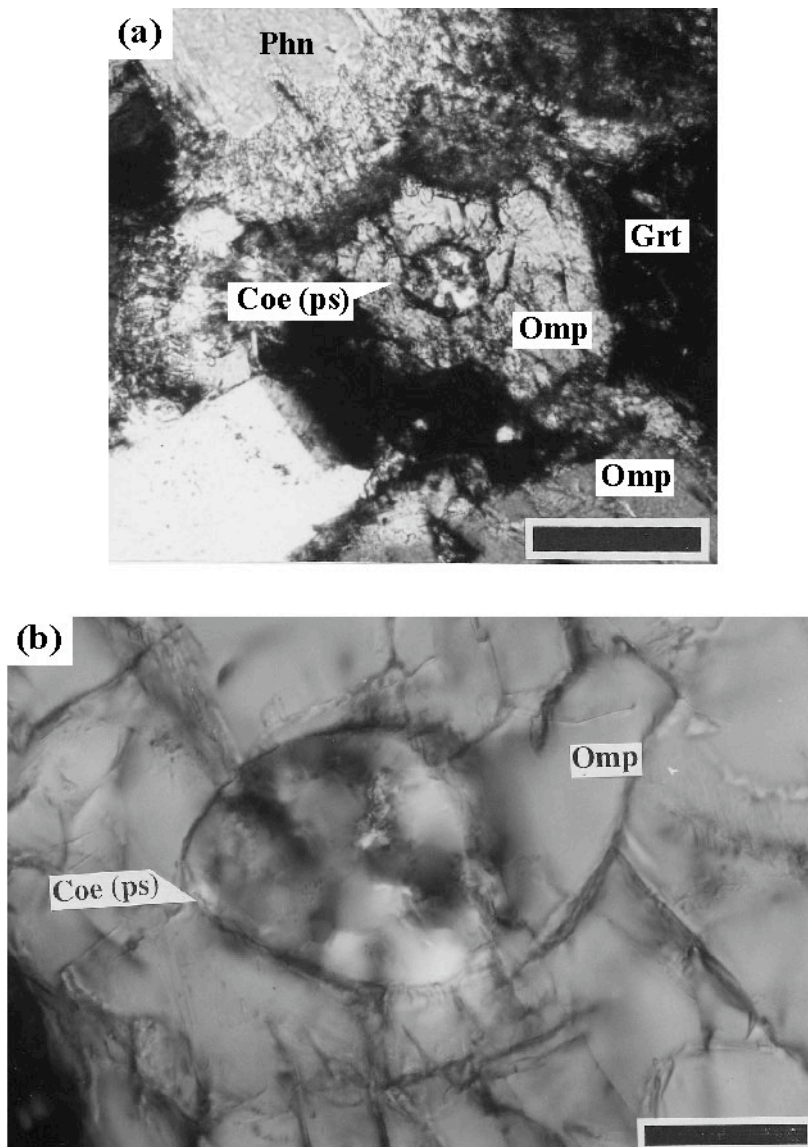
Fig. I-6 Photomicrographs showing polycrystalline quartz pseudomorph after coesite included in omphacite from phengite-bearing eclogite in the Barchi-Kol region. Scale bar indicates (a) 0.1 mm; (b) 0.02 mm. Crossed polarised light.
