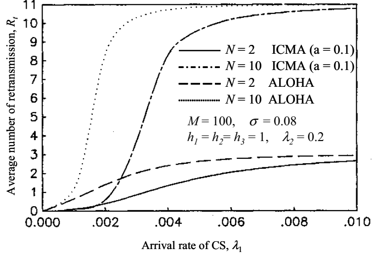
Figure 3.8: Average number of retransmission versus arrival rate of CS ( N = 2, 10 )
