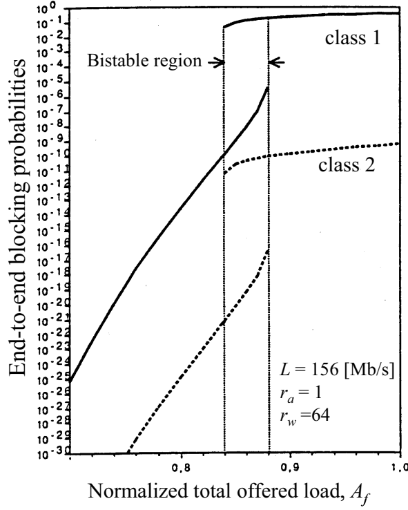
Figure 5.5: End-to-end blocking probabilities without controls
