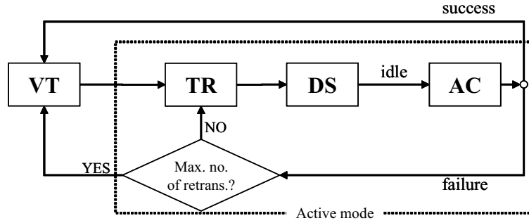
Figure 3.5: Modified state transition diagram of mobile terminal
