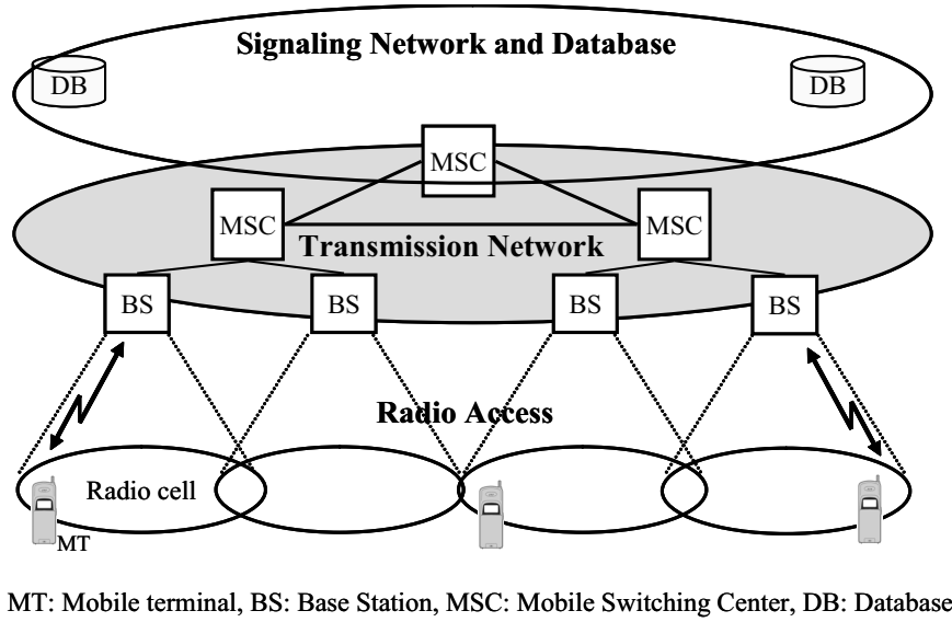
Figure 1.1: Cellular system architecture
