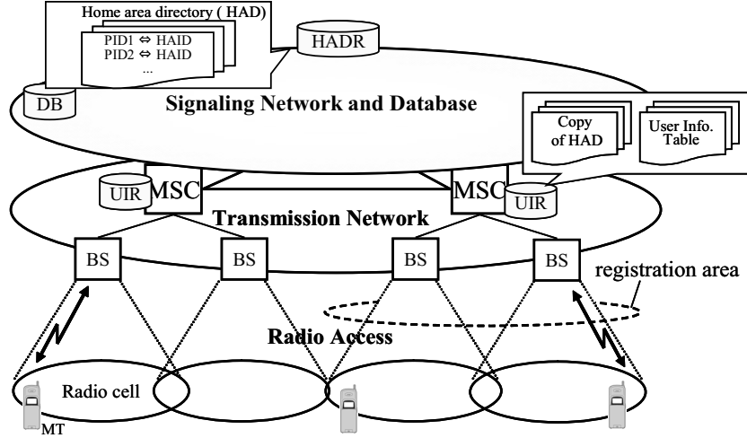
HADR: Home area directory register, HAID: Home area identification, UIR: User information register, MT: Mobile terminal, BS: Base Station, MSC: Mobile Switching Center, DB: Database
