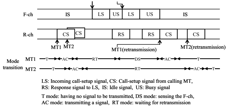
Figure 3.2: Control channel operations for ALOHA access scheme
