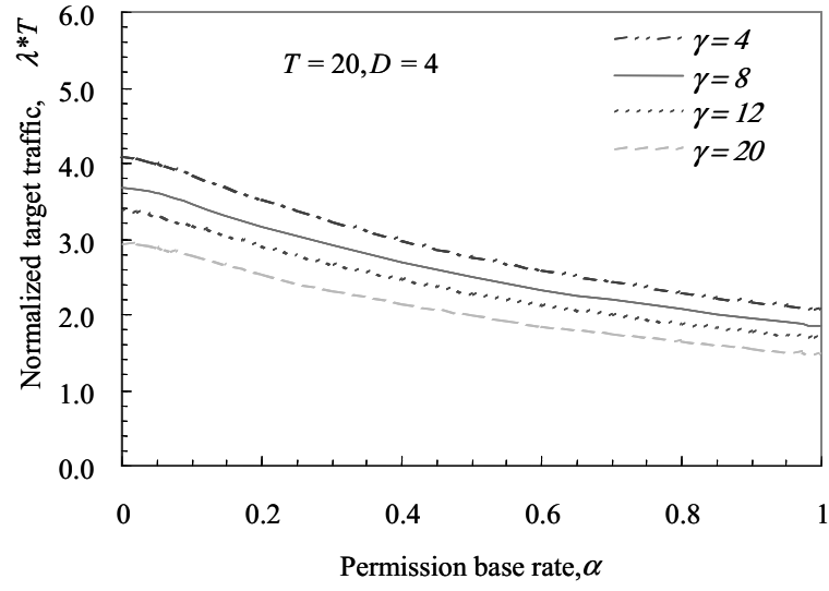
Figure 2.8: Target traffic for ICMA/CD
