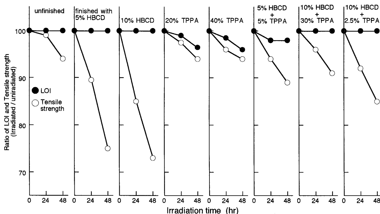
Fig. 3-42 Reduction ratio of LOI and tensile strength observed after ultraviolet irradiation.
