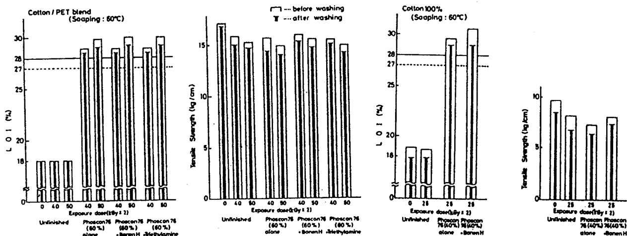
Fig. 3-58 Washability of C/P blend and Cotton fabrics treated with Phoscon 76 and cured by electron beam irradiation.
