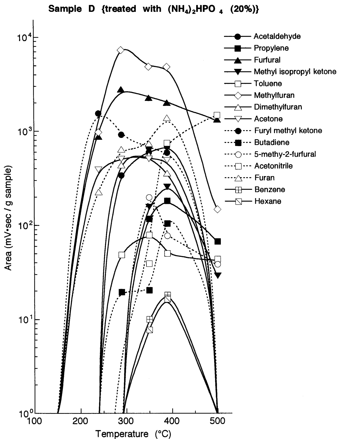
Fig. 6-42 Area vs temperature curves of all gas species from individual samples for comparison of pyrolytic gas generation behavior between flammable and flame retardant samples.
