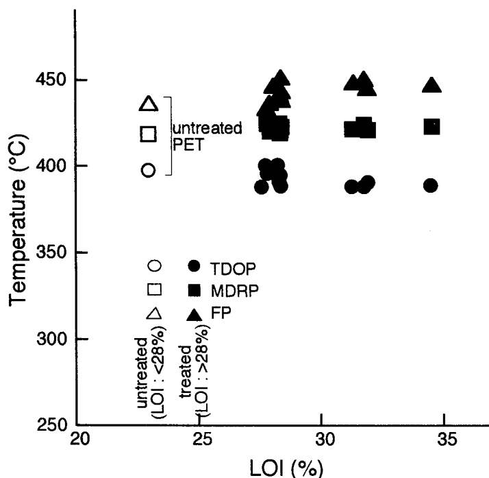
Fig. 6-35 LOI vs temperature plots of PET untreated (open marks) and treated (solid marks) samples at TDOP, MDRP and FP.
