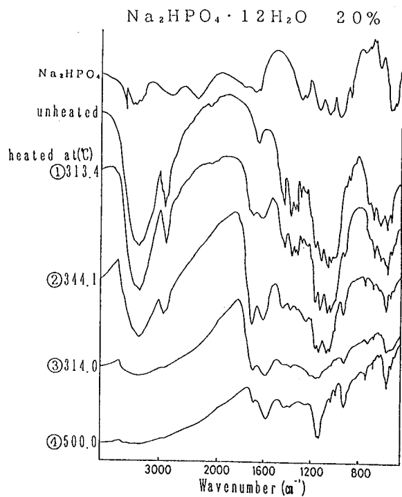
Fig. 6-23 IR spectral change in cotton fiber treated with 20% of Na 2 HPO 4 .
