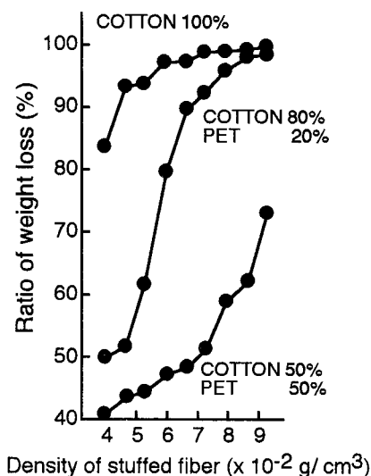
Fig. 5-8 Effect of blending polyester with cotton fiber assemblies on weight loss after smoldering combustion by burning cigarette.
