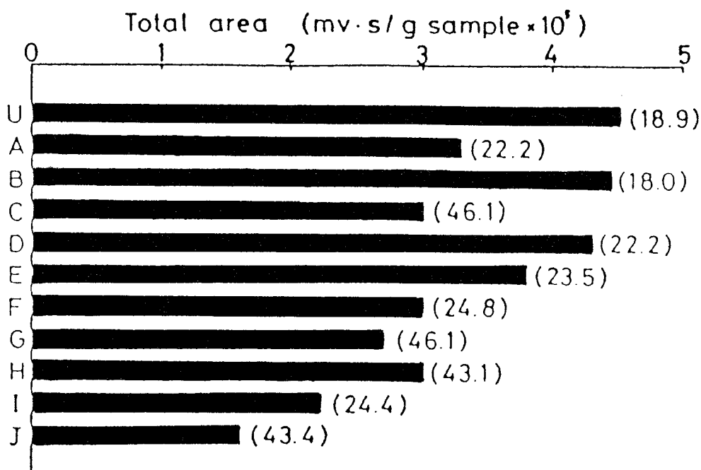
Fig. 6-50 Total amount of pyrolytic gases. (U), Untreated. Treated samples with : (A), 20% urea : (B), 20% \text{NH}_4\text{OH} : (C), 20% \text{H}_3\text{PO}_4 : (D), 20% \text{Na}_2\text{HPO}_4 : (E), 20% urea + \text{Na}_2\text{HPO}_4 : (F), 5% urea + \text{H}_3\text{PO}_4 : (G), 20% urea + \text{H}_3\text{PO}_4 : (H), 20% \text{NH}_4\text{OH} + \text{H}_3\text{PO}_4 : (I), 5% (\text{NH}_4)_2\text{HPO}_4 and (J), 20% (\text{NH}_4)_2\text{HPO}_4 .
