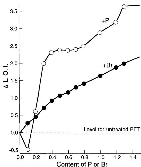
Fig. 3-29 Comparison of \Delta\text{LOI} values observed between Br-containing PET fabric and P-containing PET fabric at the same content in a range of lower contents.
