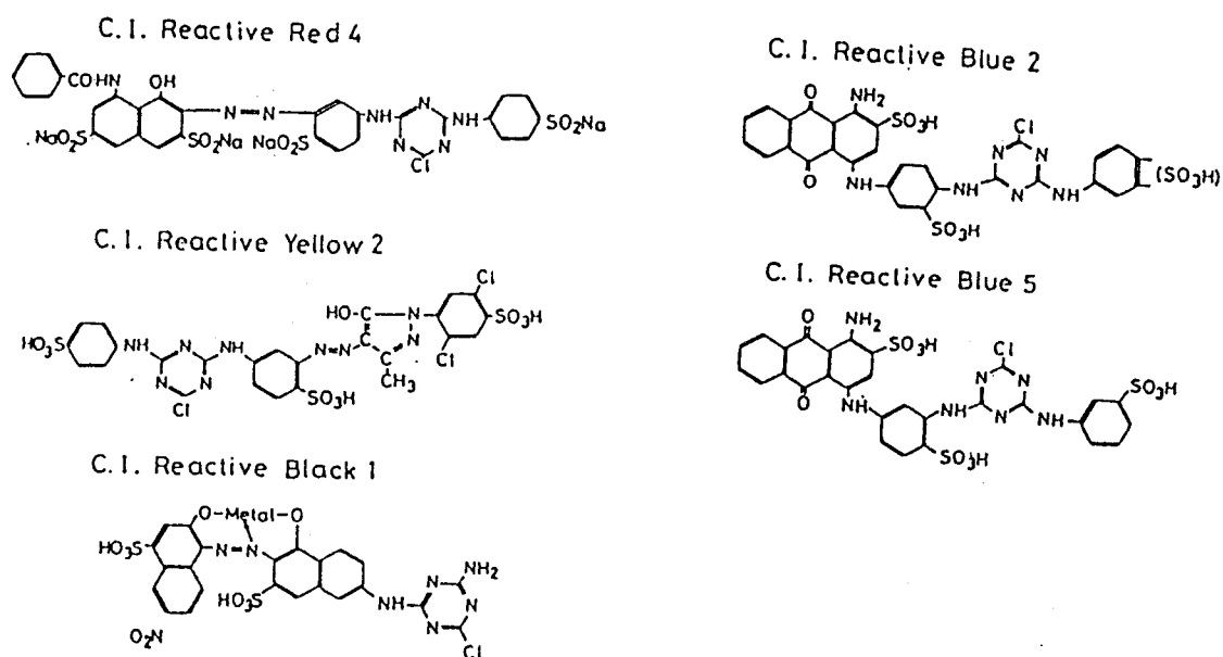
Fig. 4-1 Chemical structures of reactive dyes.
