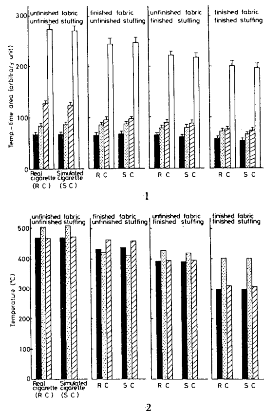
Fig. 5-19 Comparison of accumulated heats (1) and maximum temperature (2) between RC and SC observed with minature Futons. The composition of minature Futons was shown above.
