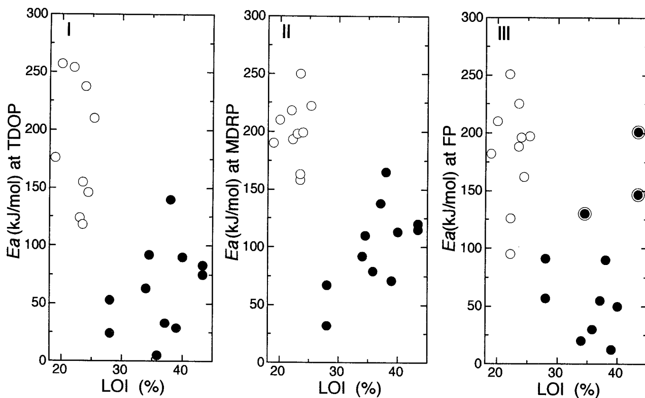
Fig. 6-13 Relationship between LOI values and E_a at TDOP, MDRP and FP. (samples with \text{LOI} \geq 28\% are indicated by solid marks and those with \text{LOI} < 28\% by open marks, \bullet indicates the samples containing N and P or Ca.
