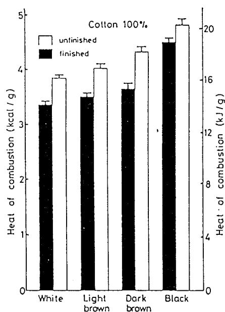
Fig. 5-26 Change in the heat of combustion of cotton fiber assemblies and fabric with progress of charring.
