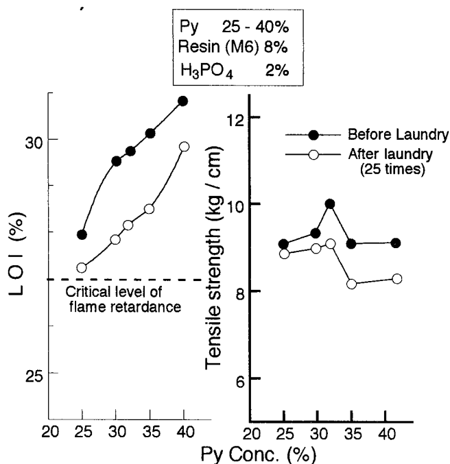
Fig. 3-1 Relationship between Pyrovatex concentrations in treating bath and LOI or tensile strength.
