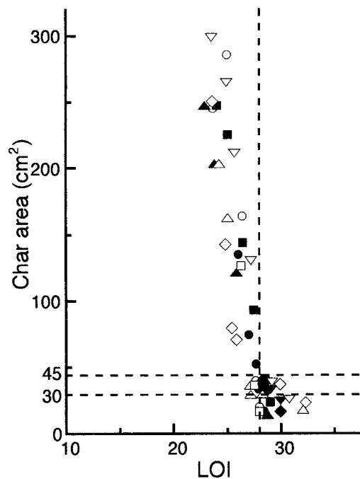
Fig. 2-3 Relation between LOI and Char area observed with flame retardant fabrics after burning.
