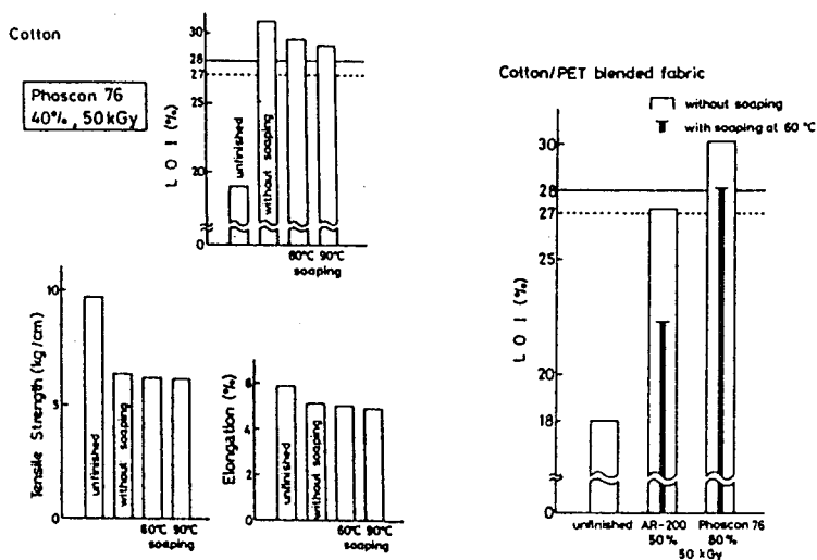
Fig. 3-51 Effect of soaping on LOI value of C/P blend treated with AR-200 in comparison with that treated with Phoscon 76.
