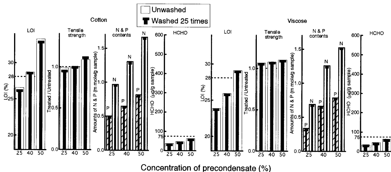
Figure 3-13 Relationship between concentration of precondensate in treating bath and LOI, tensile strength, amounts of N and P and HCHO observed for Proban finished-cotton and viscose.
