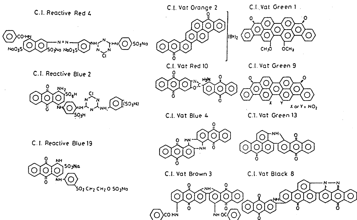
Fig. 4-4 Chemical structures of reactive dyes and vat dyes used for the present study.
