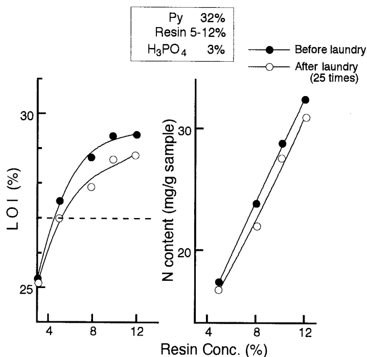
Fig. 3-4 Relationship between resin concentrations in treating bath and LOI or N content.
