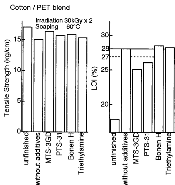
Fig. 3-57 Effect of additives on tensile strength and LOI values of C/P blend finished with Phoscon 76 (60%) and electron beam curing (conc. of each additive is 6% = 1/10 \times 60%).
