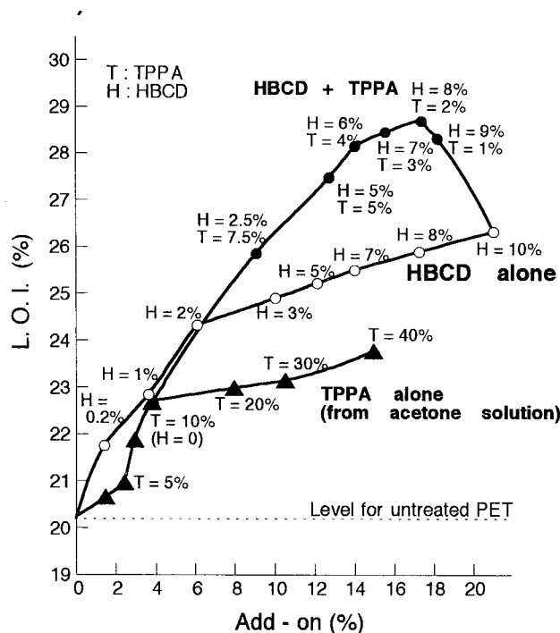
Fig. 3-28 LOI values vs add-ons of PET fabric treated with acetone solutions of HBCD and TPPA each alone as well as of combination of both elements.
