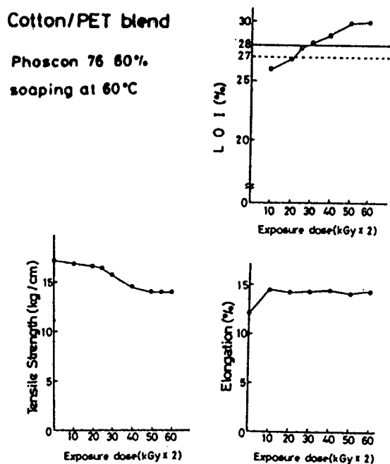
Fig. 3-56 Effect of exposure dose of electron beam (on both side) on LOI value, tensile strength and elongation.
