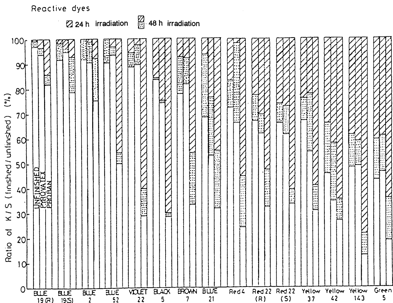
Fig. 4-7 Effect of ultraviolet irradiation on reactive dyes observed with and without flame retardant finish, Pyrovatex finish or Proban finish.
