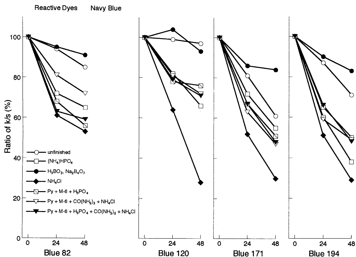
Fig. 4-19 Effect of ultraviolet irradiation on reactive dyes having bisazoic chromogen and different functional groups and inhibiting effect of \text{H}_3\text{BO}_3 + \text{Na}_2\text{B}_4\text{O}_7 observed by ratios (%) of K/S values obtained after irradiation to those obtained before irradiation.
