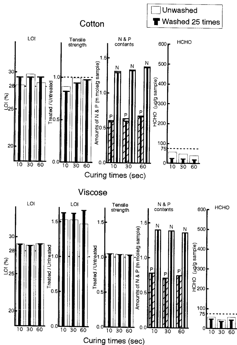
Fig. 3-16 Effects of curing time in the order of sec on LOI values, tensile strength, HCHO liberation and amounts of N and P contents on THPS-treated cotton and viscose fabrics.
