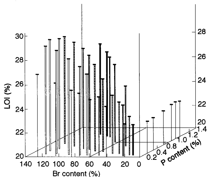
Fig. 3-33 Synergistic effect of Br and P illustrated by a three dimensional diagram.
