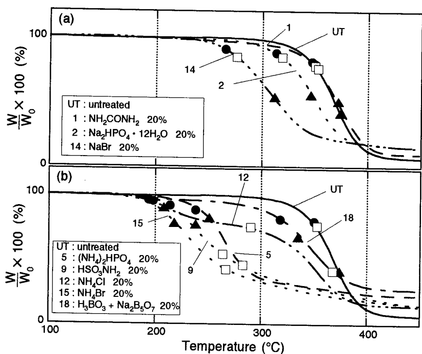
Fig. 6-5 Mutual relationship among TDOP (solid circle), MDRP (solid triangle) and FP (open square) on TG curves and difference in mutual position observed between the flame retardant samples (b) and the samples without flame retardance (a).
