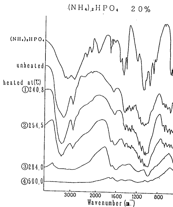
Fig. 6-24 IR spectral change in cotton fiber treated with 20% of (NH 4 ) 2 HPO 4 .
