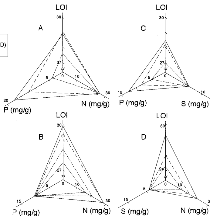
Fig. 3-10 Relationship of LOI to N, P and S contents.
