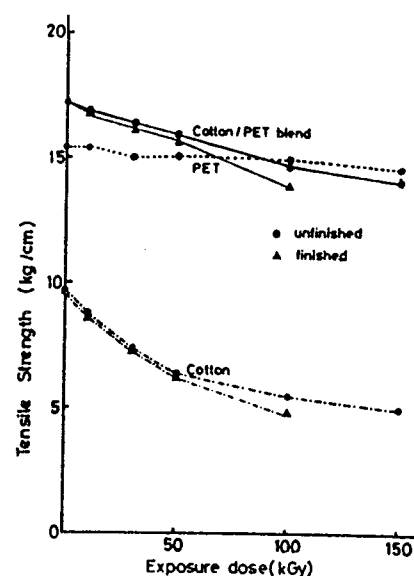
Fig. 3-54 Change in tensile strength with exposure dose of electron beam observed for Cotton, PET and C/P blended fabrics.
