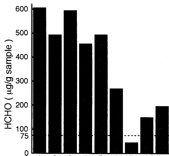
Fig. 3-12 Comparison of HCHO contents observed after oxidizing and soaping under various conditions shown in Table 3-2.
