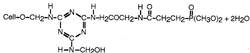
Figure 3-20 Cross linking actions of resins between cellulose and flame retardants.
