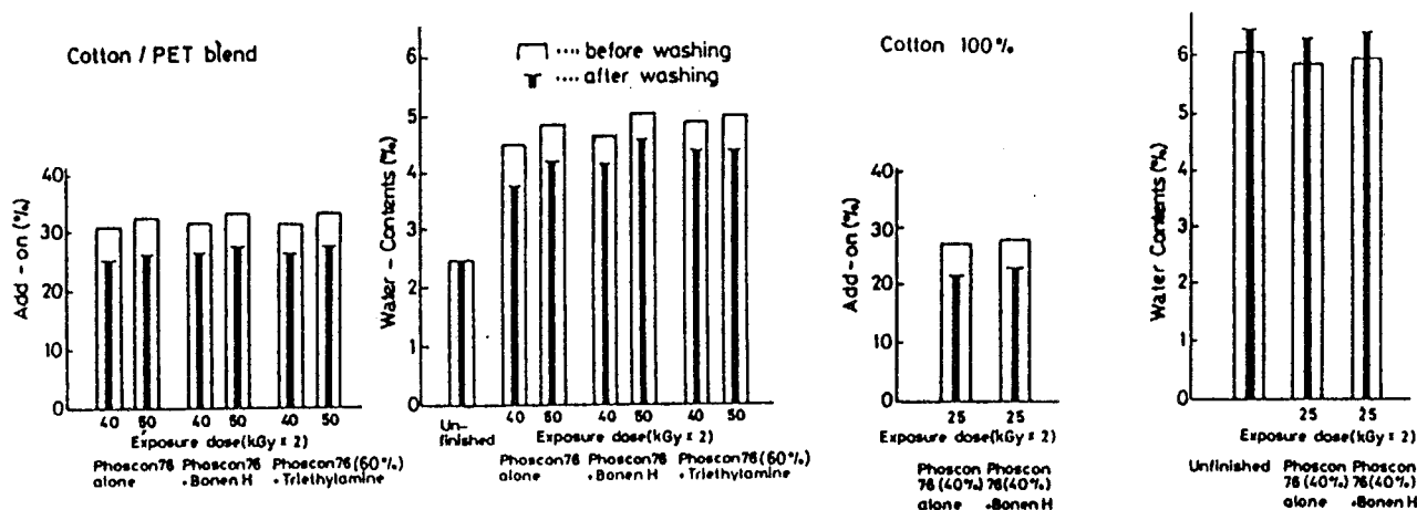
Fig. 3-59 Add-ons and water contents of C/P blended cotton 100% fabrics finished with Phoscon 76 with and without Bonen H (6%).
